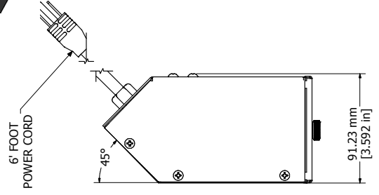
ASSEMBLY VIEW FROM SIDE
