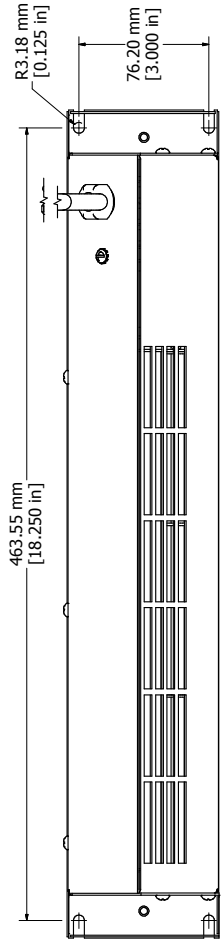
ASSEMBLY - VIEW FROM BACK
