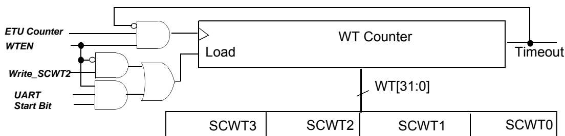
Figure 33. Waiting Time Counter
