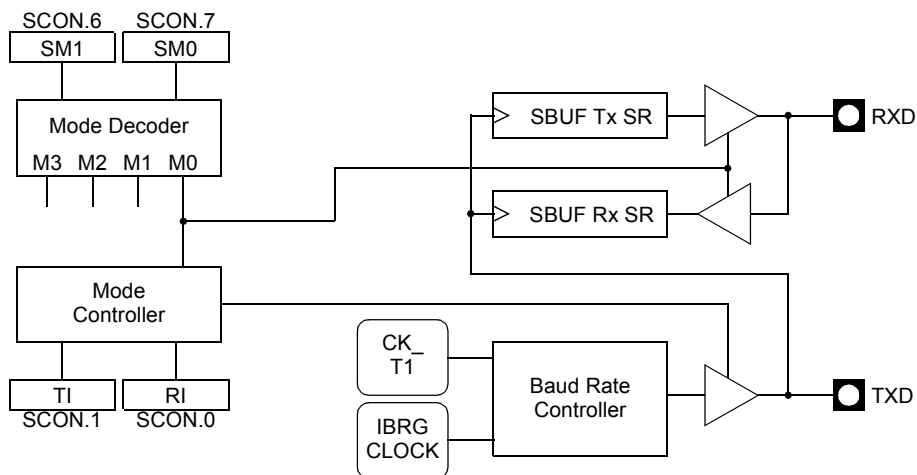
Figure 69. Serial I/O Port Block Diagram (Mode 0)
