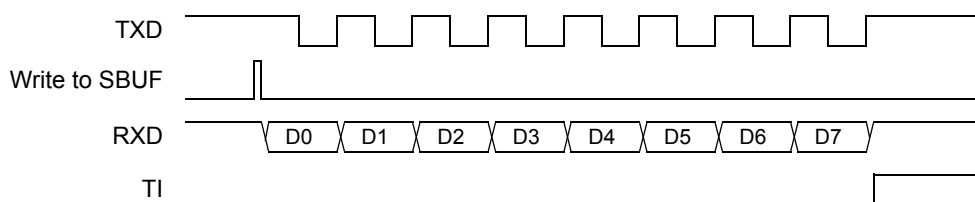
Figure 70. Transmission Waveforms (Mode 0)
