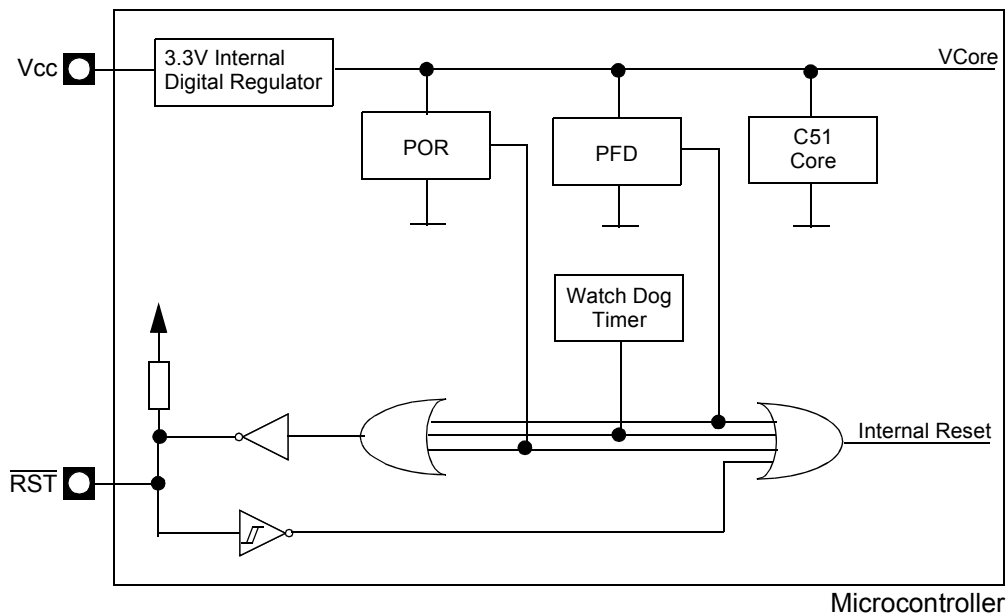
Figure 100. Reset block diagram
