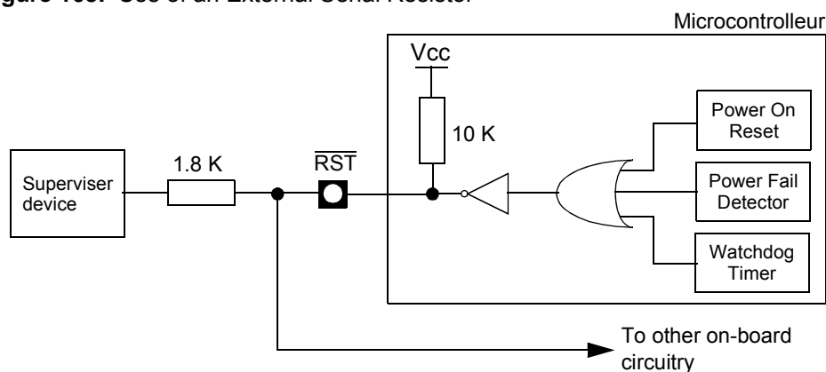
Figure 105. Use of an External Serial Resistor
