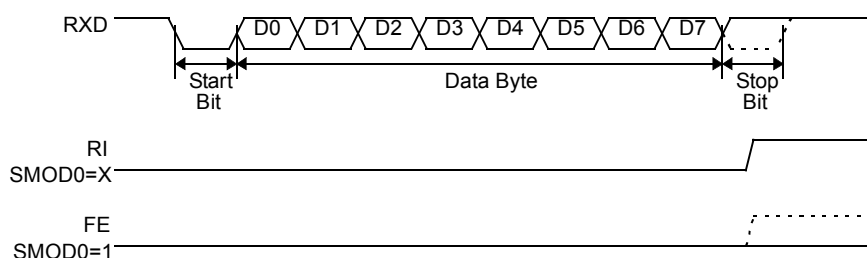
Figure 65. UART Timings in Mode 1
