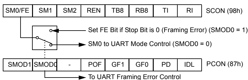
Figure 64. Framing Error Block Diagram
