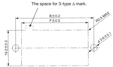
Panel Cutout
