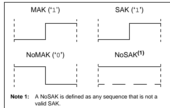
FIGURE 5-3: ACKNOWLEDGE BITS
