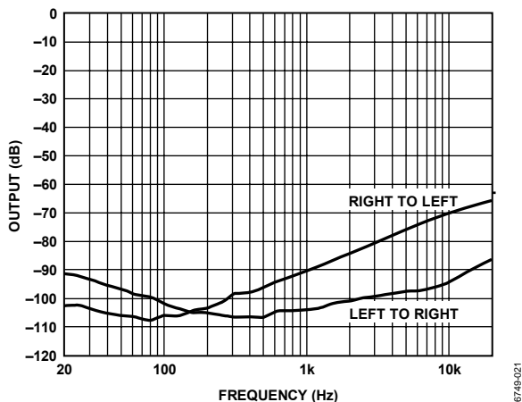
Figure 21. Crosstalk @ 1 W, 6 Ω, PVDD = 15 V, PGA = 0 dB
