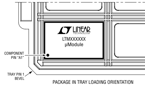
PACKAGE IN TRAY LOADING ORIENTATION
