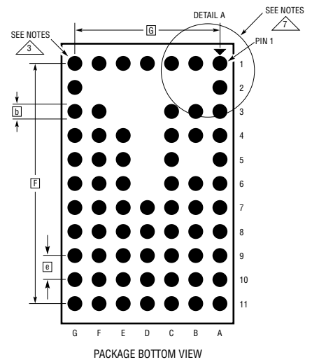
PACKAGE BOTTOM VIEW
