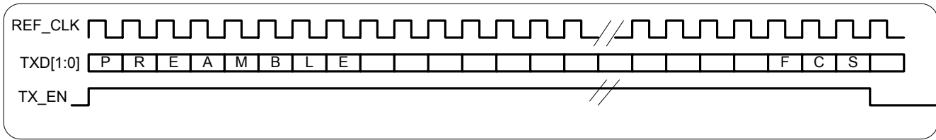
Figure 11-23. RMII Transmit Interface Functional Timing
