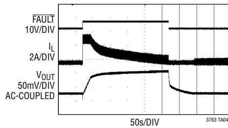
36V SLA Battery Charging
