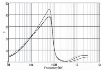
— LQB15NNR22M10 220nH ····· LQB15NNR56M10 560nH
