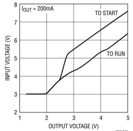
Minimum Required Input Voltage vs Output Voltage (I OUT = 200mA)
