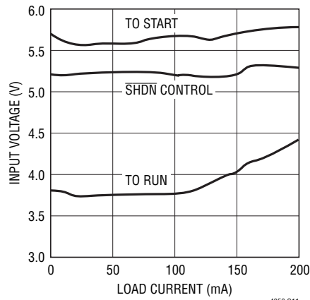
Minimum Required Input Voltage vs Load (V OUT = 3.3V)
