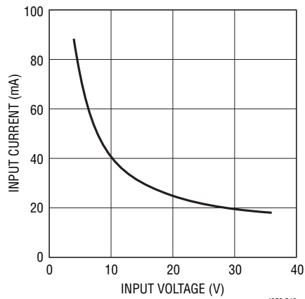
Input Current vs Input Voltage (Output Short)
