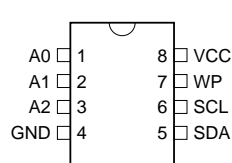
8-lead PDIP
