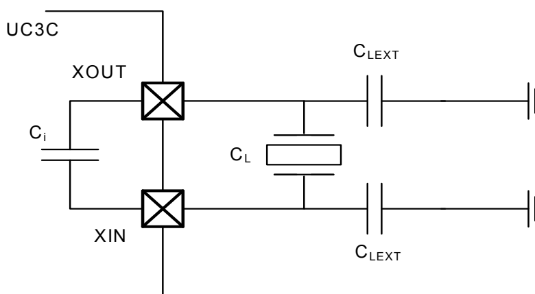
Figure 8-1. Oscillator connections
