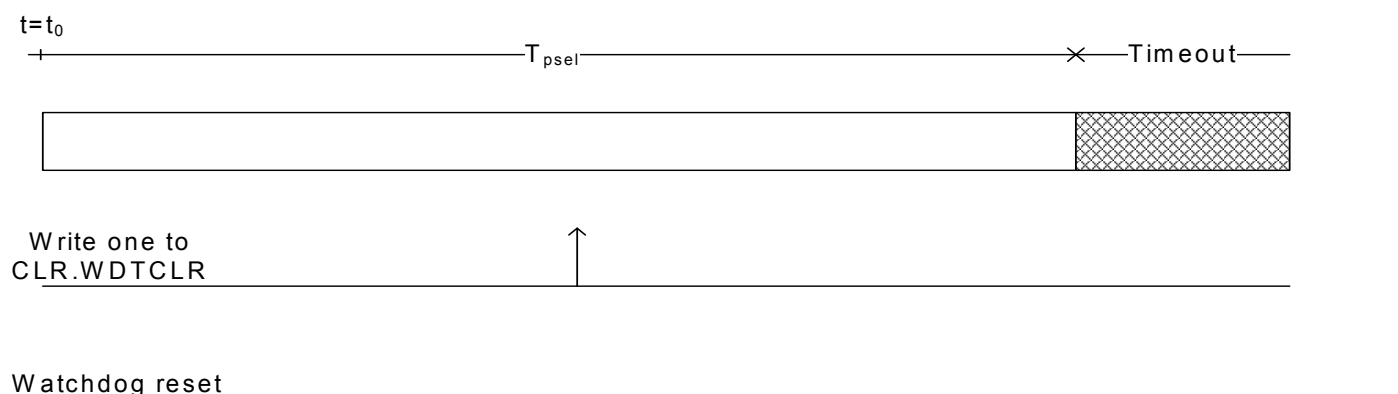
Figure 10-2. Basic Mode WDT Timing Diagram, normal operation.
