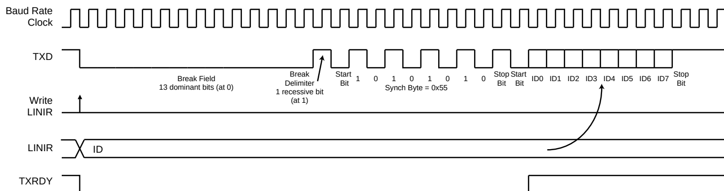
Figure 25-39. Header Transmission
