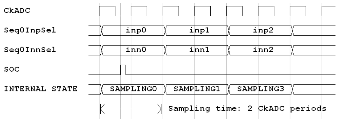
Figure 36-8. Oversampling
