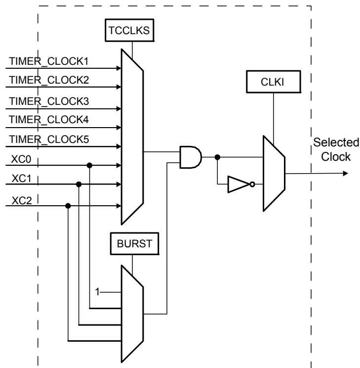
Figure 23-2. Clock Selection
