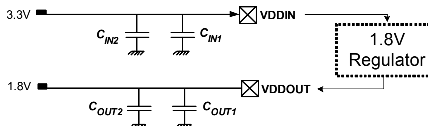
Figure 5-2. Supply Decoupling
