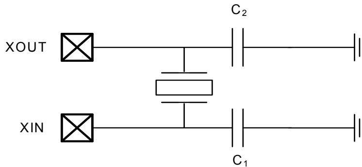
Figure 9-2. Oscillator connections
