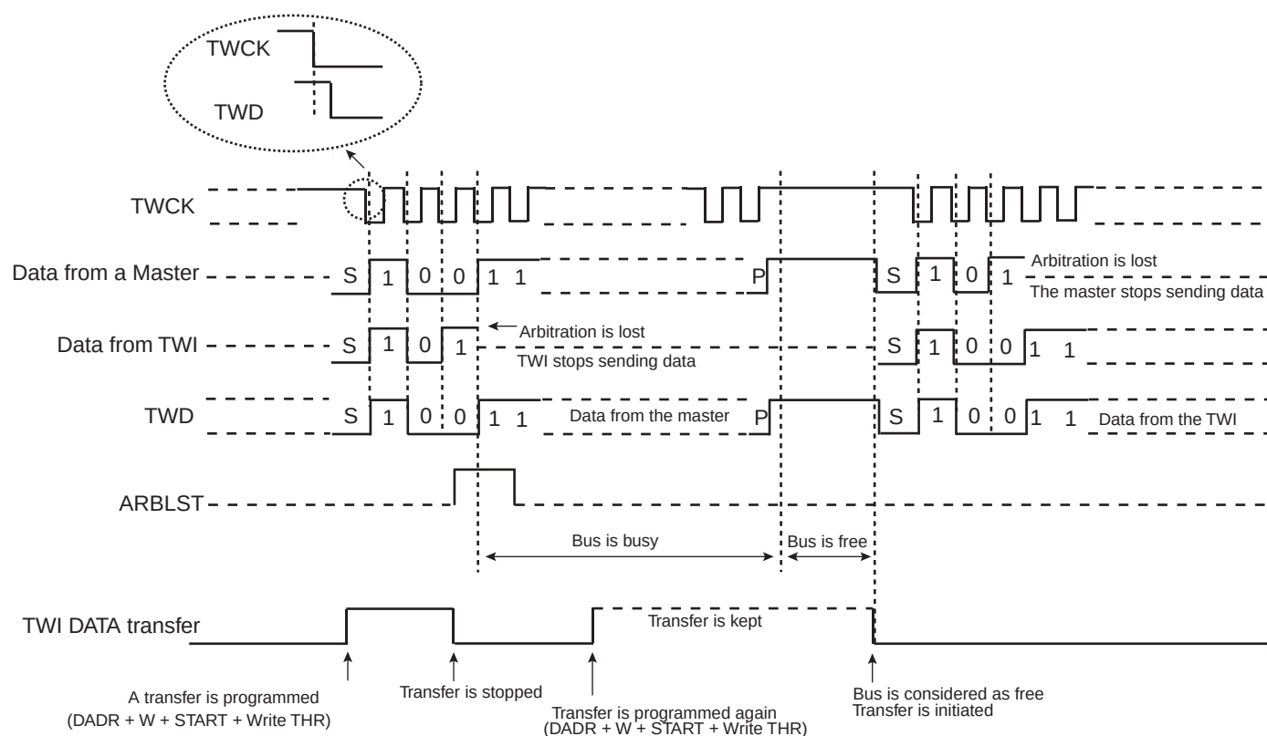
Figure 19-21. Arbitration Cases
