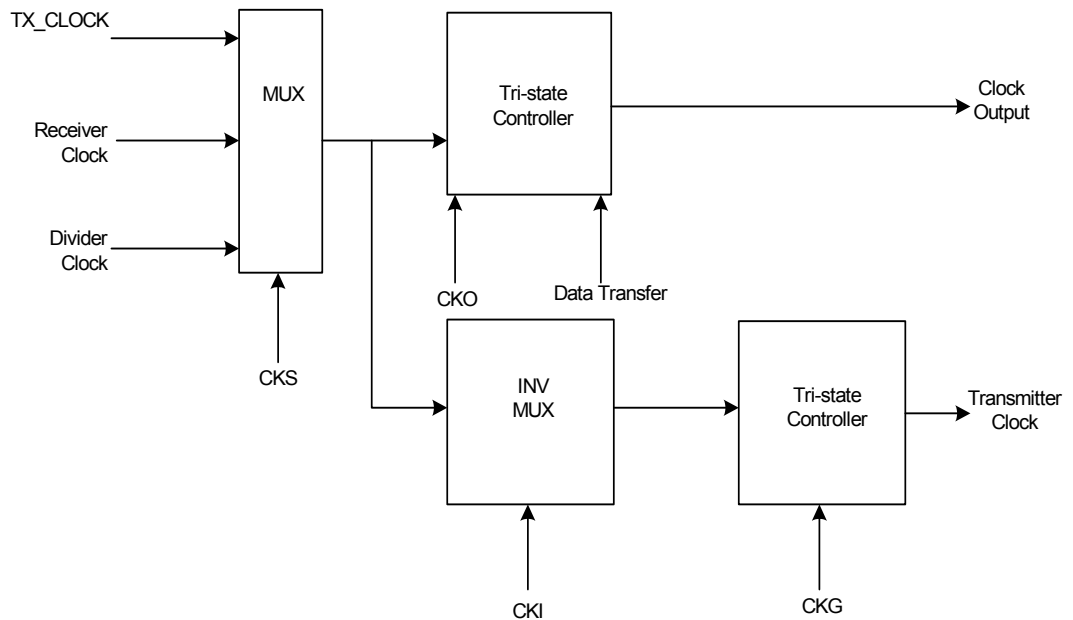
Figure 20-6. Transmitter Clock Management
