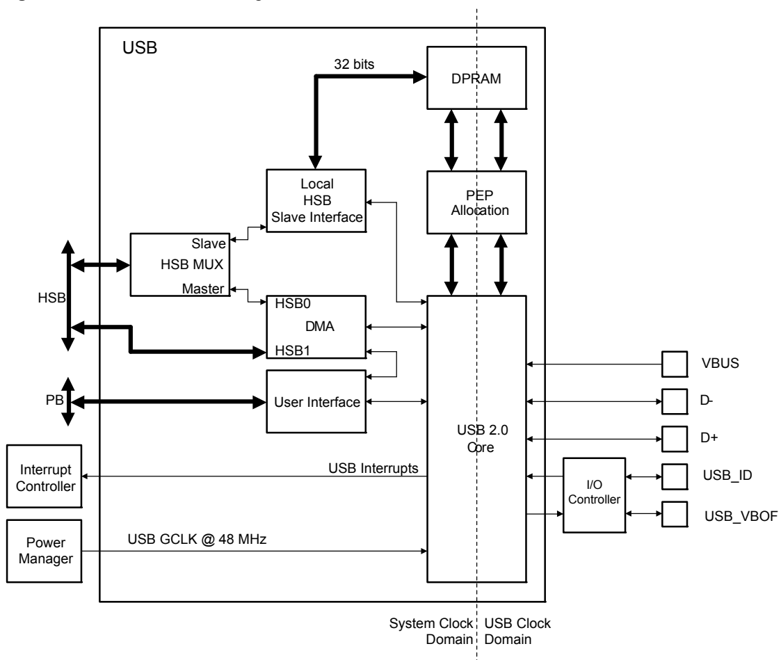
Figure 22-1. USBB Block Diagram
