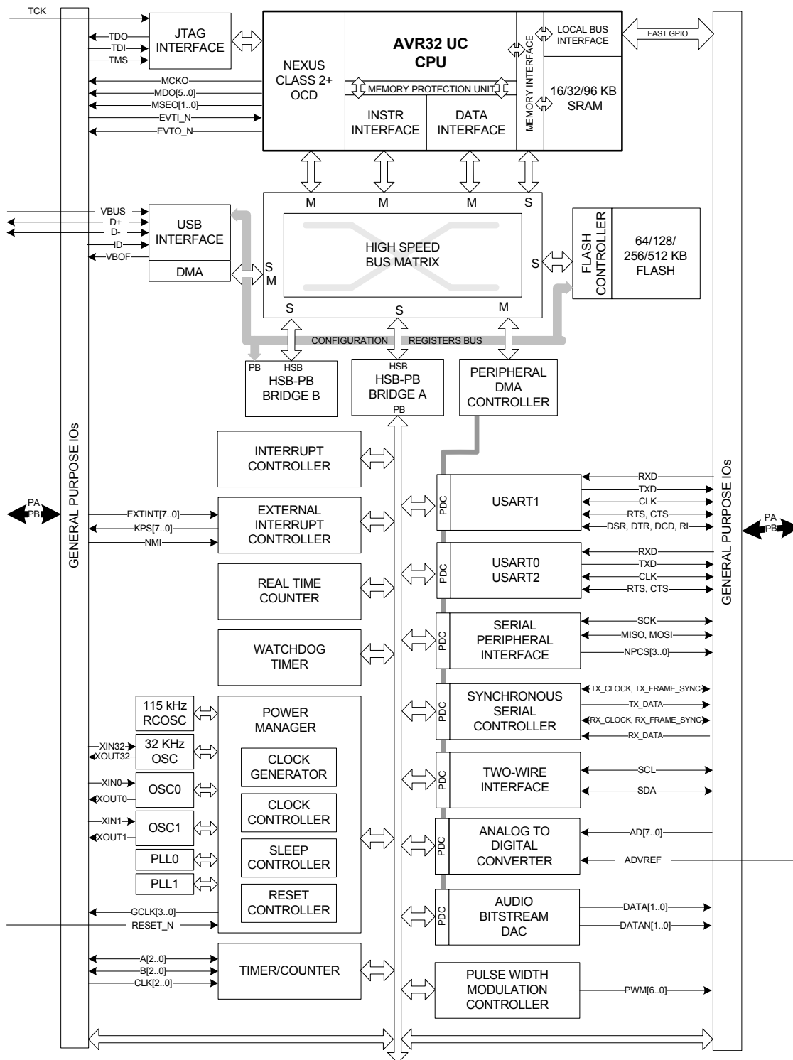
Figure 2-1. Block diagram
