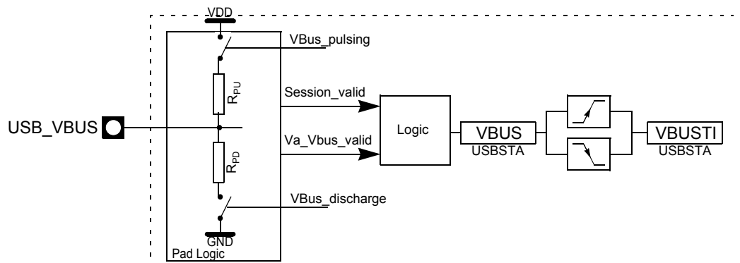
Figure 22-11. Plug-In Detection Input Block Diagram
