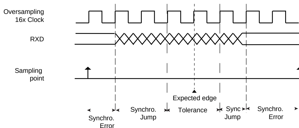
Figure 21-10. Bit Resynchronization
