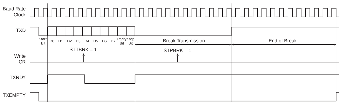
Figure 21-25. Break Transmission
