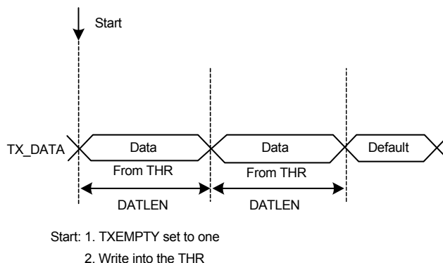
Figure 20-14. Transmit Frame Format in Continuous Mode
