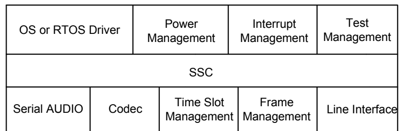
Figure 20-2. SSC Application Block Diagram
