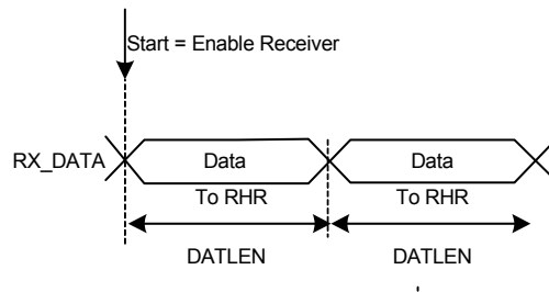
Figure 20-15. Receive Frame Format in Continuous Mode
