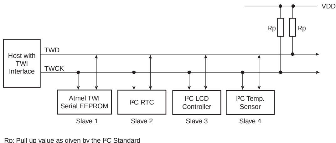
Figure 19-2. Application Block Diagram
