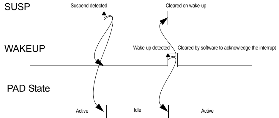
Figure 22-10. Pad Events
