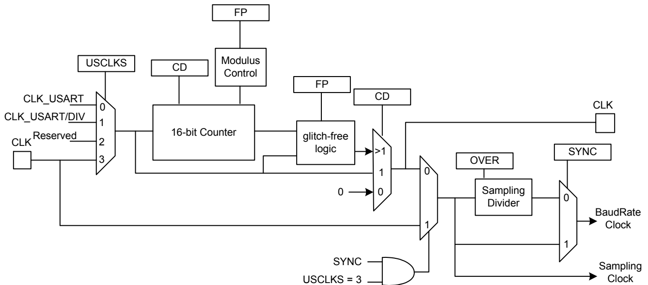
Figure 21-3. Fractional Baud Rate Generator
