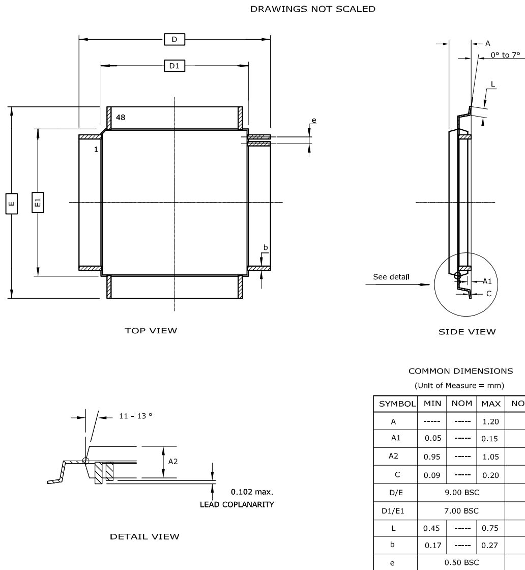
Figure 29-2. TQFP-48 package drawing
