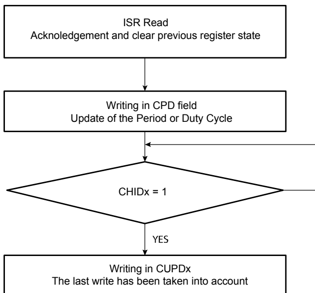
Figure 24-7. Polling Method
