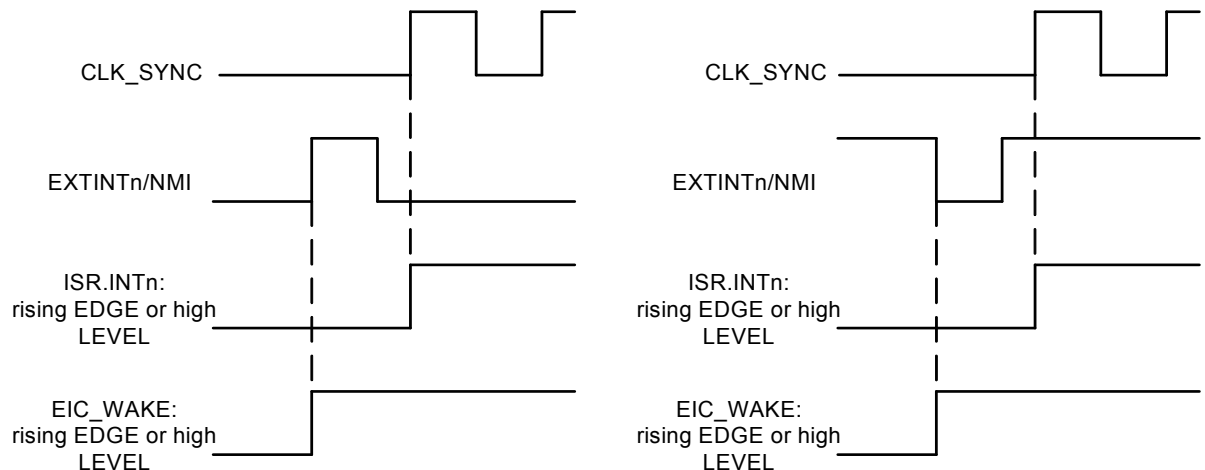
Figure 13-4. Timing Diagram, Asynchronous Interrupts
