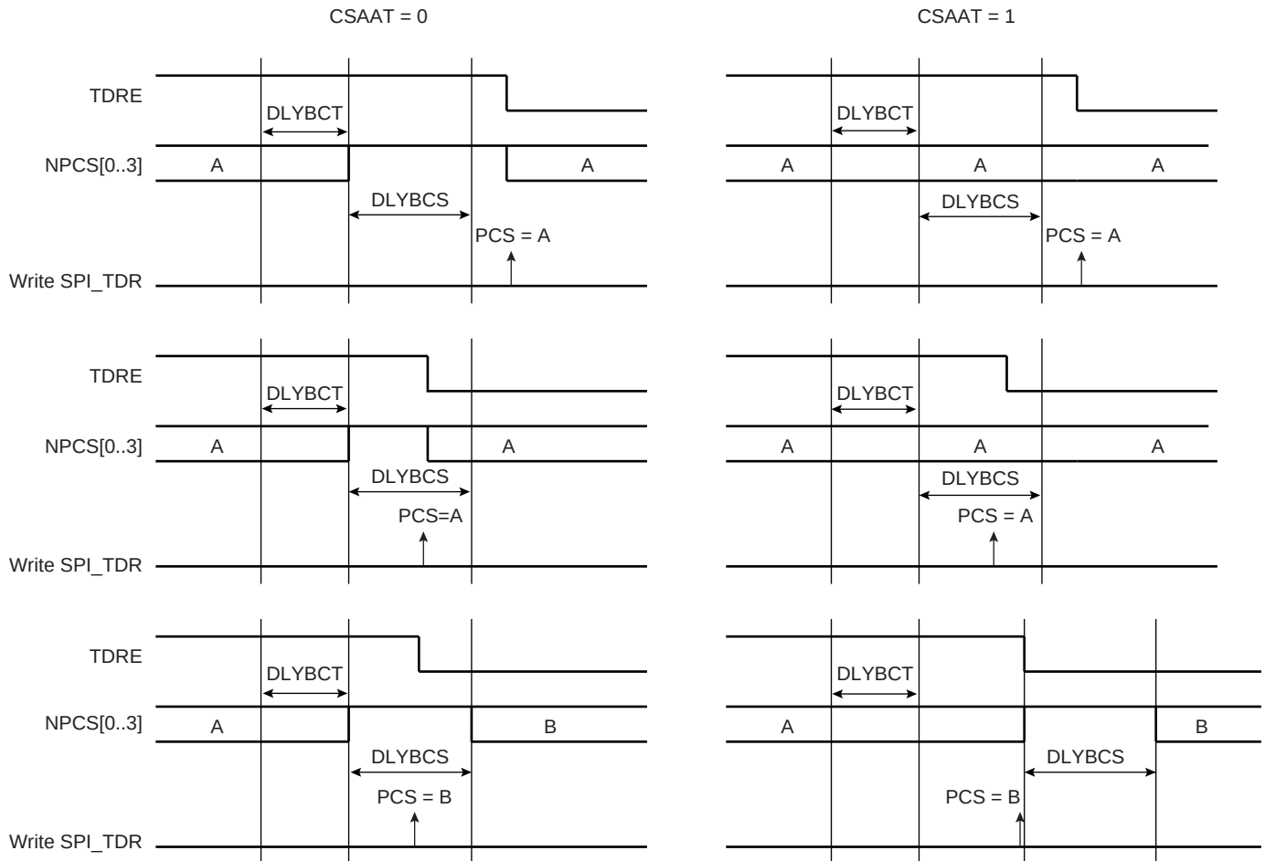
Figure 18-8. Peripheral Deselection
