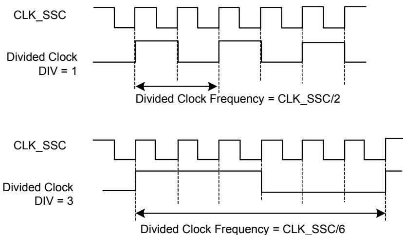
Figure 20-5. Divided Clock Generation
