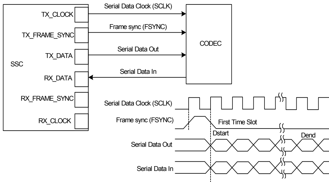
Figure 20-18. Codec Application Block Diagram
