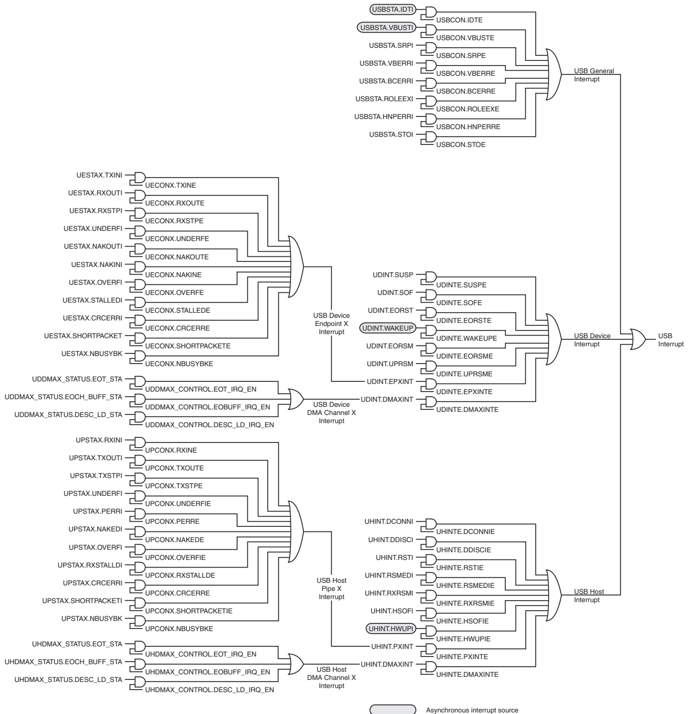
Figure 22-6. Interrupt System
