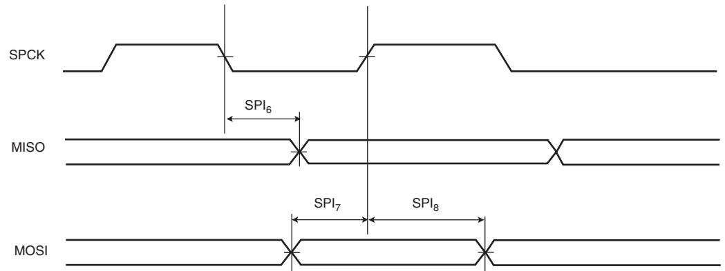
Figure 38-8. SPI Slave mode with (CPOL=0 and NCPHA=1) or (CPOL=1 and NCPHA=0)
