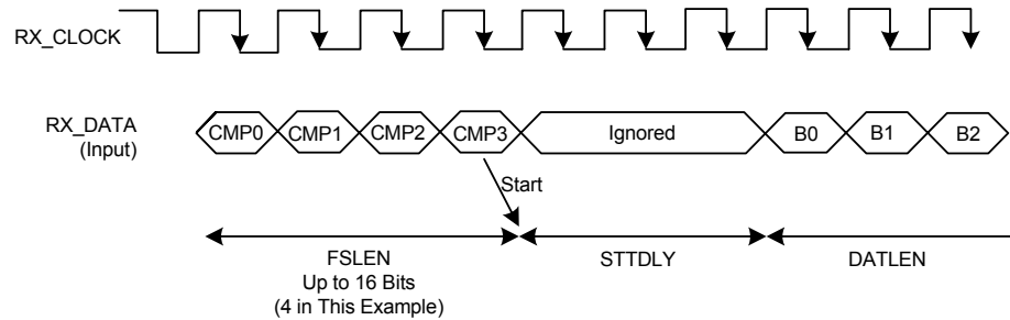
Figure 25-12. Receive Compare Modes
