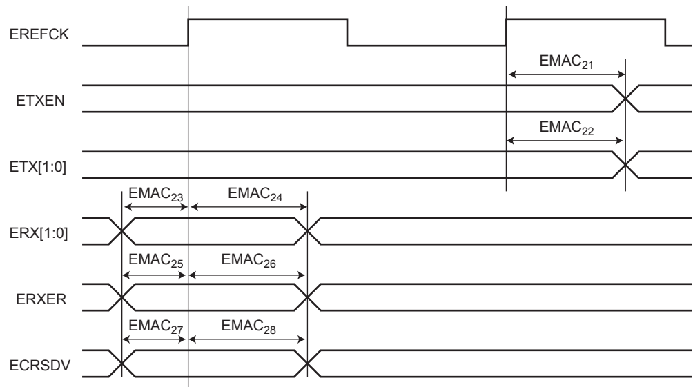
Figure 38-11. Ethernet MAC RMII Mode
