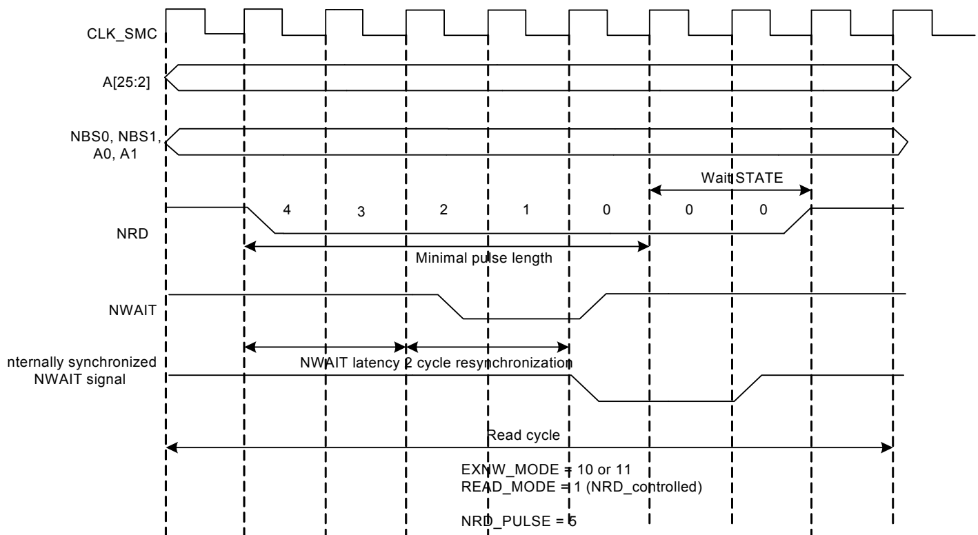
Figure 27-31. NWAIT Latency
