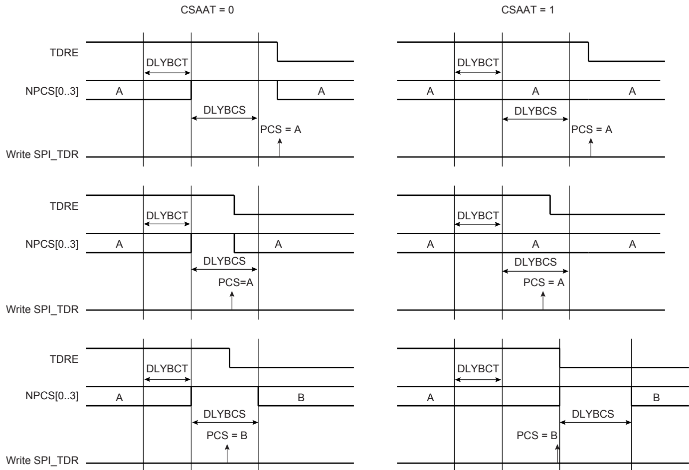
Figure 23-8. Peripheral Deselection
