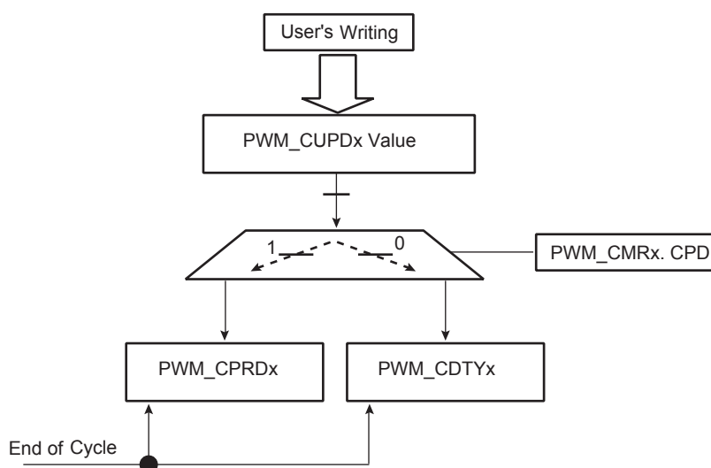
Figure 32-6. Synchronized Period or Duty Cycle Update
