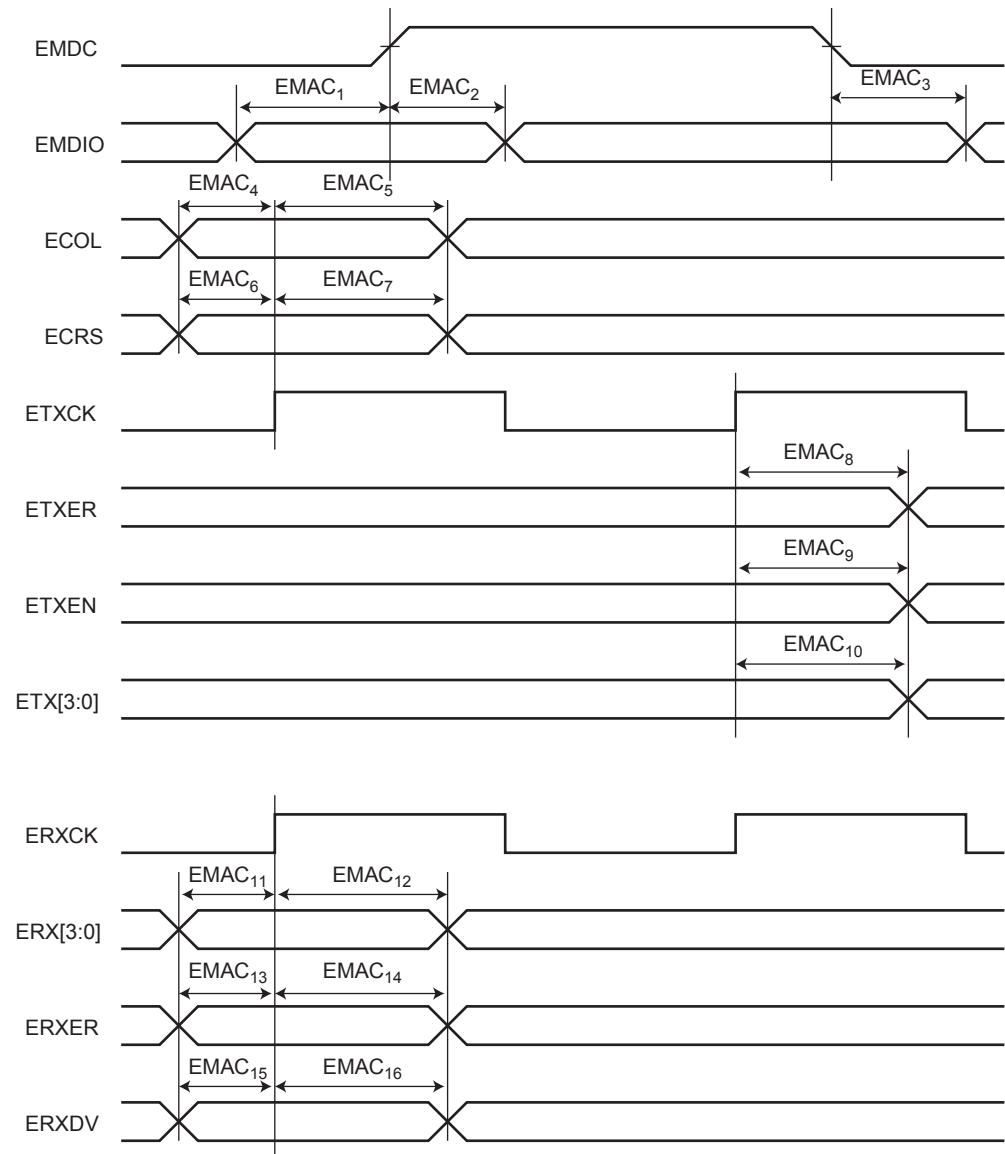
Figure 38-10. Ethernet MAC MII Mode
