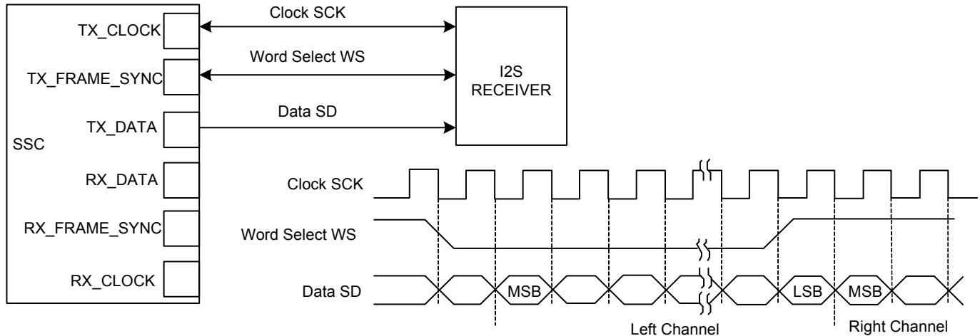
Figure 25-17. Audio Application Block Diagram
