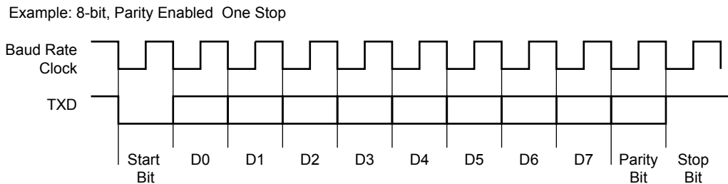
Figure 26-6. Character Transmit
