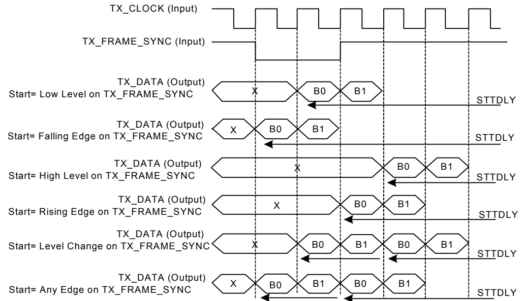
Figure 25-10. Transmit Start Mode
