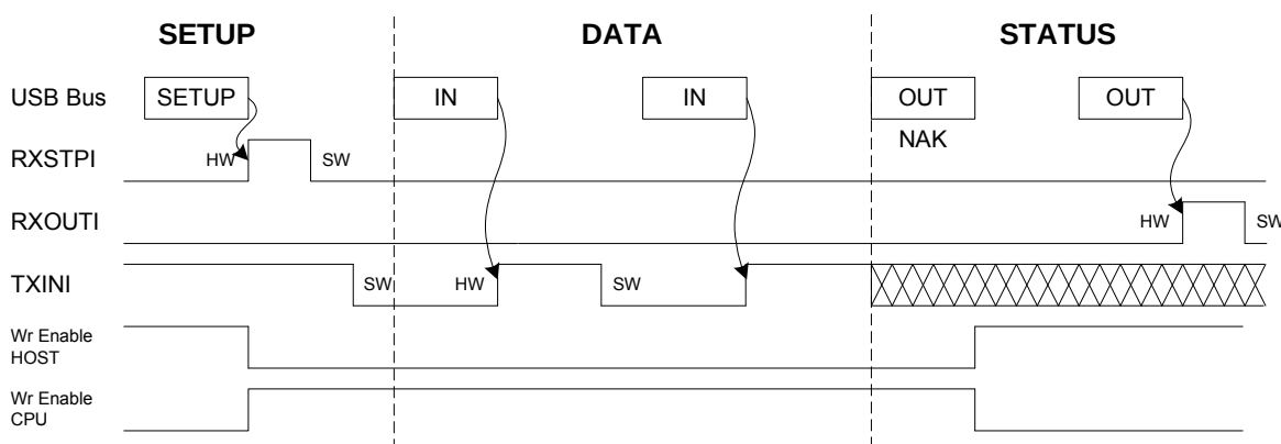
Figure 30-16. Control Read
