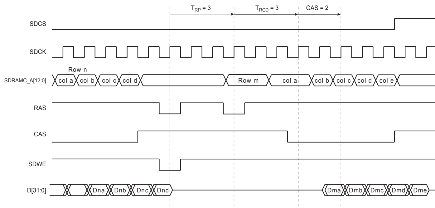
Figure 28-7. Read Burst with Boundary Row Access
