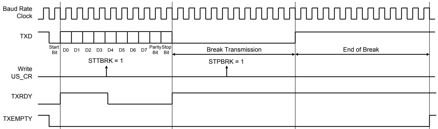
Figure 26-26. Break Transmission
