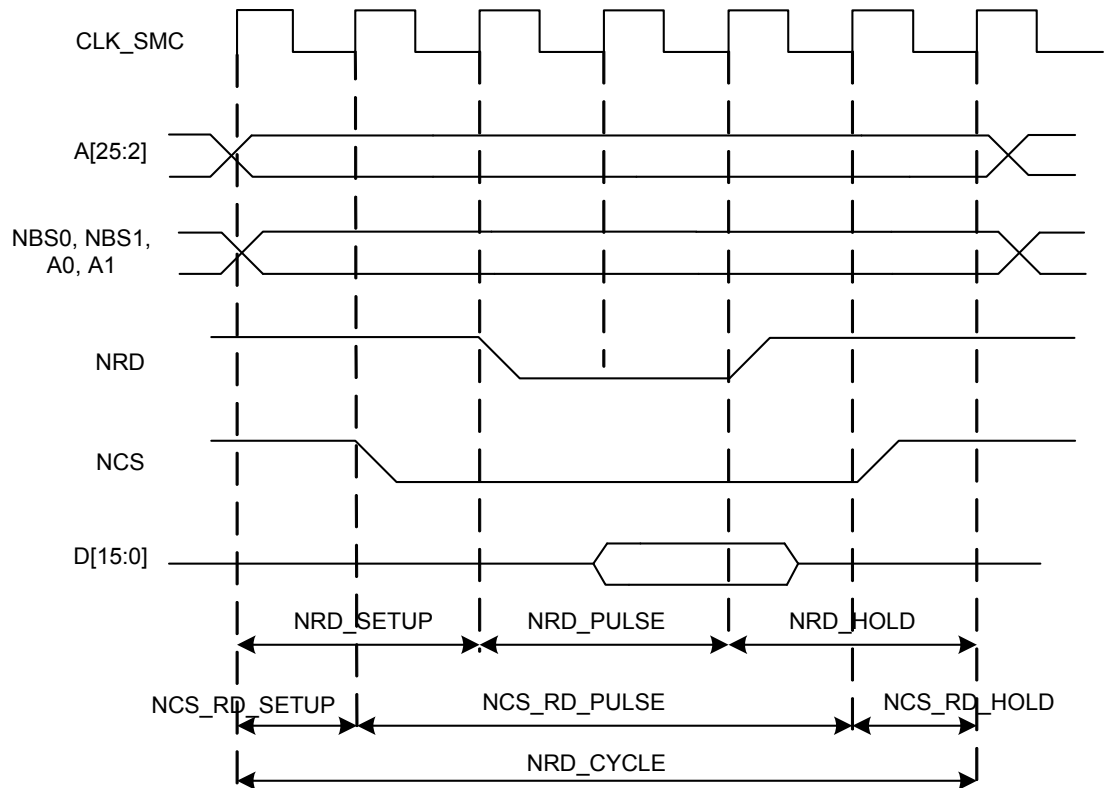
Figure 27-9. Standard Read Cycle
