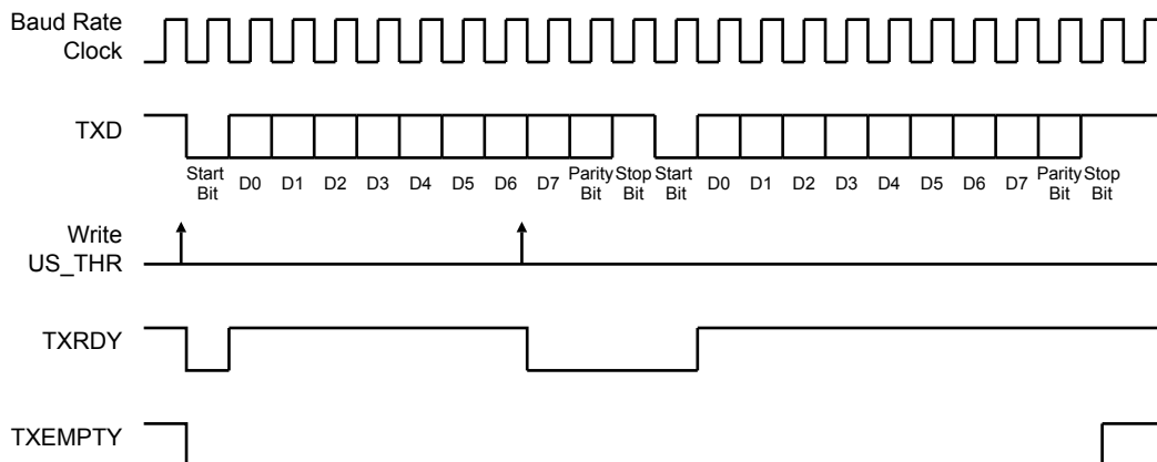
Figure 26-7. Transmitter Status
