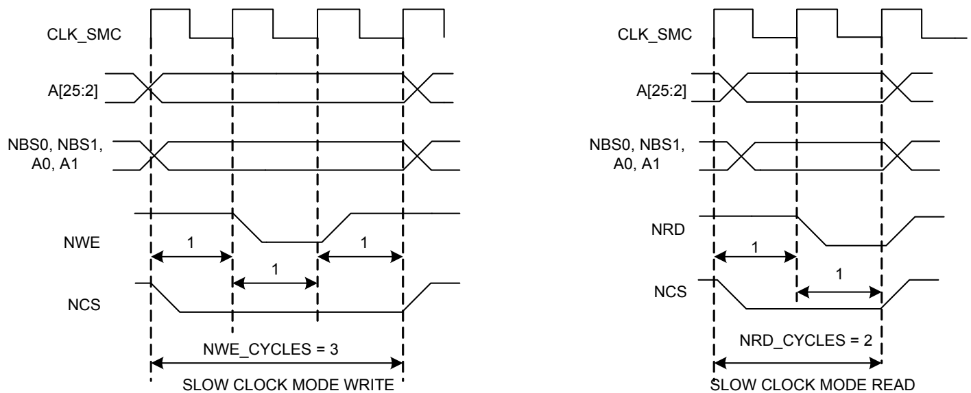
Figure 27-32. Read/write Cycles in Slow Clock Mode
