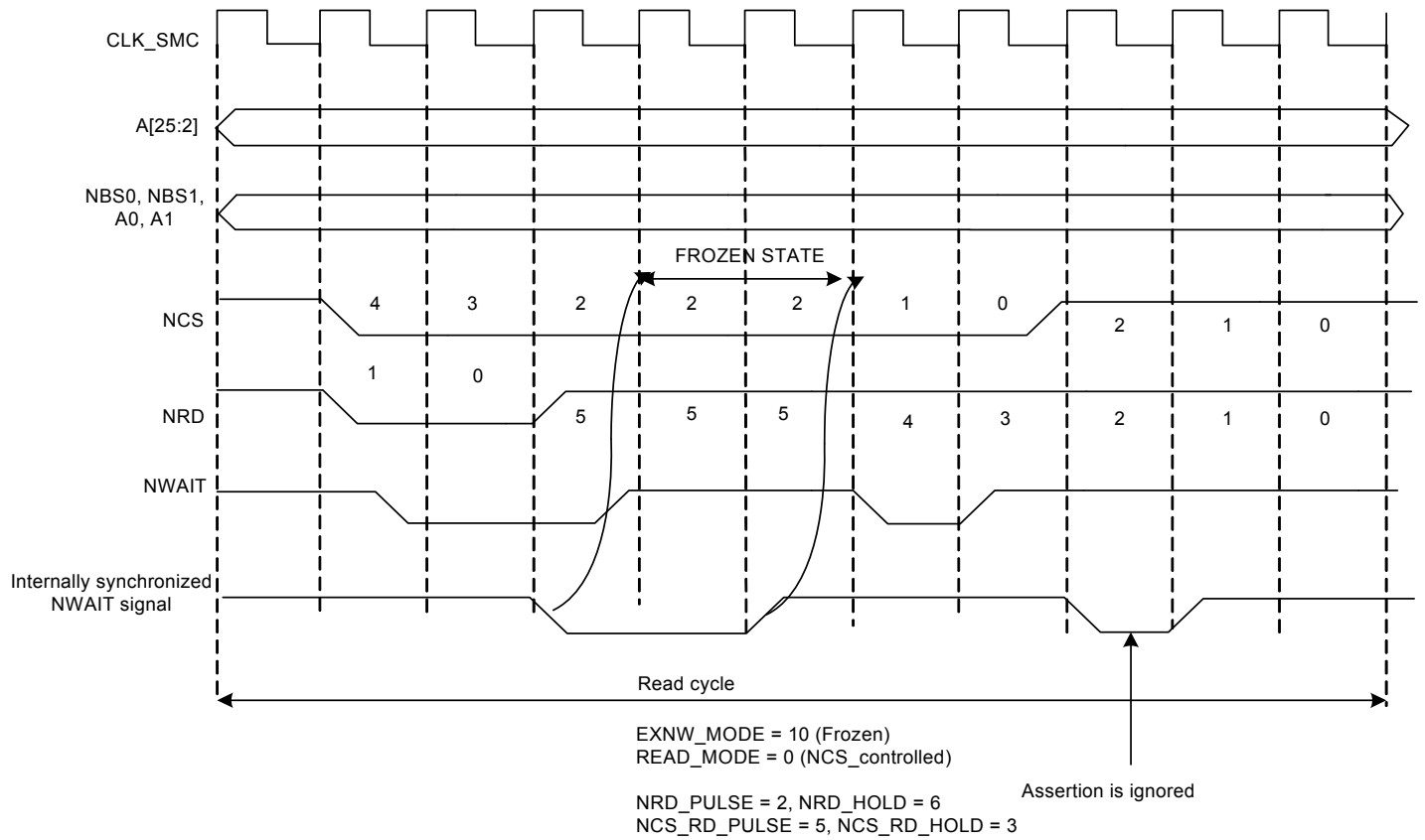
Figure 27-28. Read Access with NWAIT Assertion in Frozen Mode (EXNW_MODE = 10).
