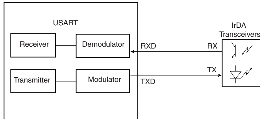
Figure 26-33. Connection to IrDA Transceivers
