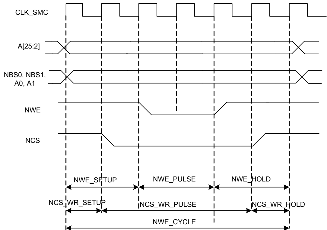
Figure 27-13. Write Cycle
