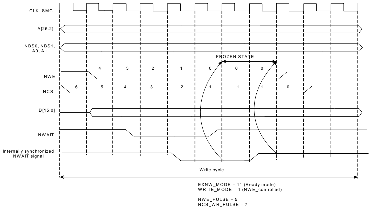
Figure 27-29. NWAIT Assertion in Write Access: Ready Mode (EXNW_MODE = 11).
