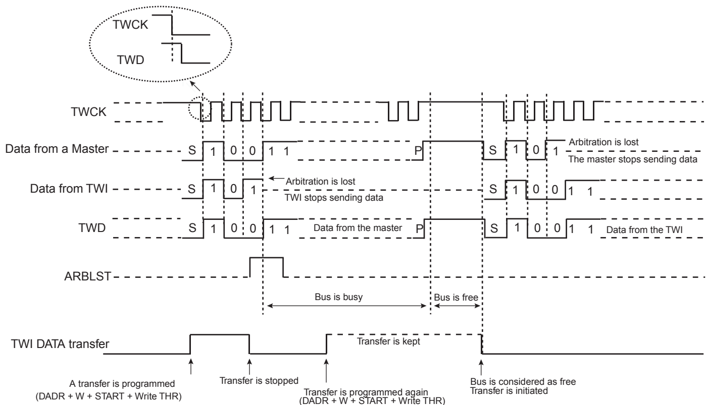
Figure 24-20. Arbitration Cases
