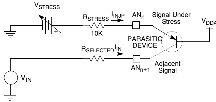
Figure 14-53. Input Signal Subjected to Positive Stress
