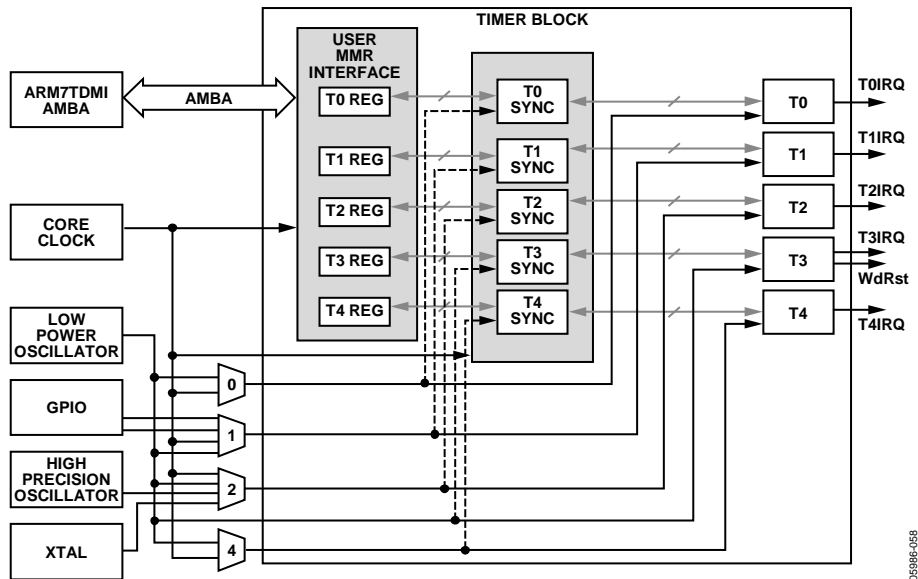
Figure 30. Timer Block Diagram
