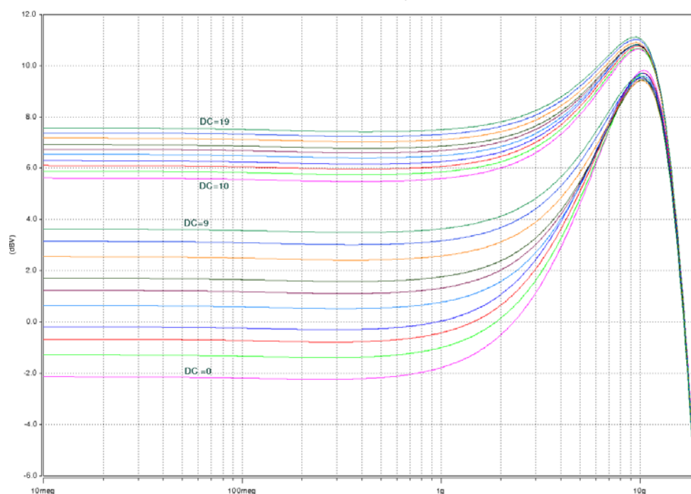
Figure 6. DC Gain Curves for GT Channels
