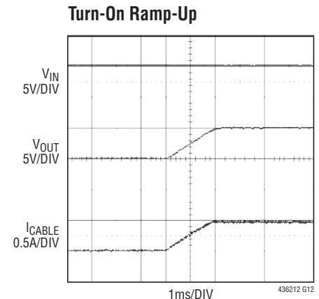
FIGURE 4 CIRCUIT R_{\text{IN}} = 150\text{m}\Omega , L_{\text{IN}} = 0.7\mu\text{H} \text{LOAD} = 10\Omega , C_{\text{OUT}} = 10\mu\text{F}
