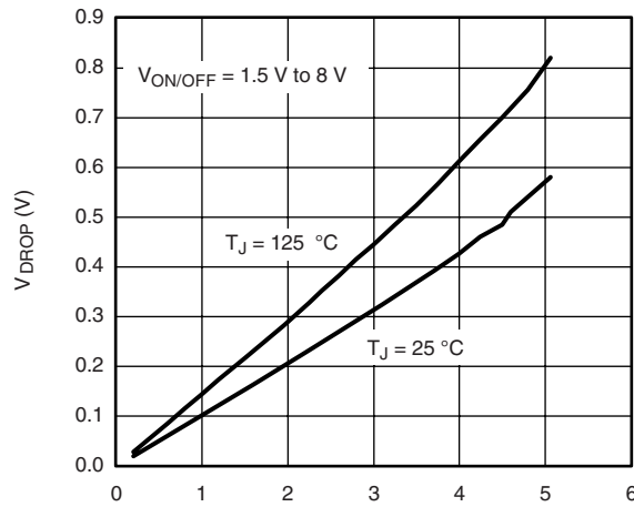
V_{DROP} vs. I_L at V_{IN} = 5 \text{ V}
