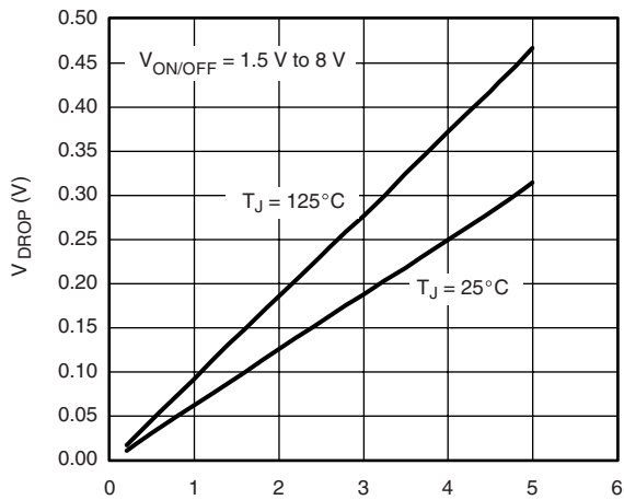
V_{DROP} vs. I_L at V_{IN} = 10 \text{ V}
