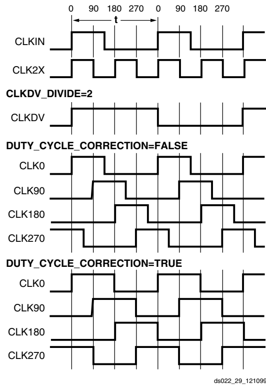
ds022_29_121099 Figure 25: DLL Output Characteristics
