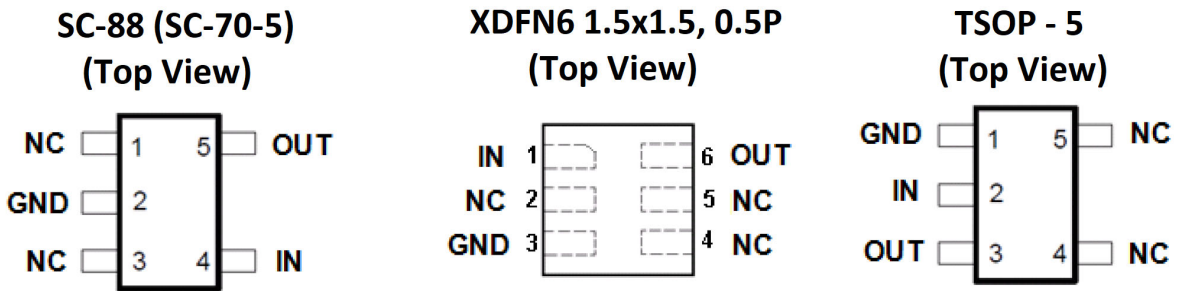
Figure 3. Pin Description
