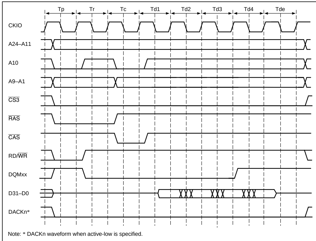
Figure 7.26 (a) Burst Read Timing (Bank Active, Different Row Addresses) Except t_{E_{cyc}} : t_{p_{cyc}} 1:1
