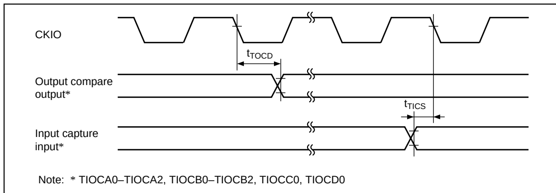
Figure 21.57 TPU Input/Output Timing (Except t_{E_{cyc}}:t_{P_{cyc}} 1:1 )
