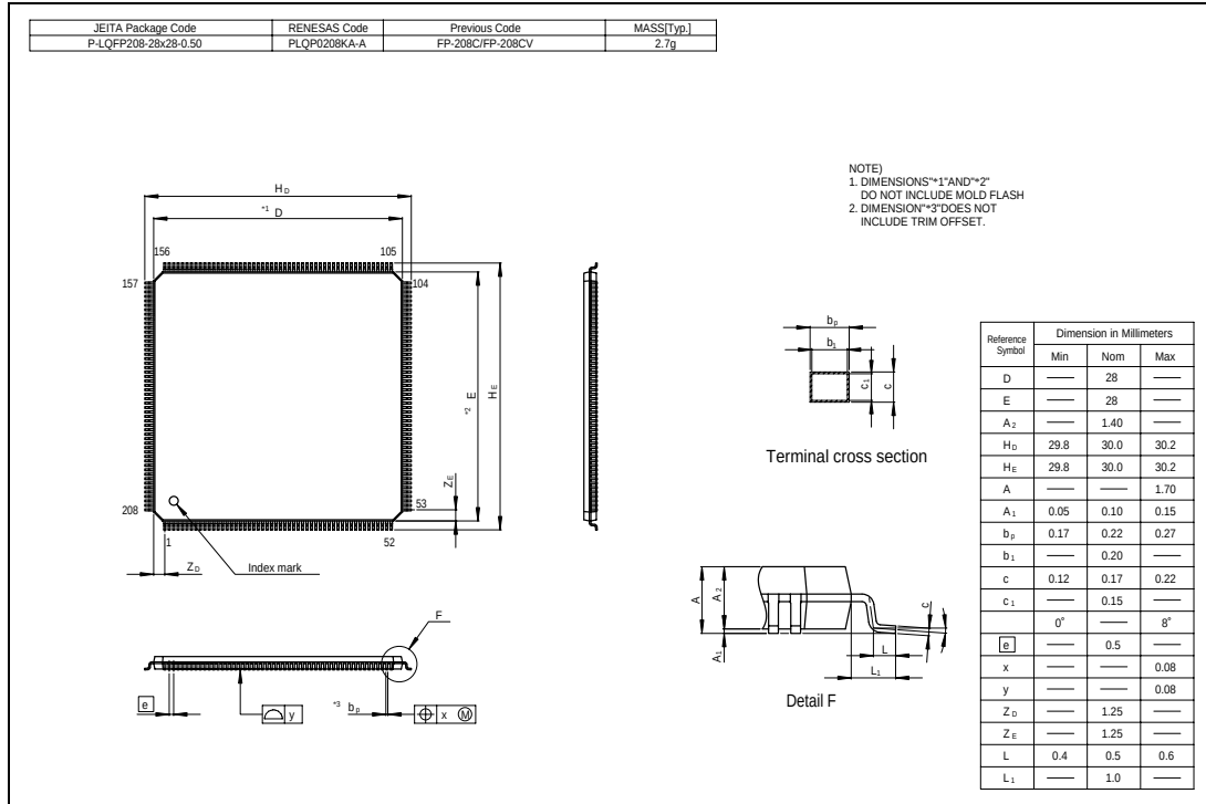
Figure D.1 Package Dimensions (FP-208C, FP-208CV)
