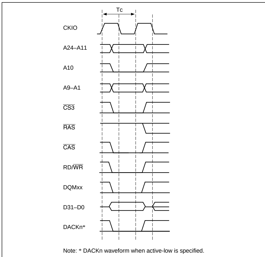
Figure 7.28 Single Write Mode Timing (Bank Active, Same Row Address)
