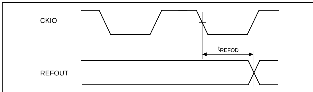
Figure 21.47 REFOUT Delay Time
