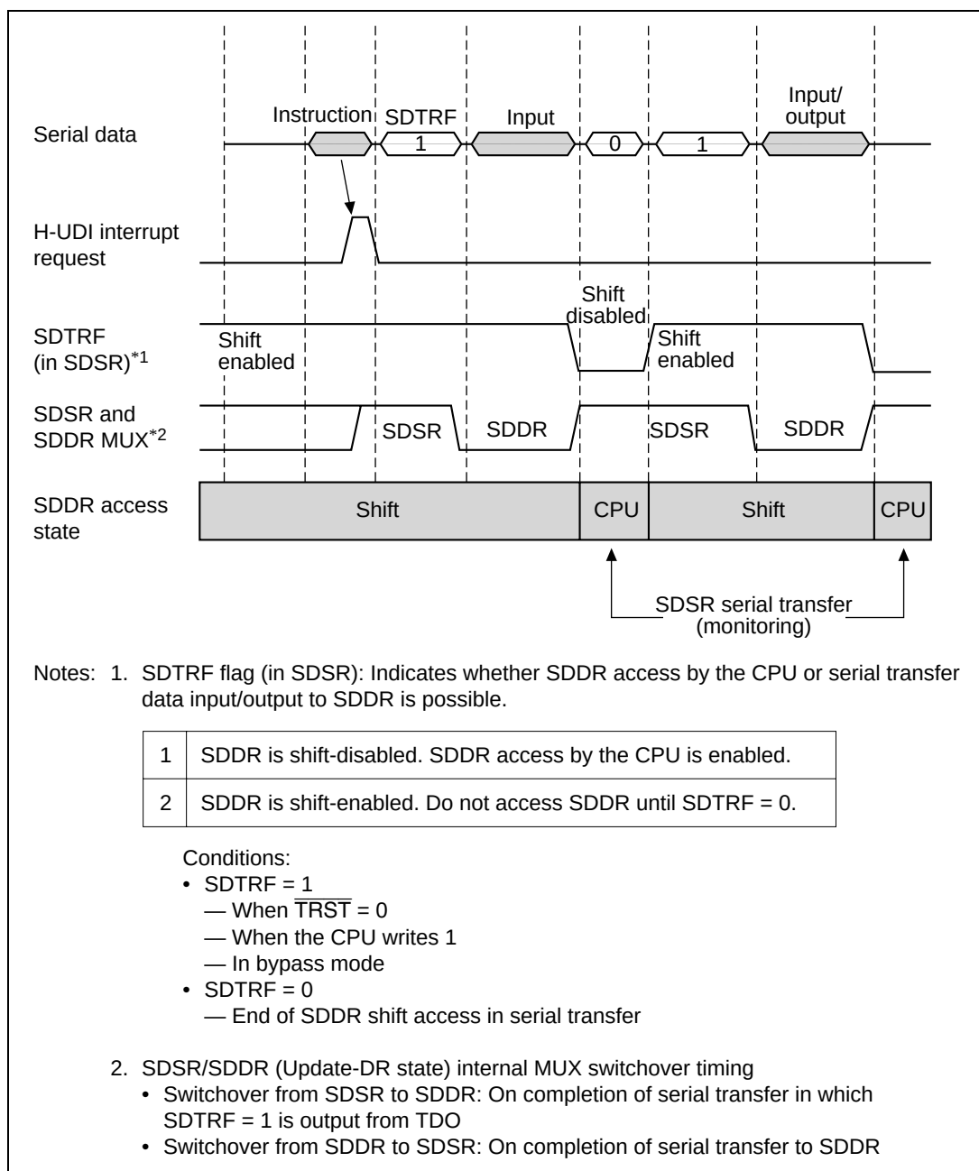
Figure 17.3 Data Input/Output Timing Chart (1)
