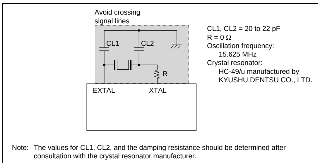
Figure 3.5 Points for Attention when Using Crystal Resonator
