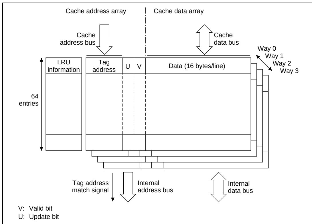
Figure 8.1 Cache Configuration
