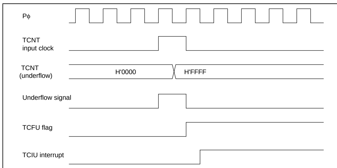
Figure 16.41 TCIU Interrupt Setting Timing
