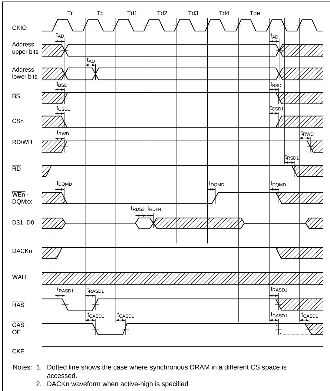
Figure 21.17 Synchronous DRAM Single Read Bus Cycle (RCD = 1 Cycle, CAS Latency = 1 Cycle, Burst = 4)
