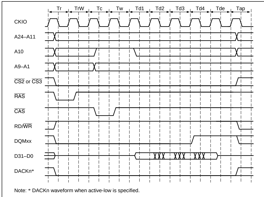
Figure 7.20 (a) Burst Read Wait Specification Timing (Auto-Precharge) Except t_{E_{CYC}}:t_{P_{CYC}} 1:1
