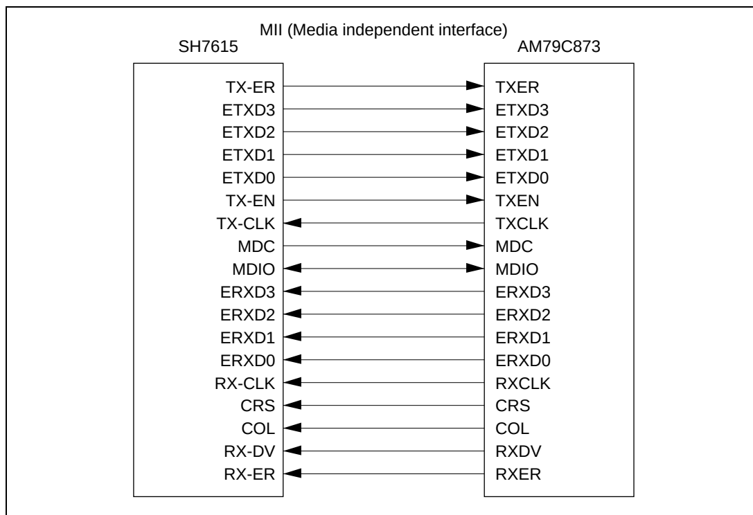
Figure 9.7 Example of Connection to AM79C873
