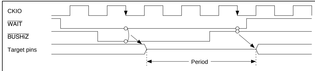
Figure 7.60 \overline{\text{BUSHiZ}} Bus Timing
