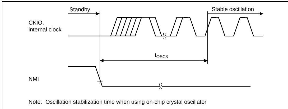
Figure 21.7 Oscillation Stabilization Time after Standby Recovery (Recovery by NMI)
