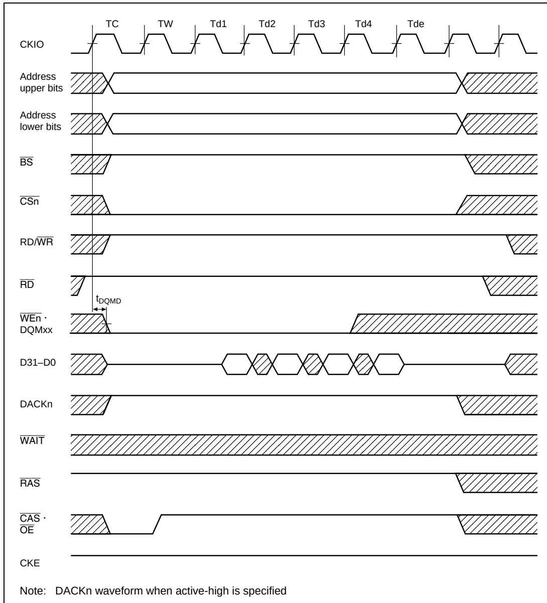
Figure 21.20 Synchronous DRAM Read Bus Cycle (Bank Active, Same Row Access, CAS Latency = 2 Cycles)
