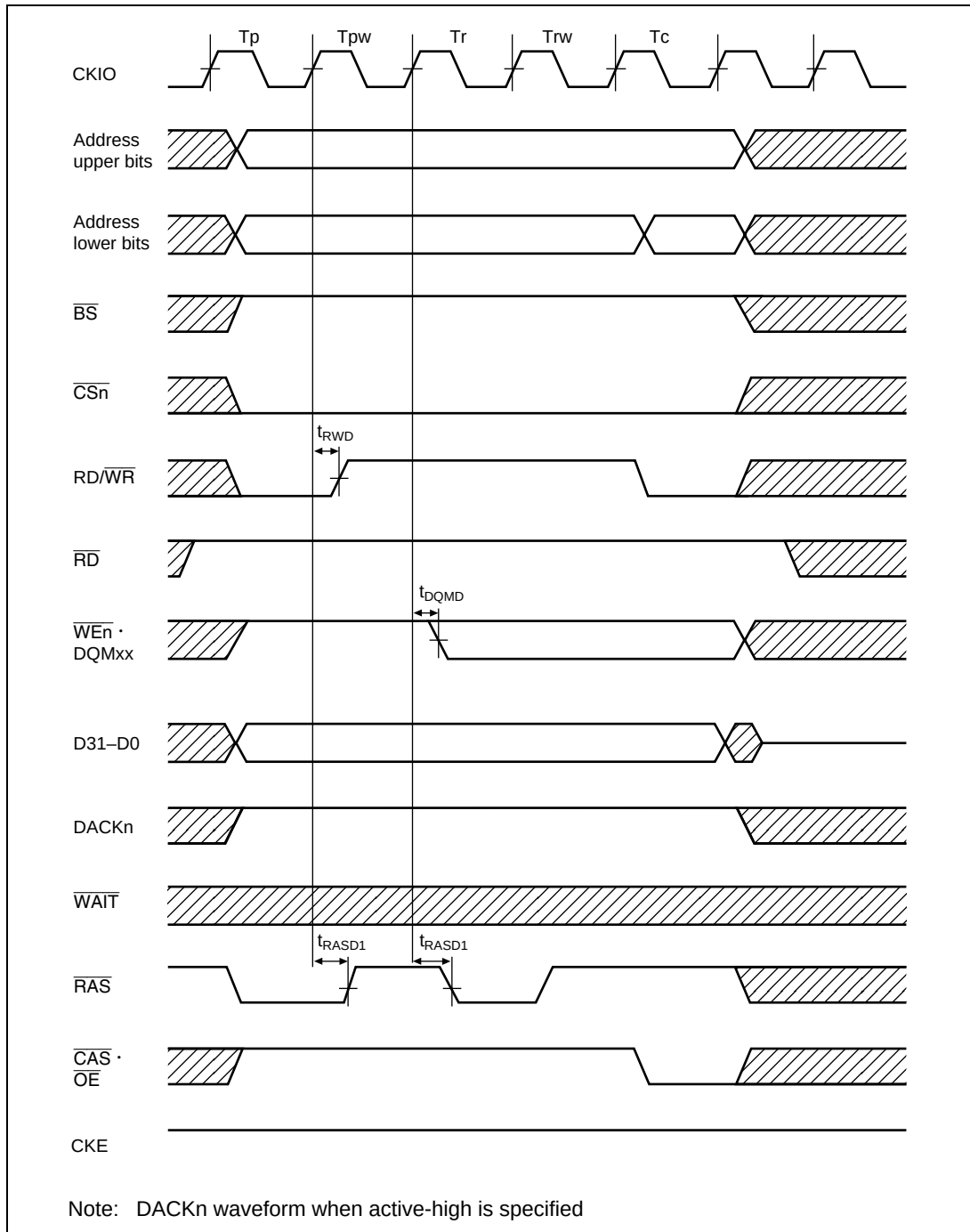
Figure 21.30 Synchronous DRAM Write Bus Cycle (Bank Active, Different Row Access, TRP = 2 Cycles, RCD = 2 Cycles)
