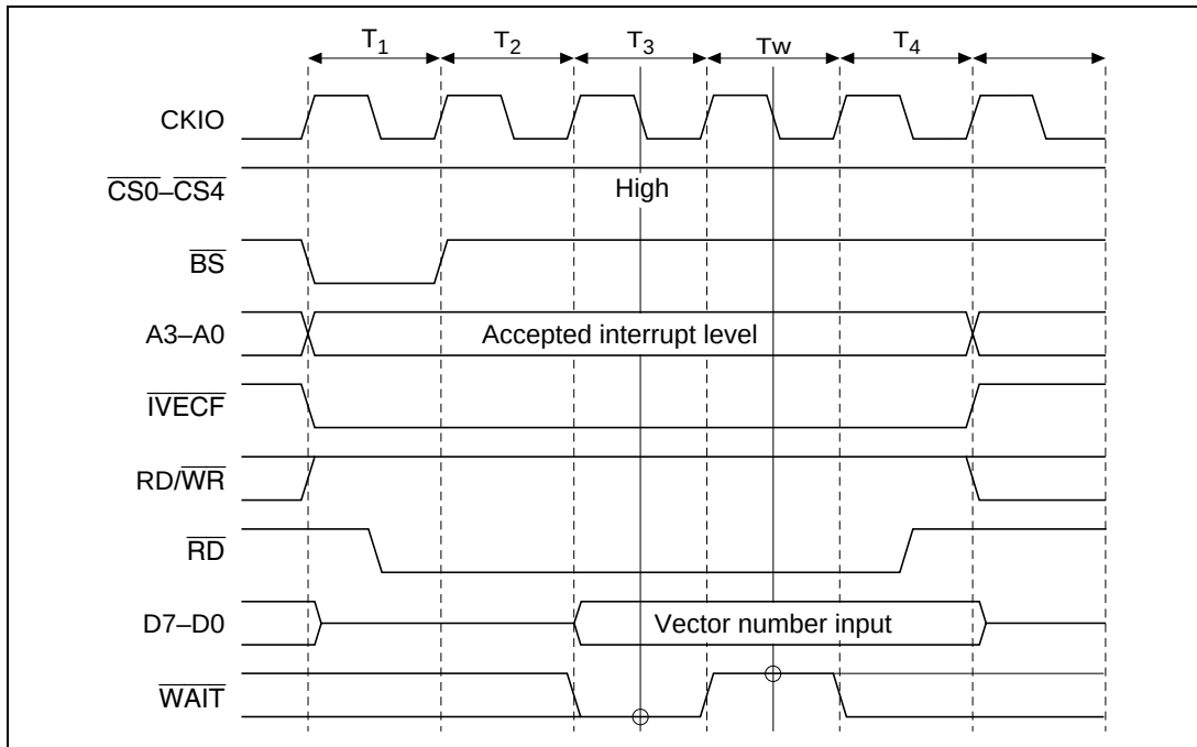
Figure 5.6 External Vector Fetch ( I\phi:E\phi = 1:1 ( \overline{WAIT} Input))
