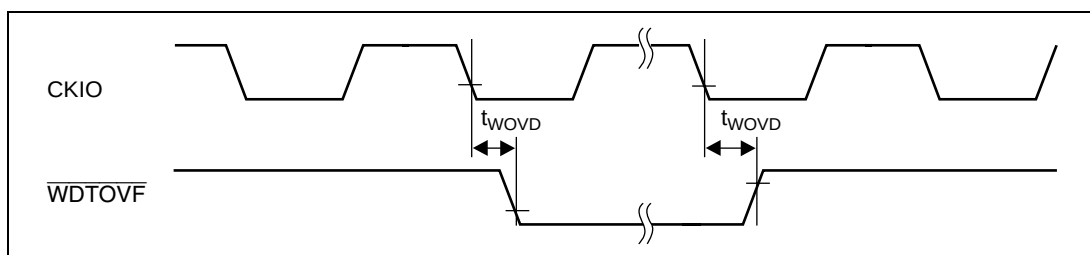
Figure 21.60 Watchdog Timer Output Timing (Except t_{\text{Ecy}}:t_{\text{Pcy}} 1:1 )
