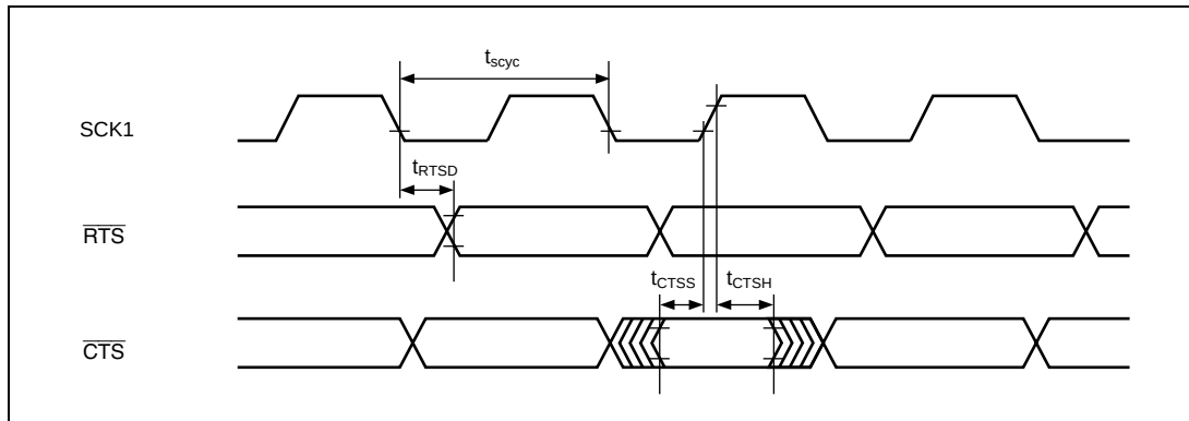
Figure 21.55 \overline{\text{RTS}} and \overline{\text{CTS}} Input/Output Timing
