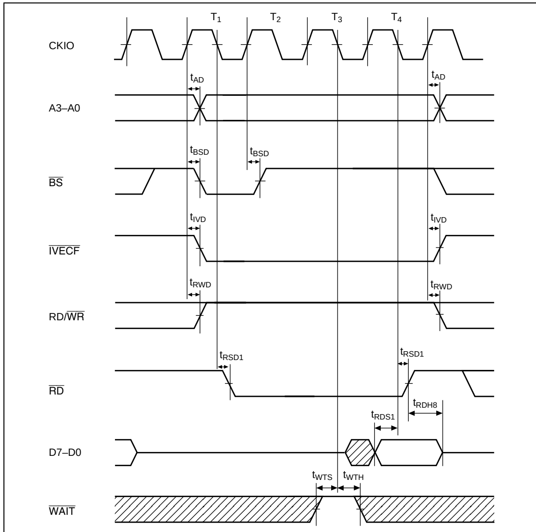
Figure 21.44 Interrupt Vector Fetch Cycle (No Wait, I\phi:E\phi = 1:1 )
