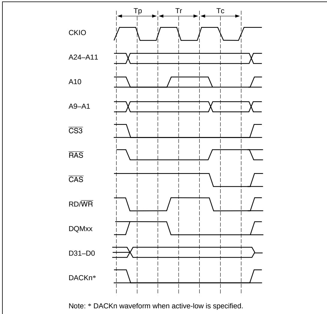
Figure 7.29 Single Write Mode Timing (Bank Active, Different Row Addresses)
