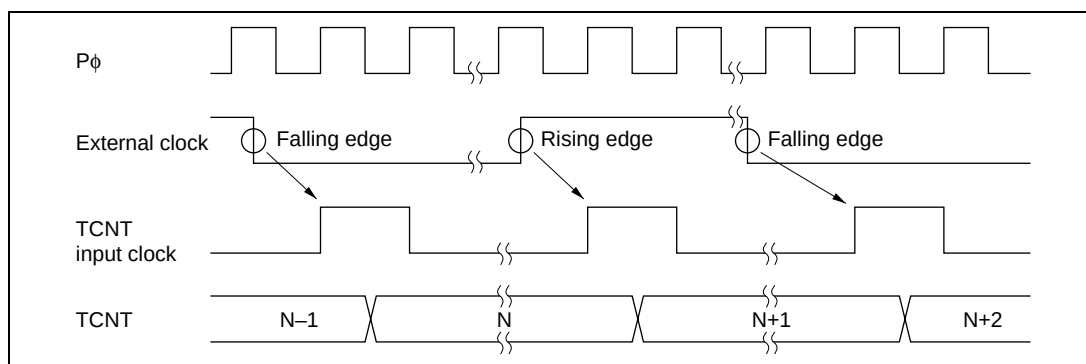
Figure 16.31 Count Timing in External Clock Operation
