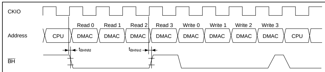
Figure 21.79 \overline{\text{BH}} Output Timing
