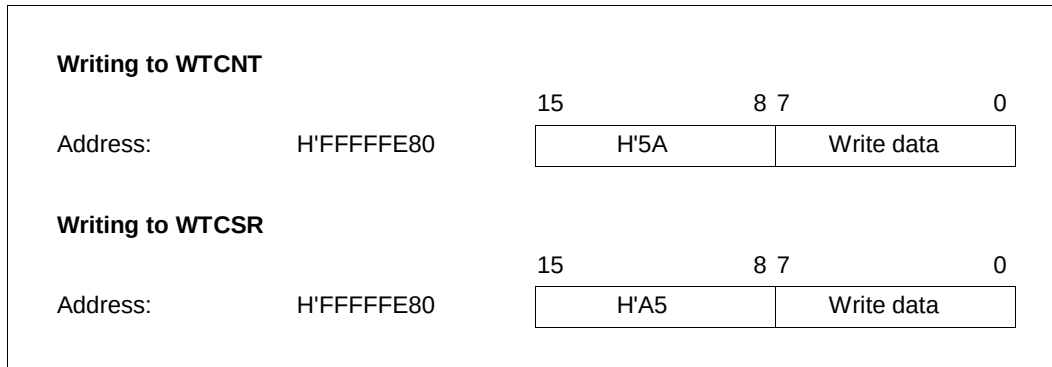
Figure 13.2 Writing to WTCNT and WTCNR
