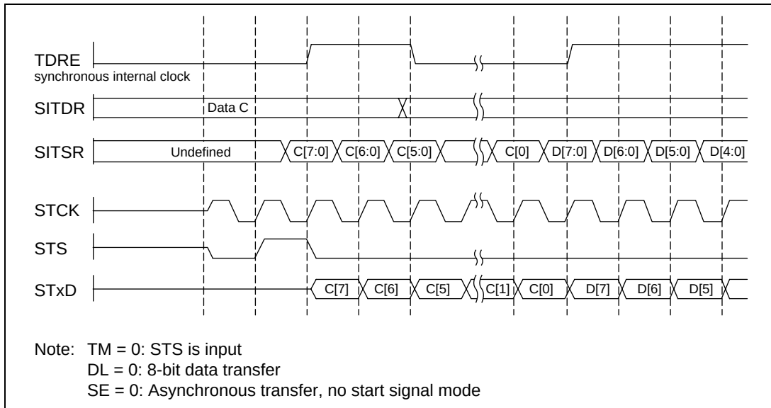
Figure 15.5 Transmission: Continuous Transfer Mode (TM = 0 Mode)
