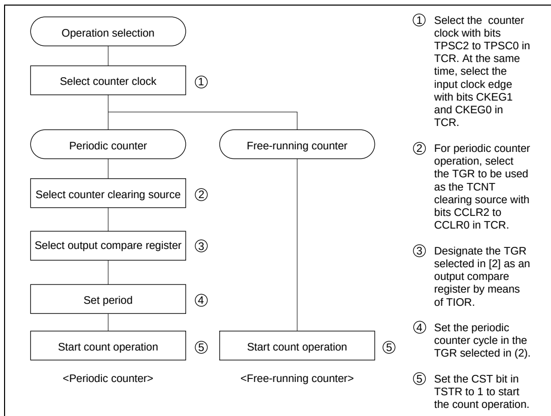
Figure 16.6 Example of Counter Operation Setting Procedure
