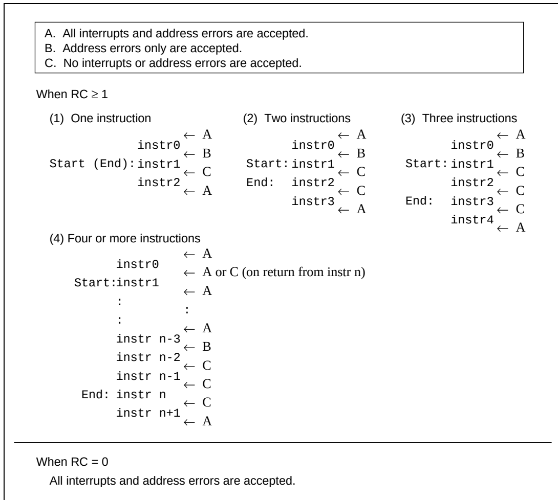
Figure 4.1 Interrupt Acceptance Restrictions in Repeat Mode
