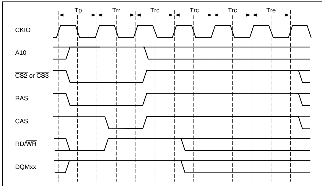
Figure 7.30 Auto-Refresh Timing
