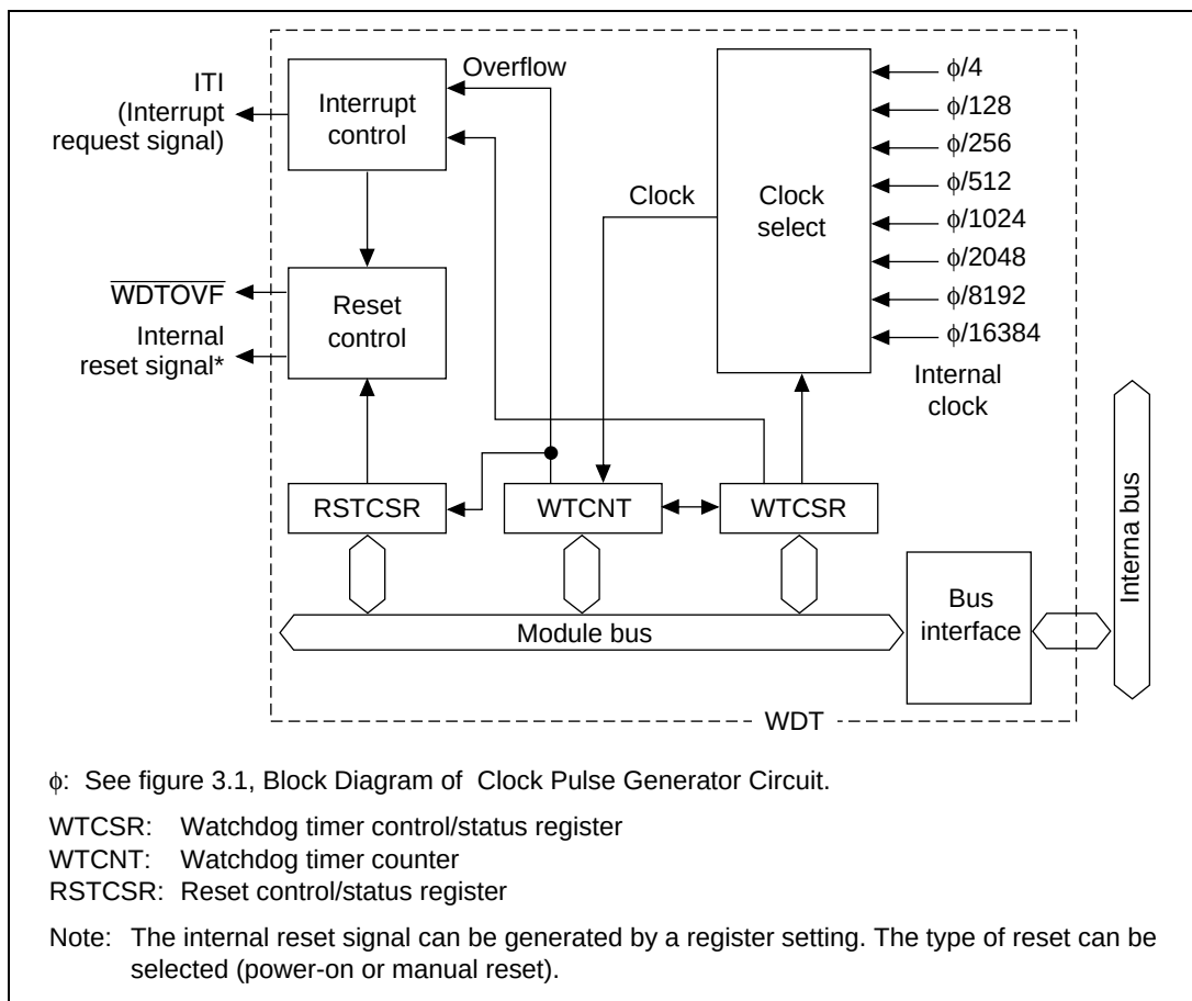
Figure 13.1 WDT Block Diagram
