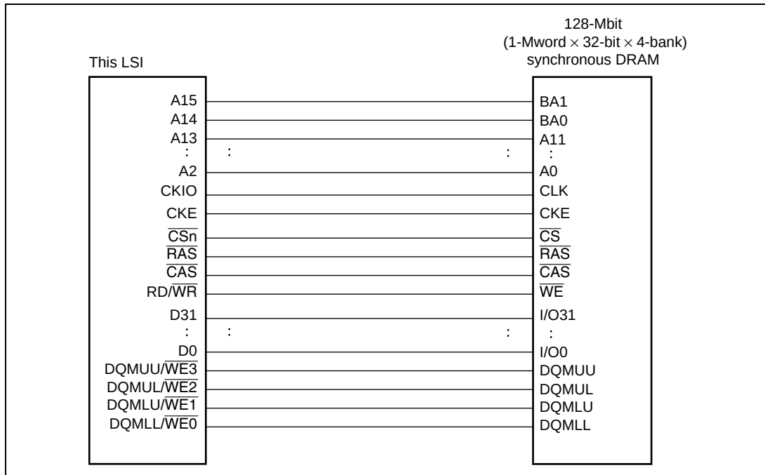
Figure 7.35 128-Mbit Synchronous DRAM (4 Mwords × 32 Bits) Connection Example
