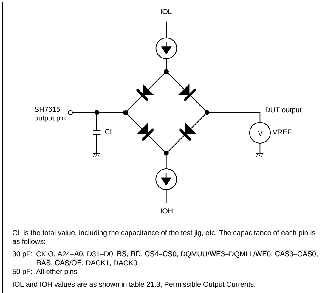
Figure 21.81 Output Load Circuit
