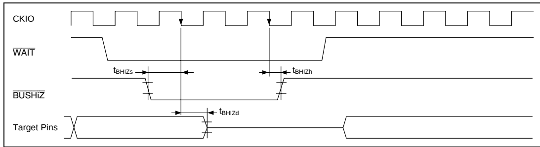
Figure 21.80 \overline{\text{BUSHiZ}} Bus Timing
