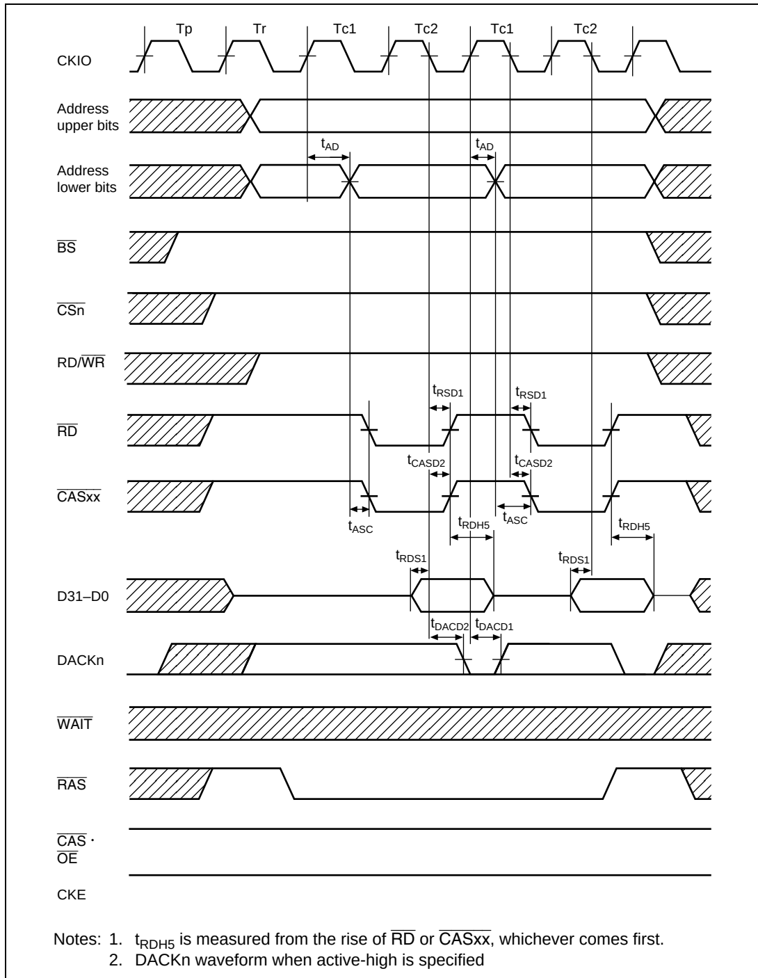
Figure 21.38 DRAM Burst Read Cycle (TRP = 1 Cycle, RCD = 1 Cycle, No Wait)
