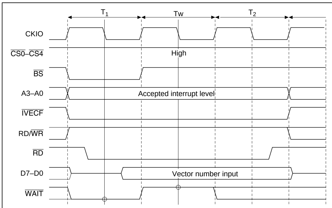
Figure 5.7 External Vector Fetch ( I\phi:E\phi \neq 1:1 ( \overline{WAIT} Input))
