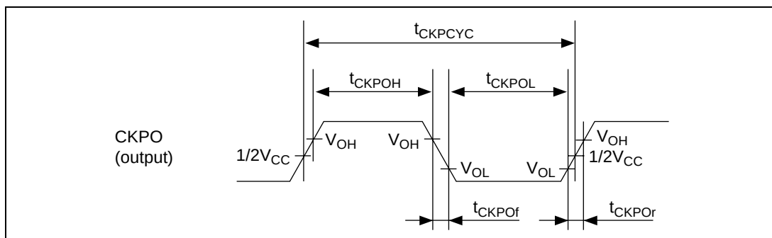
Figure 21.4 CKPO Clock Output Timing
