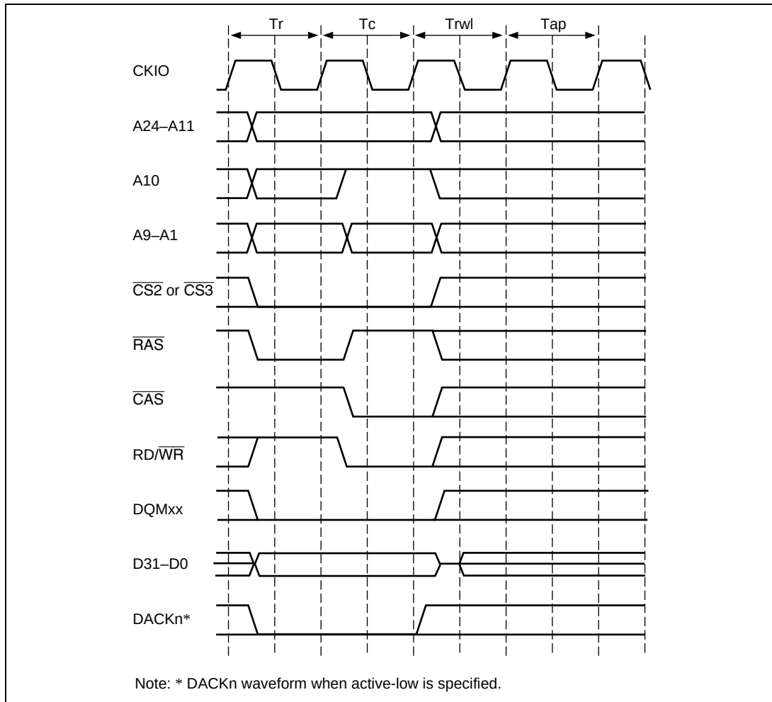
Figure 7.22 Basic Single Write Cycle Timing (Auto-Precharge)
