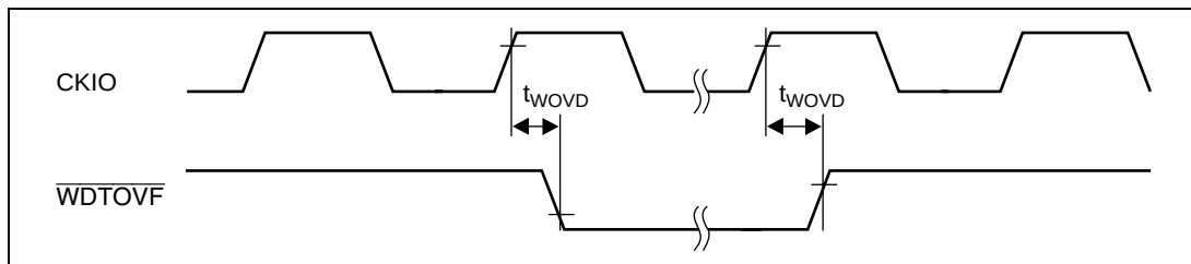
Figure 21.59 Watchdog Timer Output Timing ( t_{\text{Ecy}}:t_{\text{Pcy}} = 1:1 )
