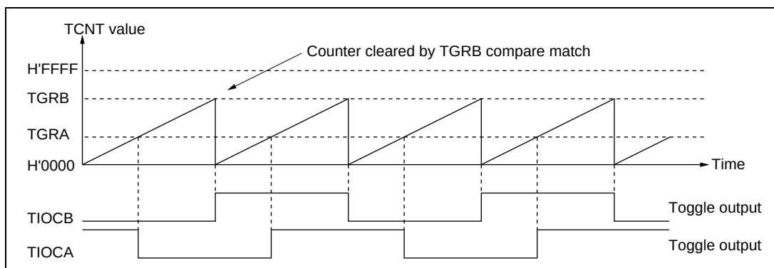
Figure 16.11 Example of Toggle Output Operation
