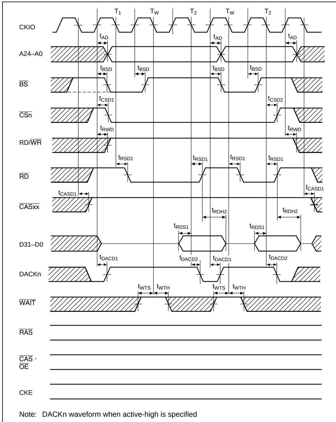
Figure 21.43 Burst ROM Read Cycle (Wait = 1)
