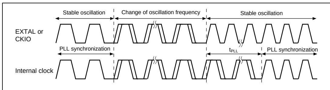
Figure 21.8 PLL Synchronization Stabilization Time
