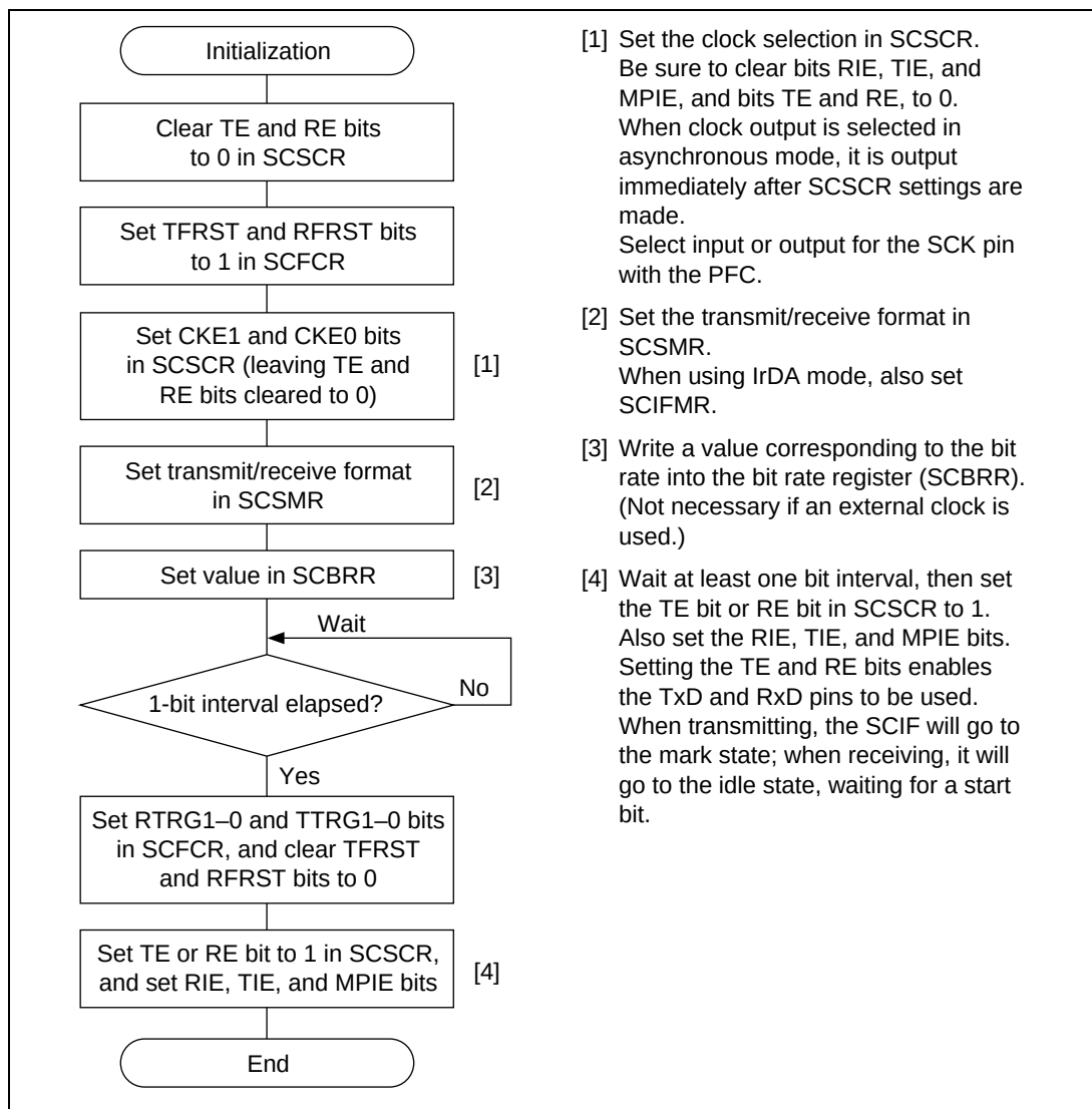
Figure 14.4 Sample SCIF Initialization Flowchart
