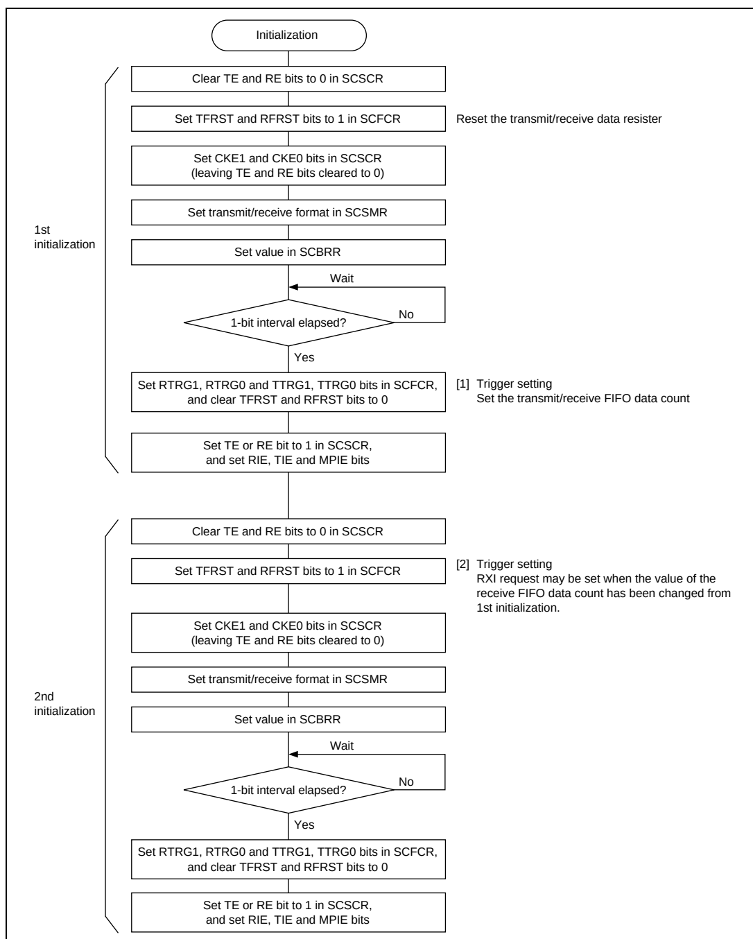
Figure 14.27 Example of SCIF Initialization Flowchart
