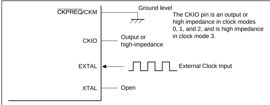
Figure 3.3 External Clock Input Method
