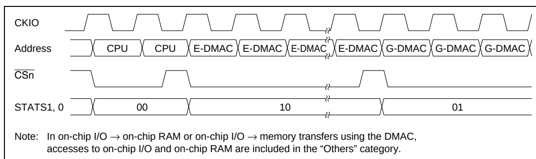
Figure 7.59 STATS Output Timing
