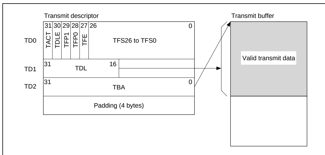
Figure 10.2 Relationship between Transmit Descriptor and Transmit Buffer
