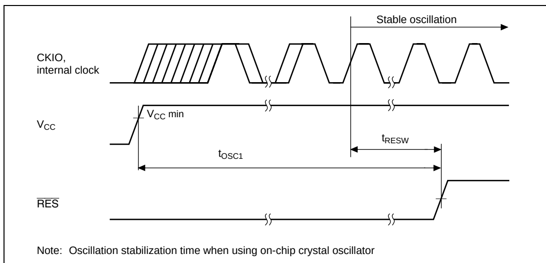
Figure 21.5 Power-On Oscillation Stabilization Time at Power-On
