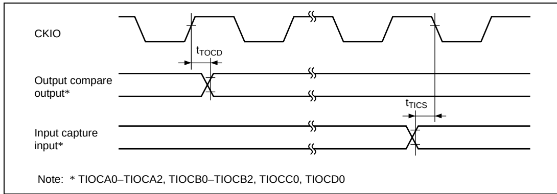
Figure 21.56 TPU Input/Output Timing ( t_{E_{cyc}}:t_{P_{cyc}} = 1:1 )
