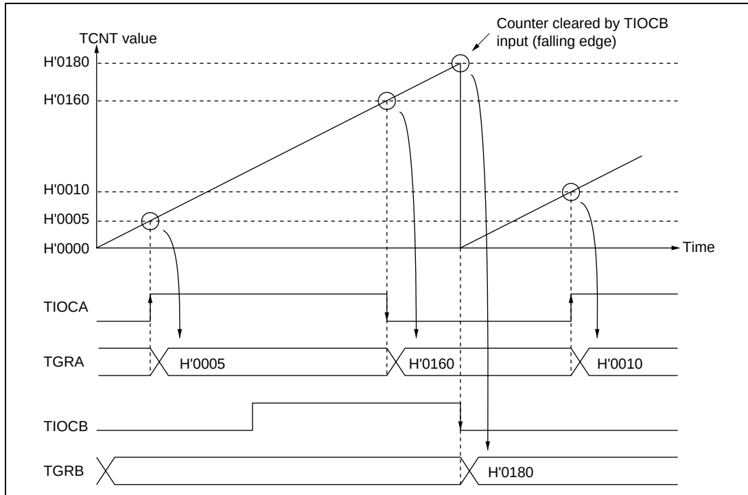
Figure 16.13 Example of Input Capture Operation
