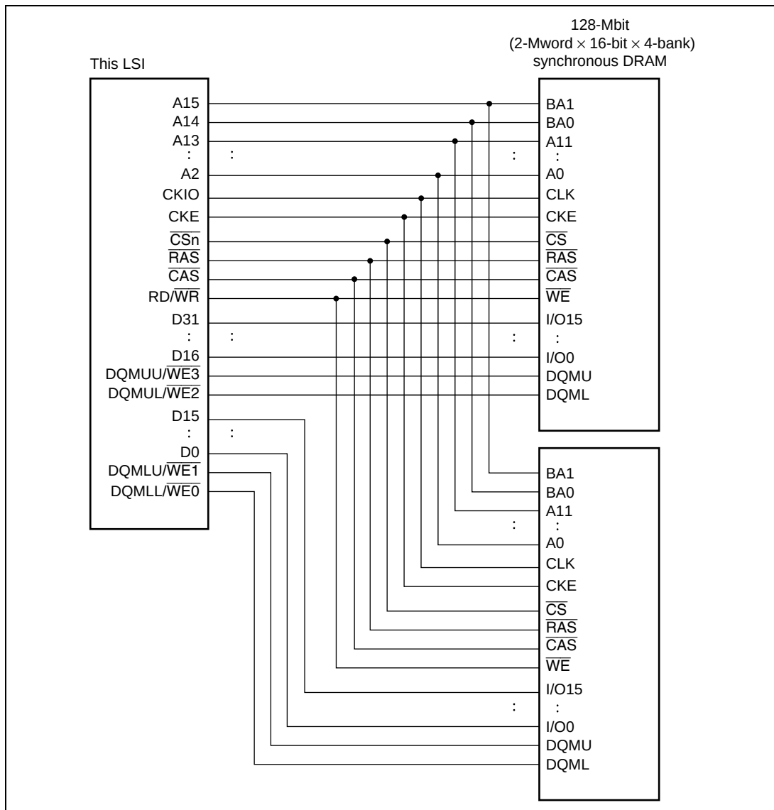
Figure 7.36 128-Mbit Synchronous DRAM (8 Mwords \times 16 Bits) Connection Example
