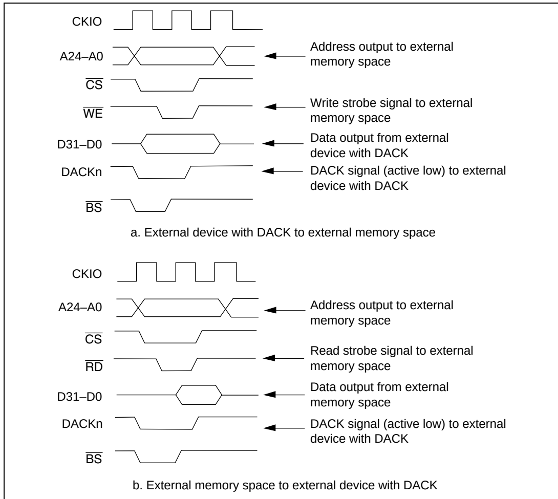
Figure 11.7 DMA Transfer Timing in Single Address Mode
