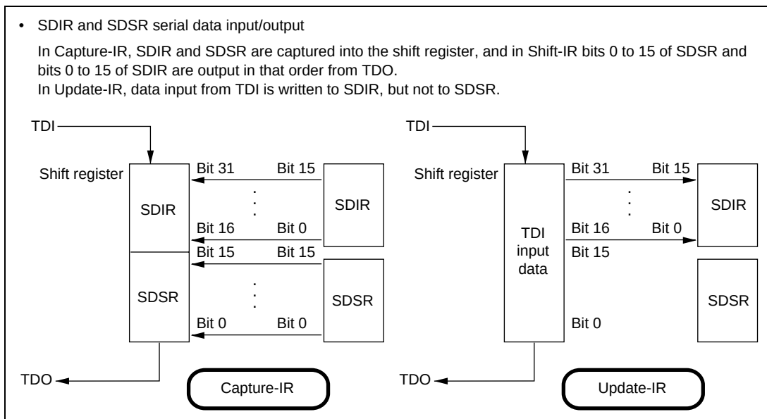
Figure 17.6 Serial Data Input/Output (1)
