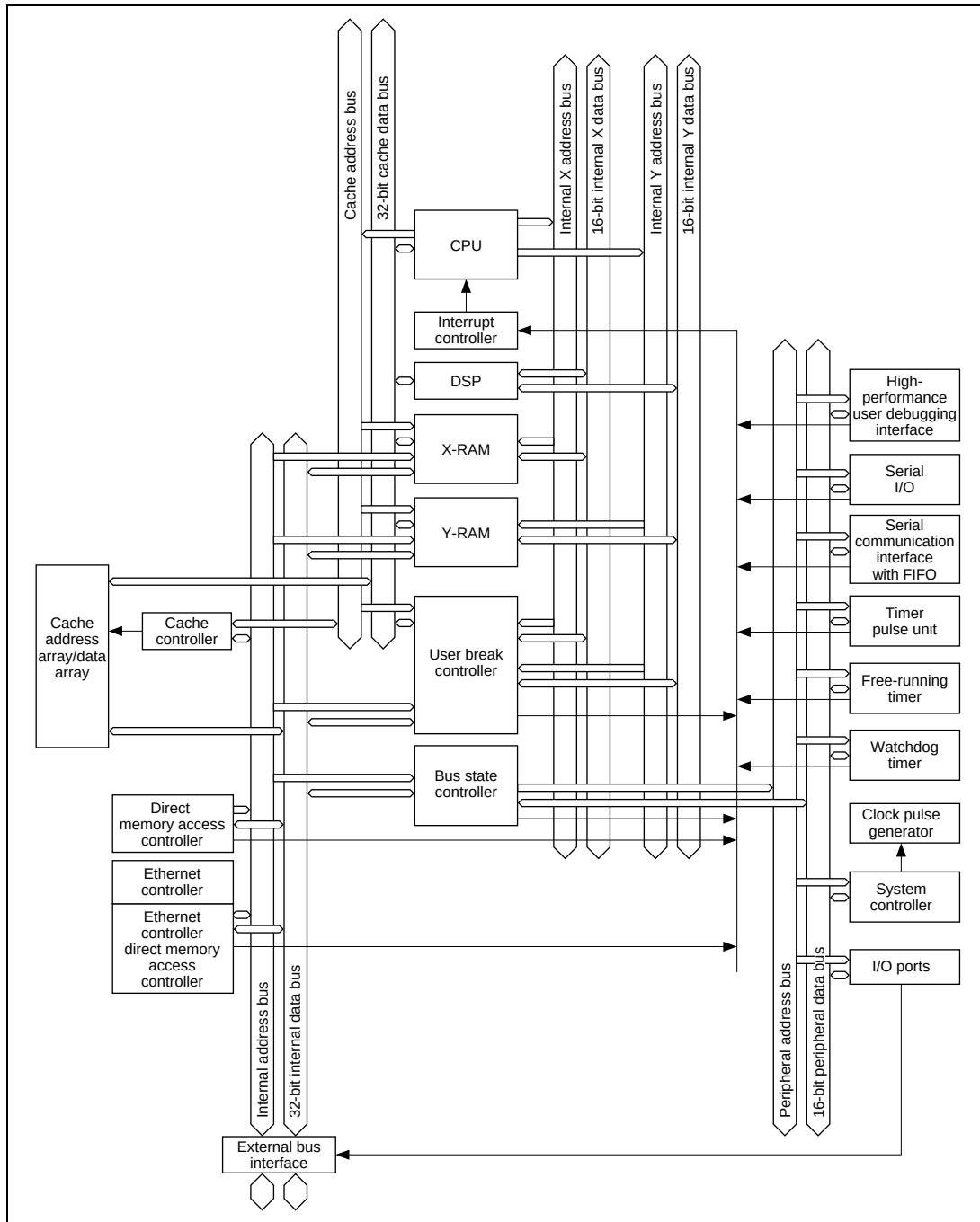
Figure 1.1 Block Diagram of SH7615
