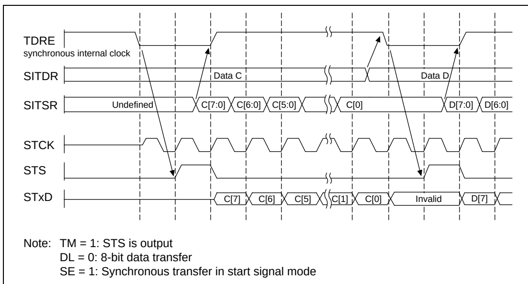
Figure 15.6 Transmission: Interval Transfer Mode (TM = 1 Mode)
