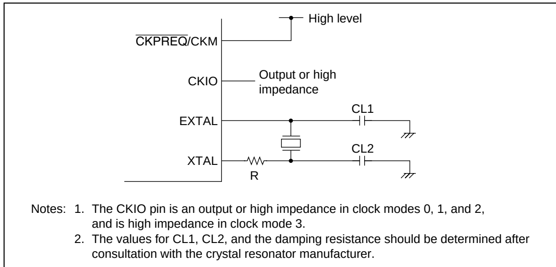
Figure 3.2 Example of Crystal Oscillator Connection
