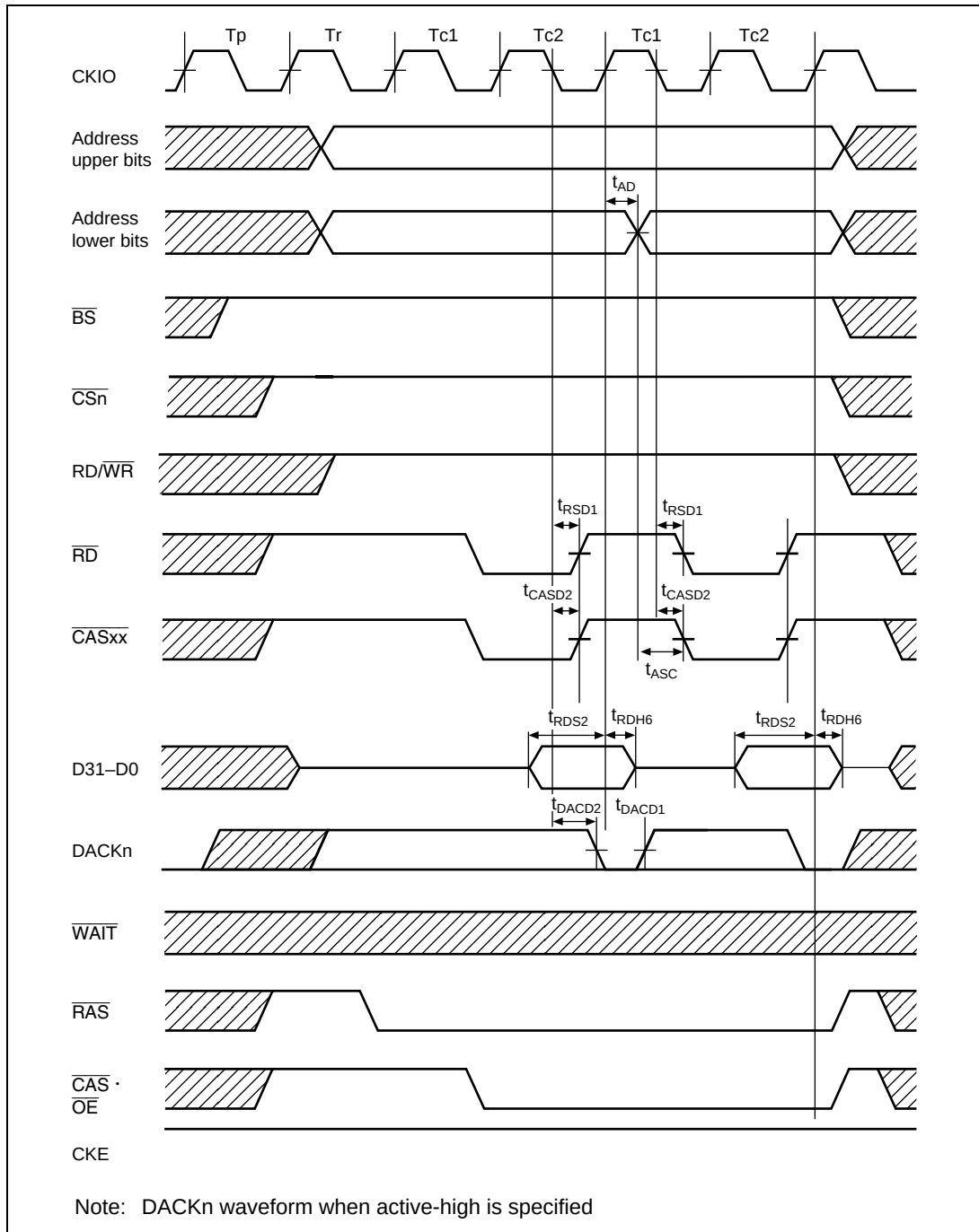
Figure 21.41 EDO Burst Read Cycle (TRP = 1 Cycle, RCD = 1 Cycle, No Wait)
