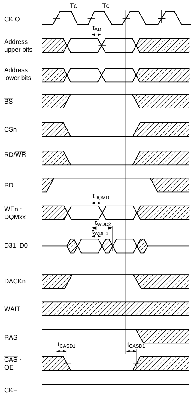
Figure 21.28 Synchronous DRAM Continuous Write Cycle (Bank Active, Same Row Access, Iφ:Eφ = 1:1)
