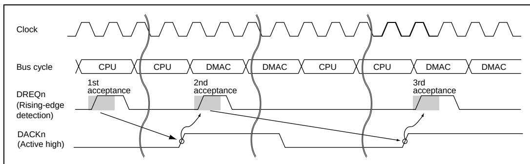
Figure 11.33 DREQn/DACKn Handshaking
