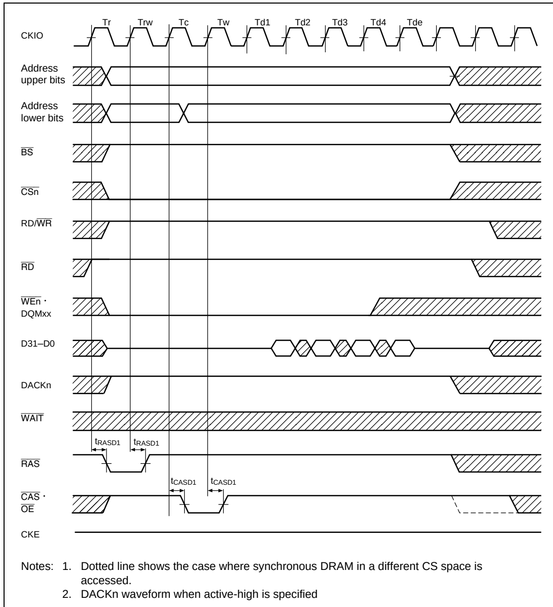
Figure 21.18 Synchronous DRAM Read Bus Cycle (RCD = 2 Cycles, CAS Latency = 2 Cycles, Burst = 4)
