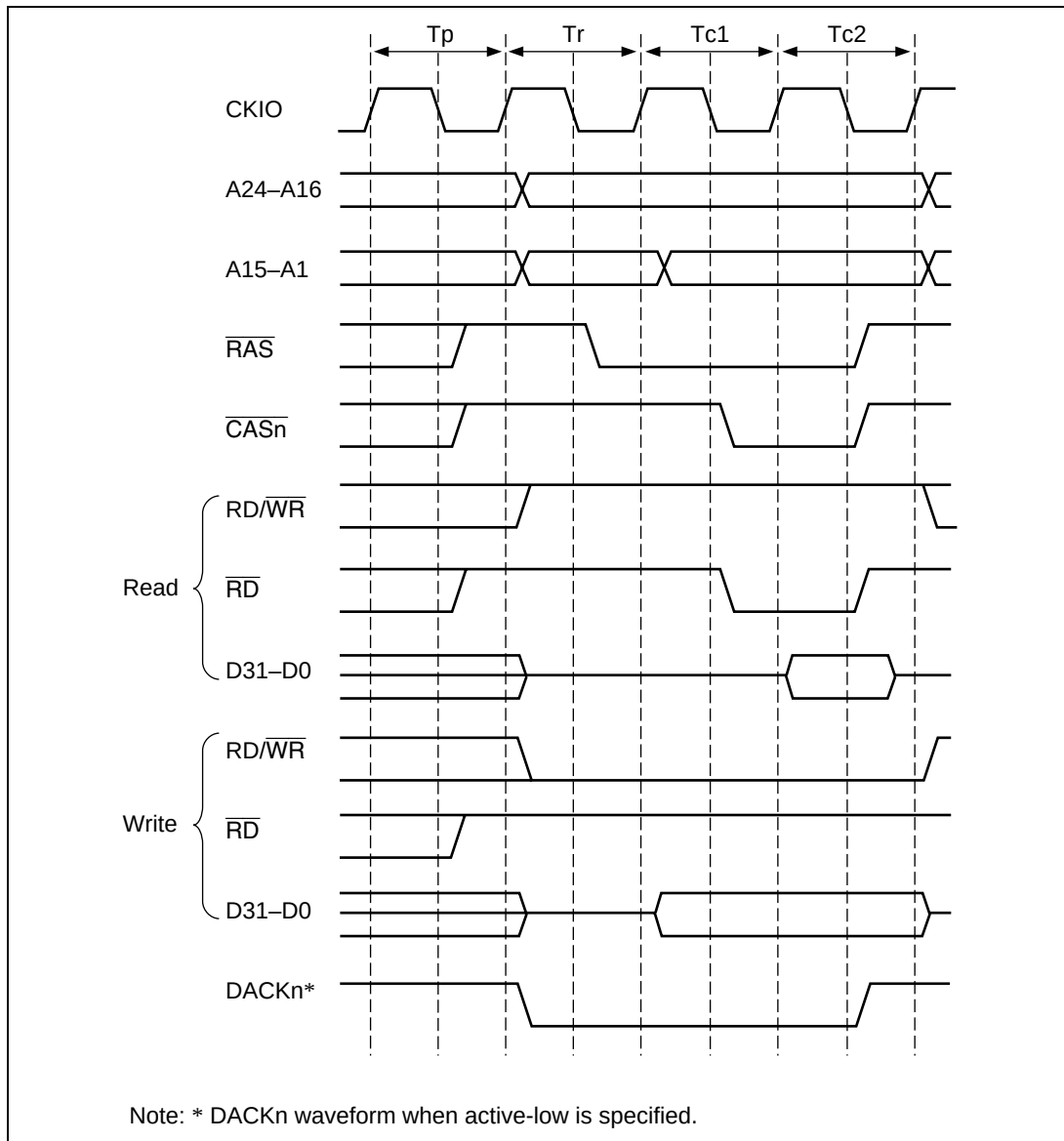
Figure 7.40 Basic Access Timing
