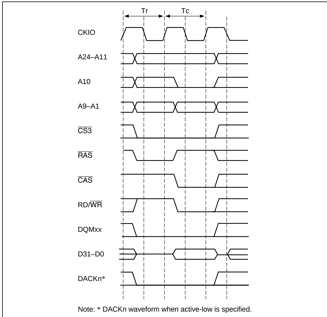
Figure 7.27 Single Write Mode Timing (No Precharge)
