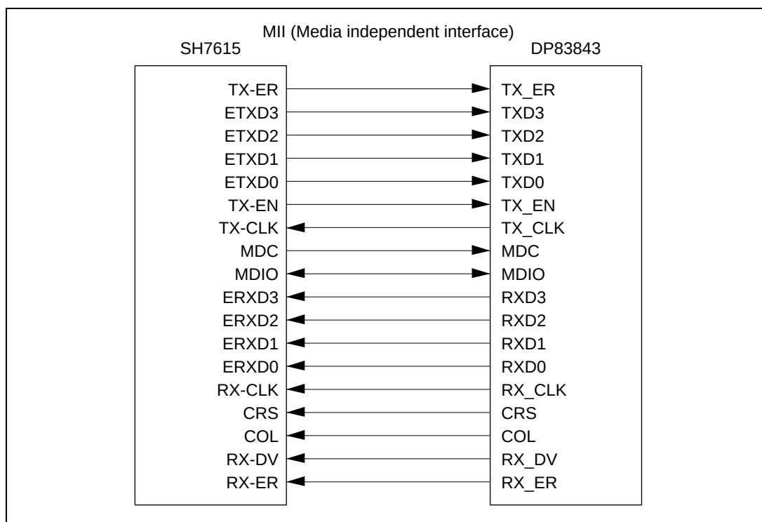
Figure 9.8 Example of Connection to DP83843
