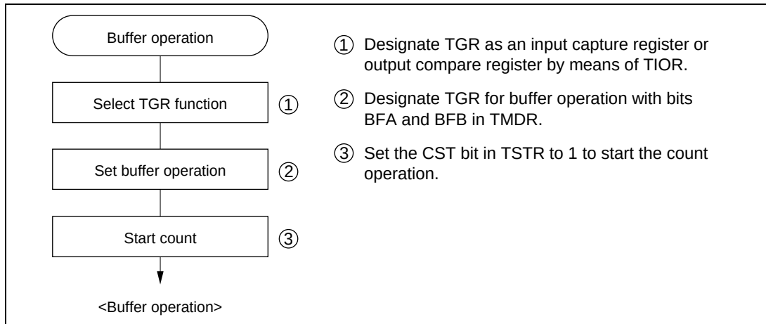
Figure 16.18 Example of Buffer Operation Setting Procedure
