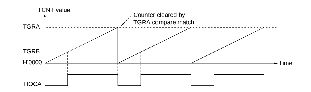
Figure 16.22 Example of PWM Mode Operation (1)
