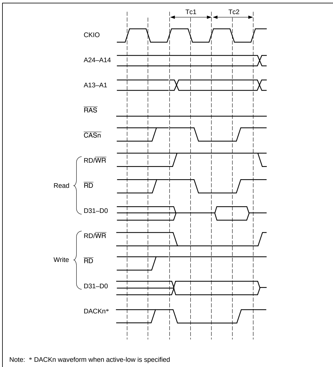
Figure 7.44 \overline{RAS} Down Mode Same Row Access Timing
