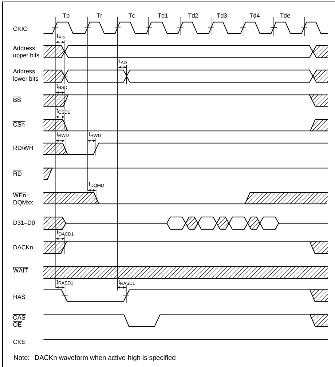
Figure 21.21 Synchronous DRAM Read Bus Cycle (Bank Active, Different Row Access, TRP = 1 Cycle, RCD = 1 Cycle, CAS Latency = 1 Cycle)
