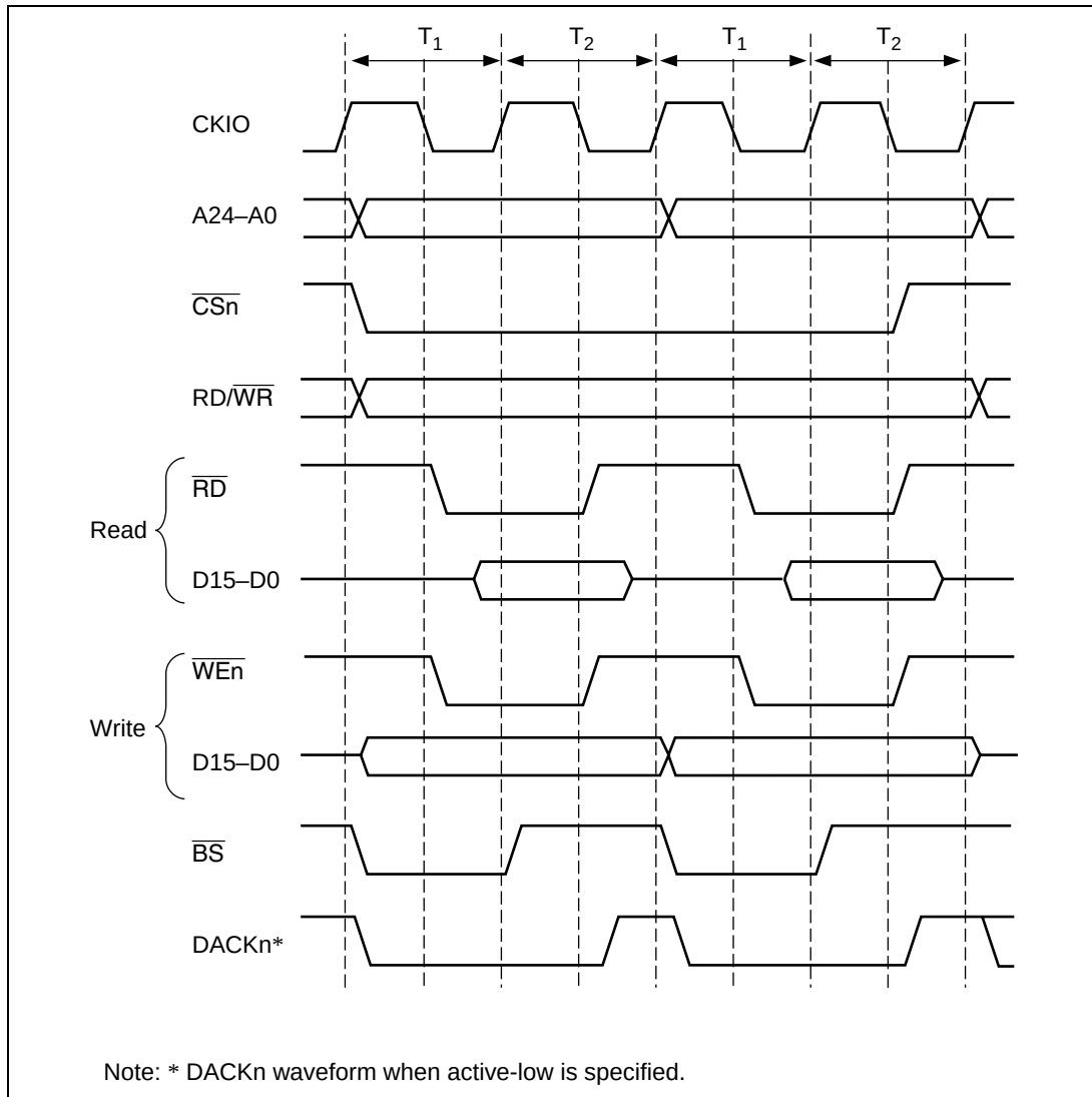
Figure 7.9 Timing of Longword Access in Ordinary Space Using 16-Bit Bus Width (Clock Ratio Iφ:Eφ = 1:1)
