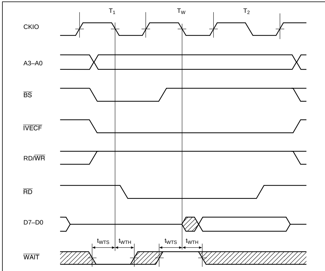
Figure 21.46 Interrupt Vector Fetch Cycle (External Wait Input, Except t_{E\text{cyc}}:t_{P\text{cyc}} 1:1)
