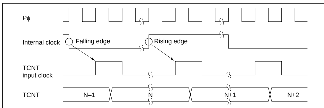
Figure 16.30 Count Timing in Internal Clock Operation
