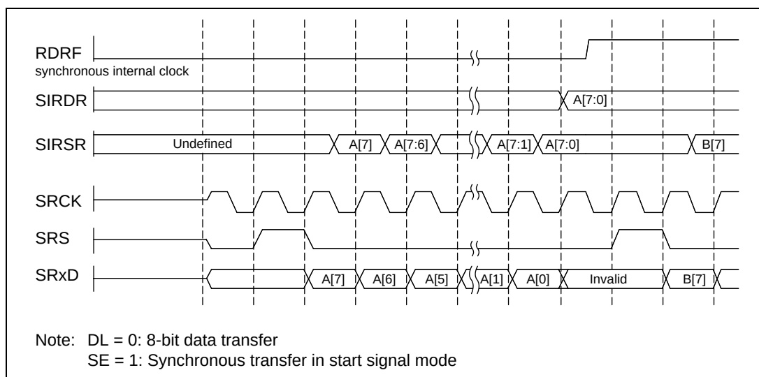
Figure 15.2 Reception: Interval Transfer Mode
