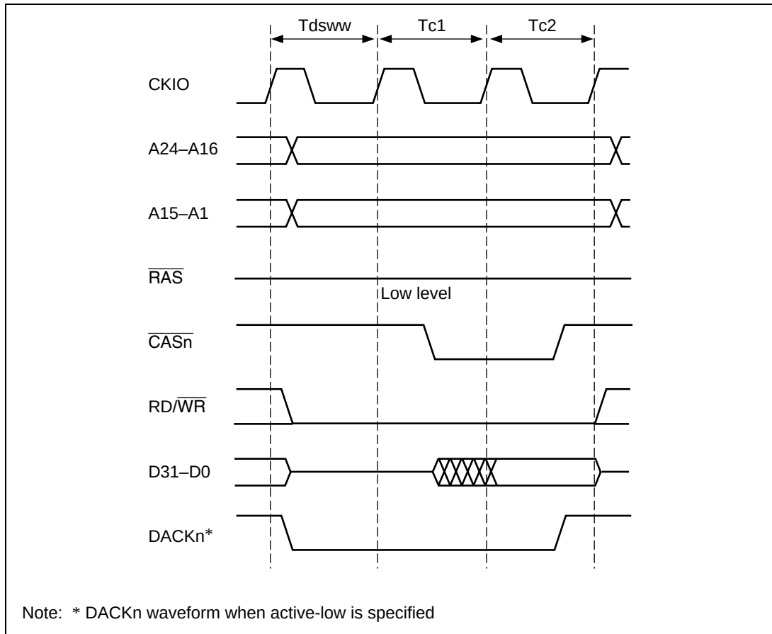
Figure 7.50 DMA Single Transfer Mode Write Cycle Timing (RAS Down Mode, Same Row Address)
