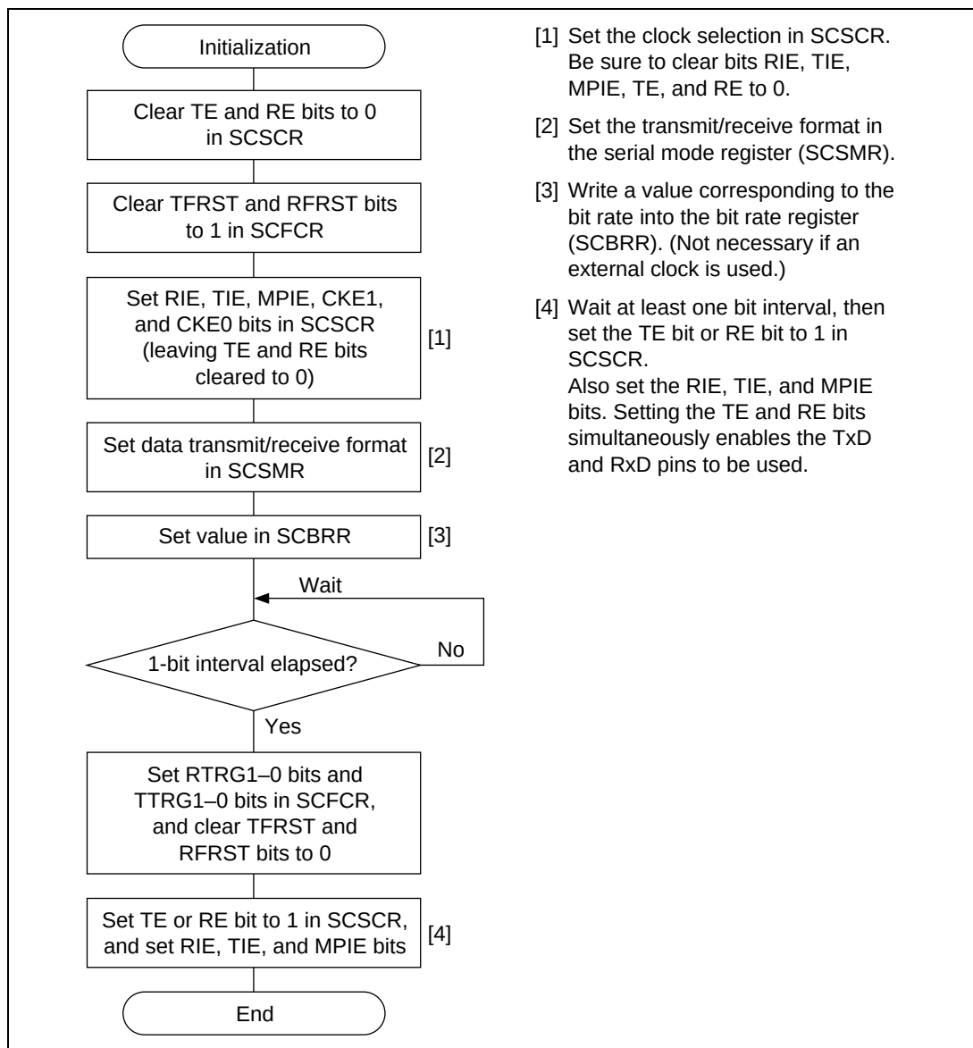
Figure 14.17 Sample SCIF Initialization Flowchart
