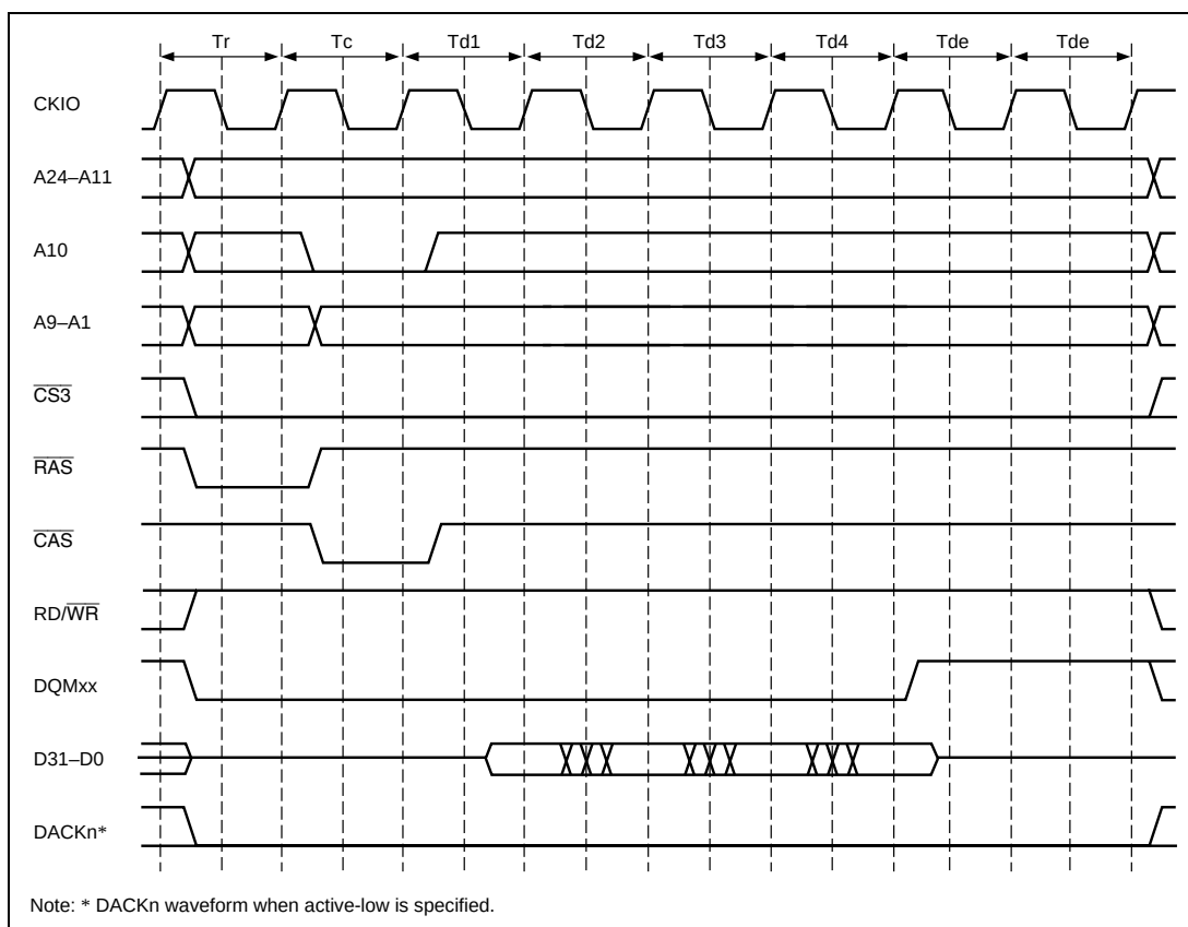
Figure 7.24 (b) Burst Read Timing (No Precharge) I\phi:E\phi = 1:1
