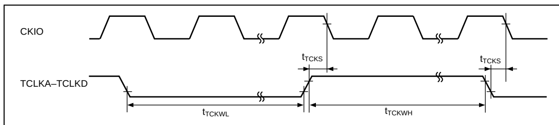
Figure 21.58 TPU Clock Input Timing
