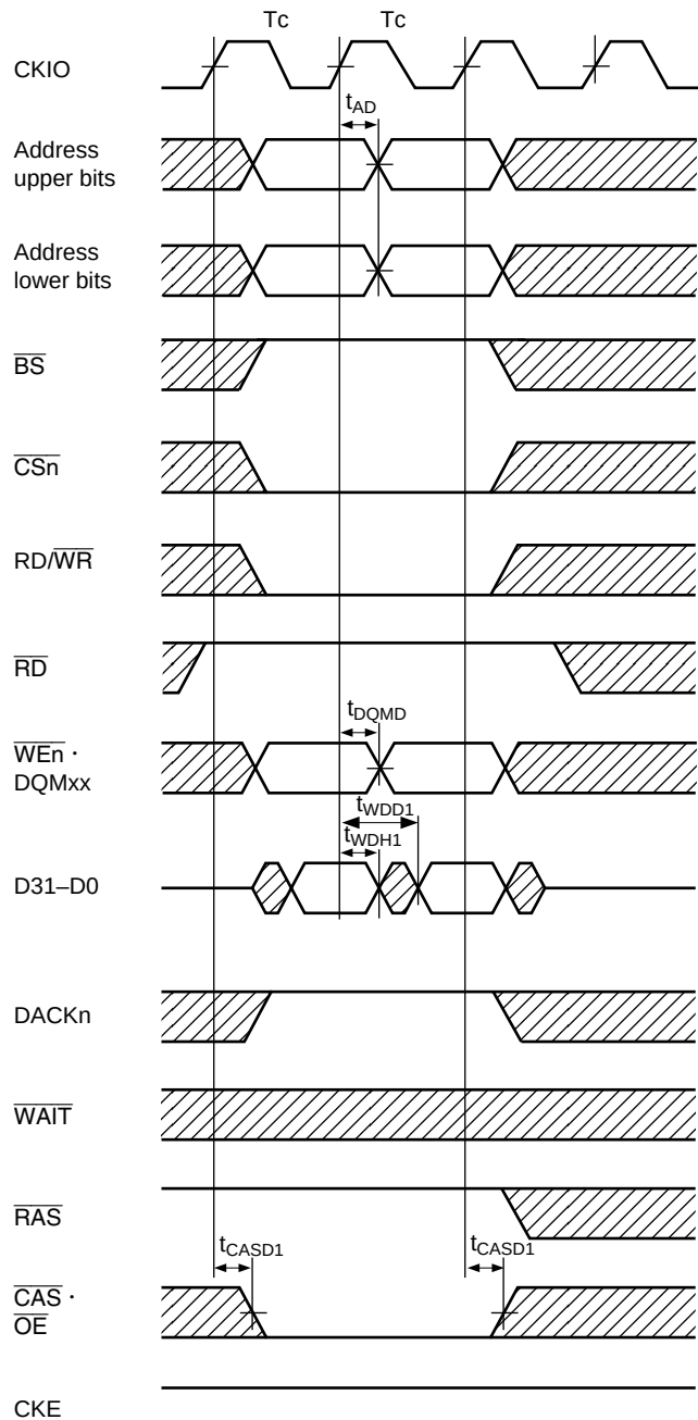
Figure 21.27 Synchronous DRAM Continuous Write Cycle (Bank Active, Same Row Access, Except t_{E\text{cyc}}:t_{P\text{cyc}} 1:1)
