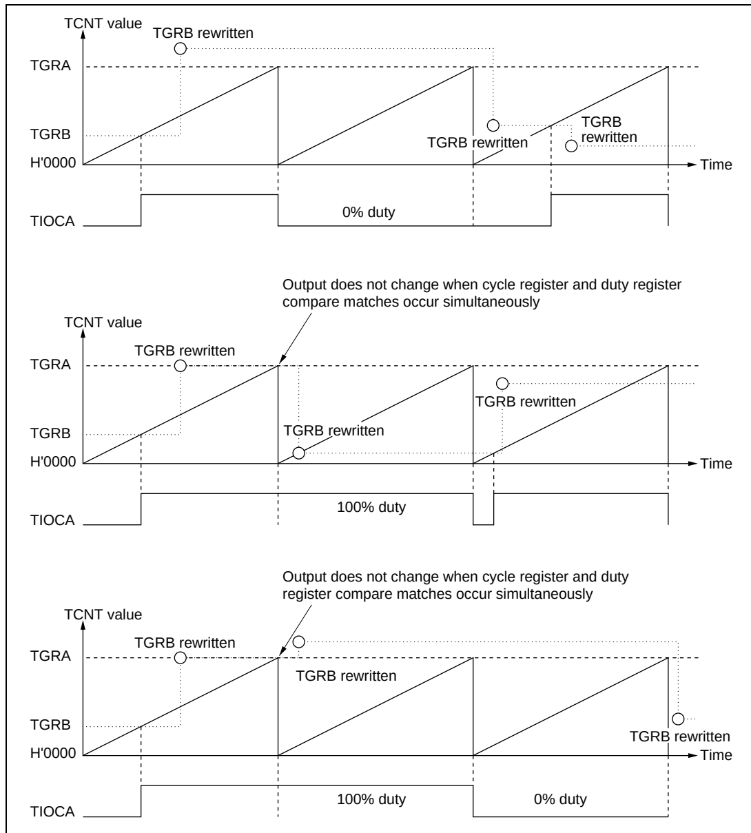
Figure 16.24 Example of PWM Mode Operation (3)
