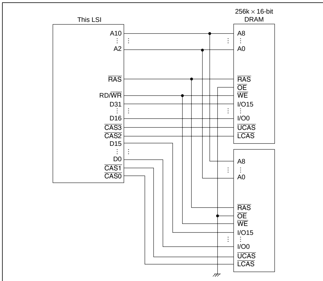
Figure 7.38 Example of DRAM Connection (32-Bit Data Width)
