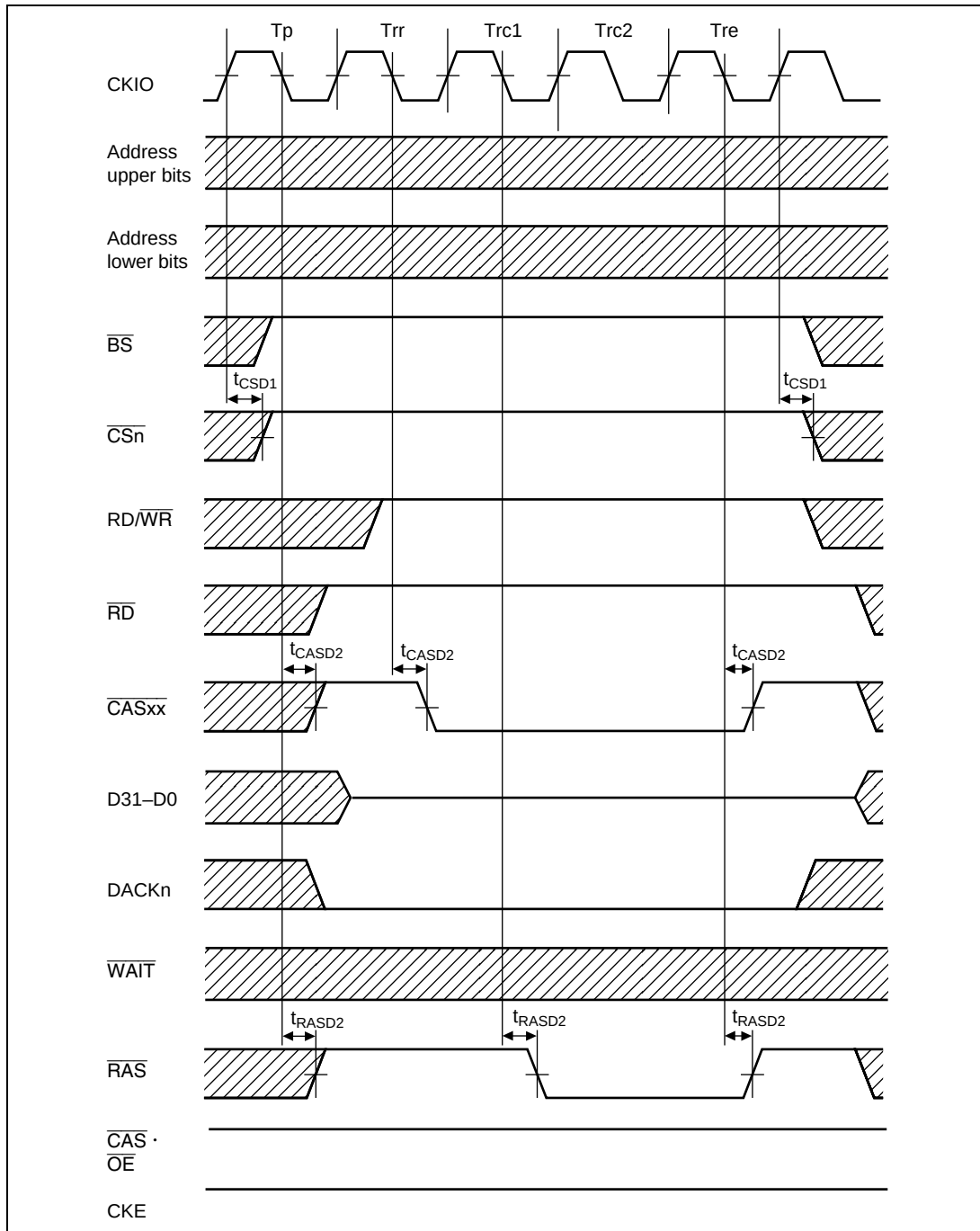
Figure 21.42 DRAM \overline{\text{CAS}} -Before- \overline{\text{RAS}} Refresh Cycle ( \text{TRP} = 1 \text{ Cycle} , \text{TRAS} = 2 \text{ Cycles} )
