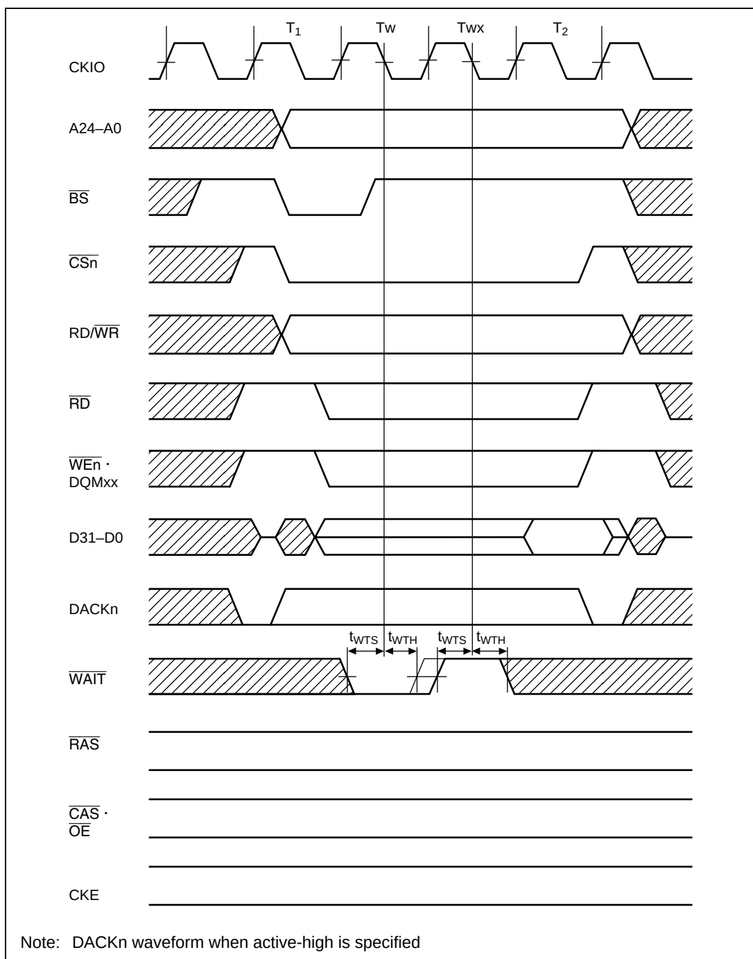
Figure 21.15 Basic Bus Cycle (External Wait Input)
