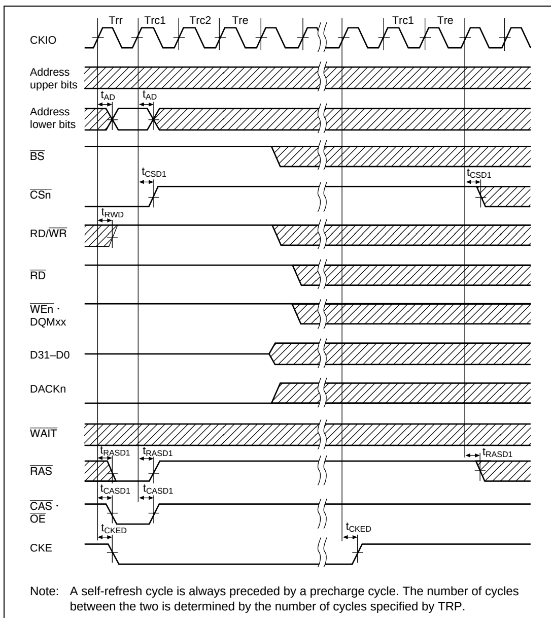
Figure 21.33 Synchronous DRAM Self-Refresh Cycle ( TRAS = 3 )
