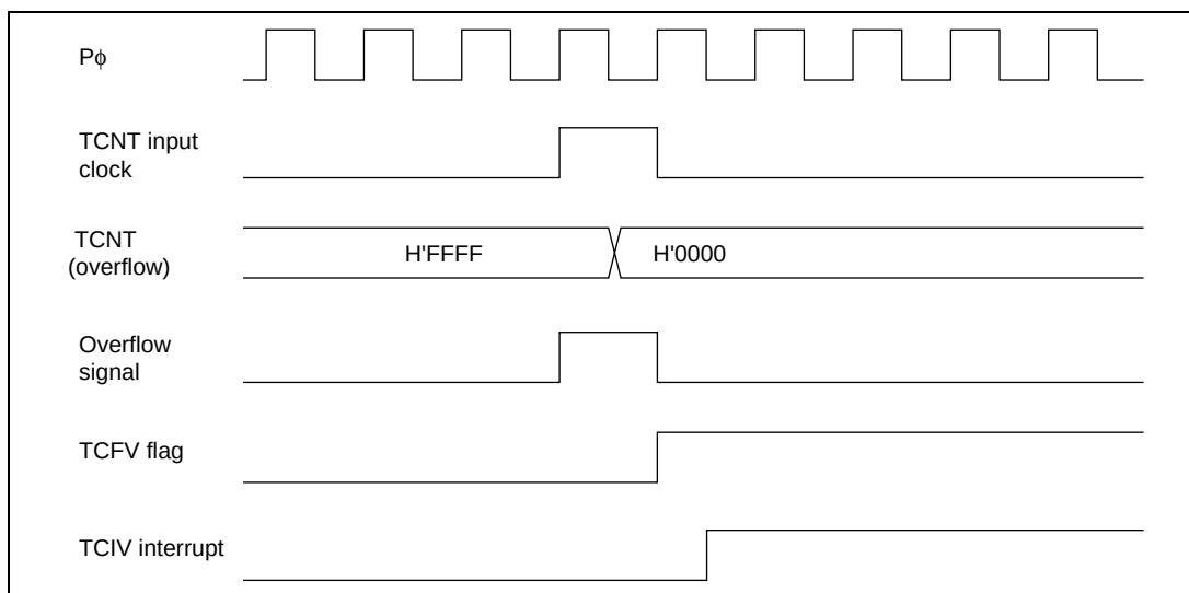
Figure 16.40 TCIV Interrupt Setting Timing
