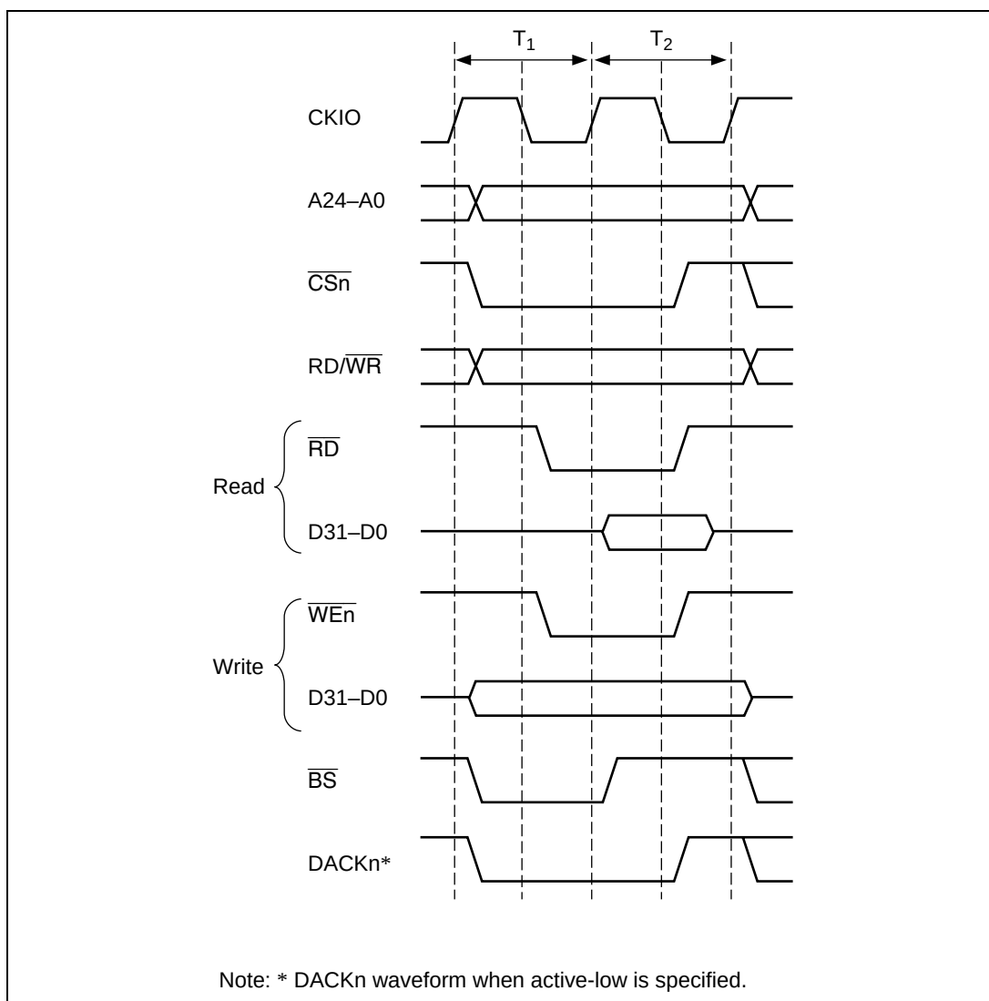
Figure 7.8 Basic Timing of Ordinary Space Access
