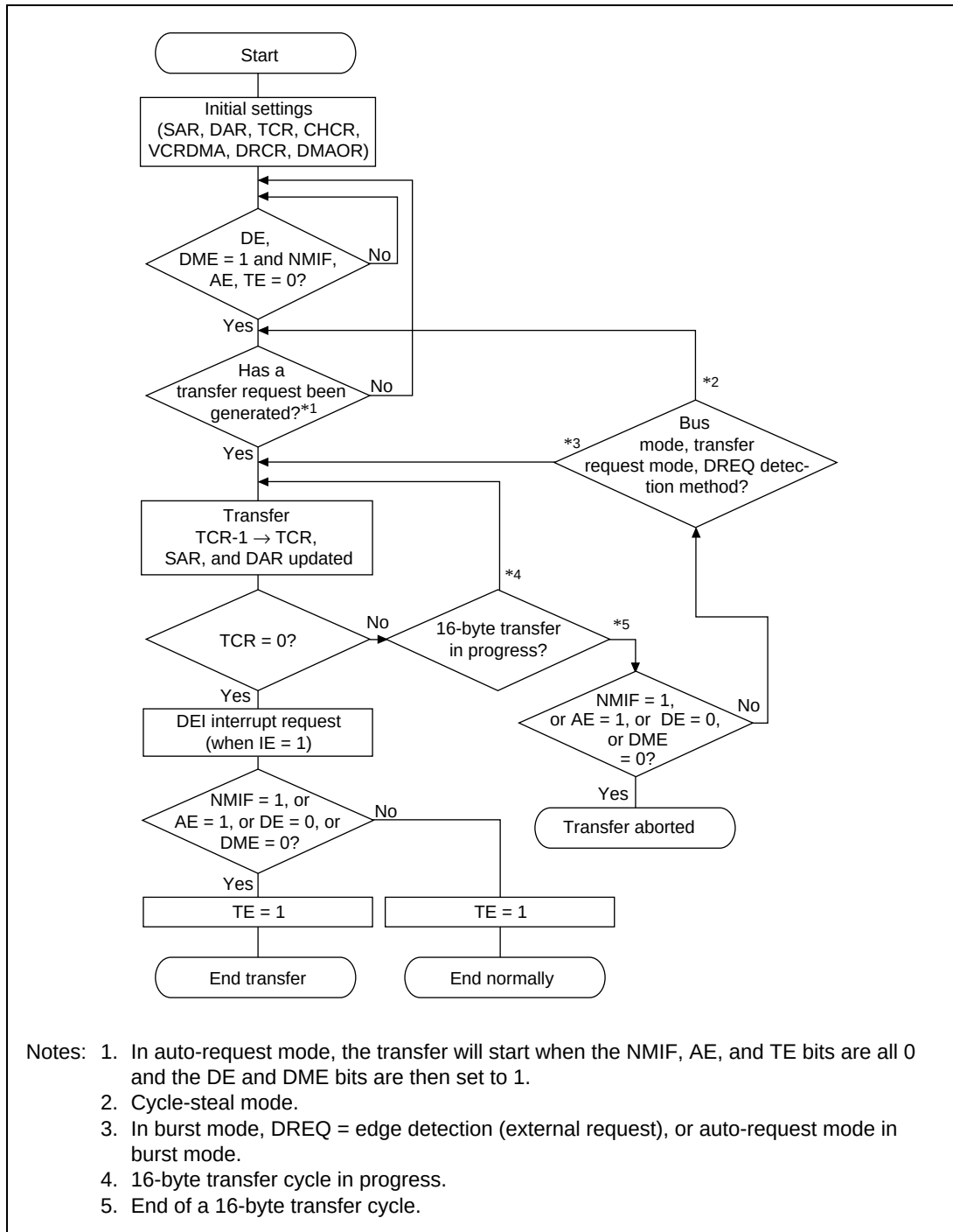
Figure 11.2 DMA Transfer Flow
