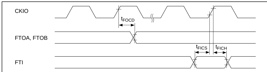
Figure 21.49 FRT Input/Output Timing ( t_{E_{cyc}}:t_{P_{cyc}} = 1:1 )
