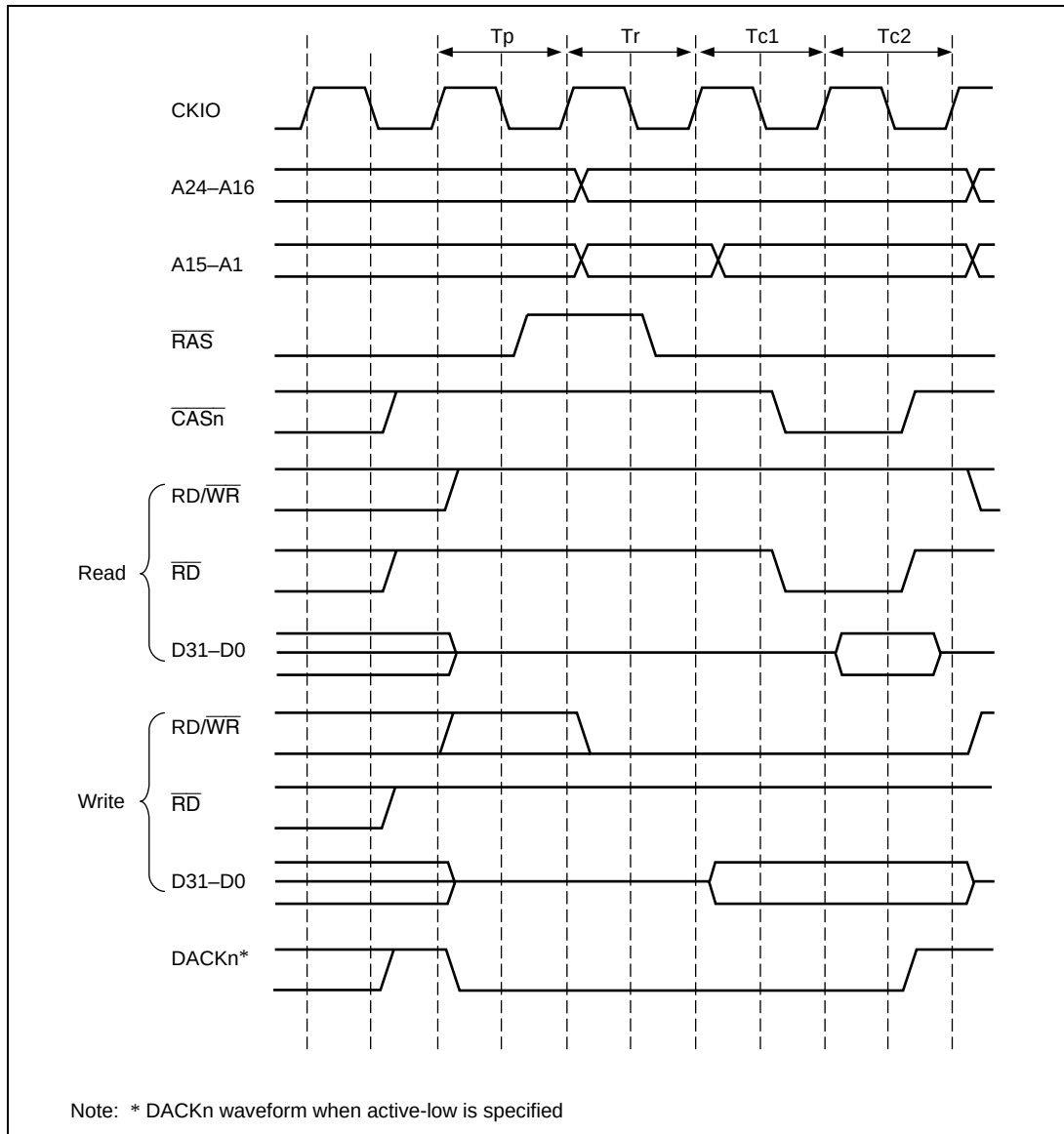
Figure 7.45 \overline{\text{RAS}} Down Mode Different Row Access Timing
