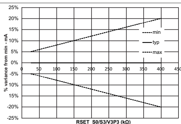
Figure 4. % Variance from Minimum I_{LIM} vs R_{SET}
