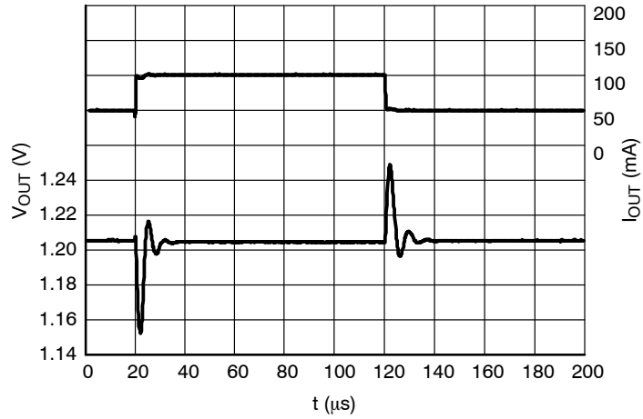
Figure 26. Load Transients, 3.0 V Version, I_{OUT} = 1 - 20 mA, t_R = t_F = 50 \mu s, V_{IN} = 6.0 V
