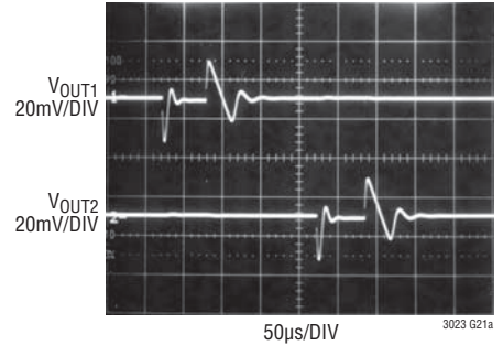
Channel-to-Channel Isolation
