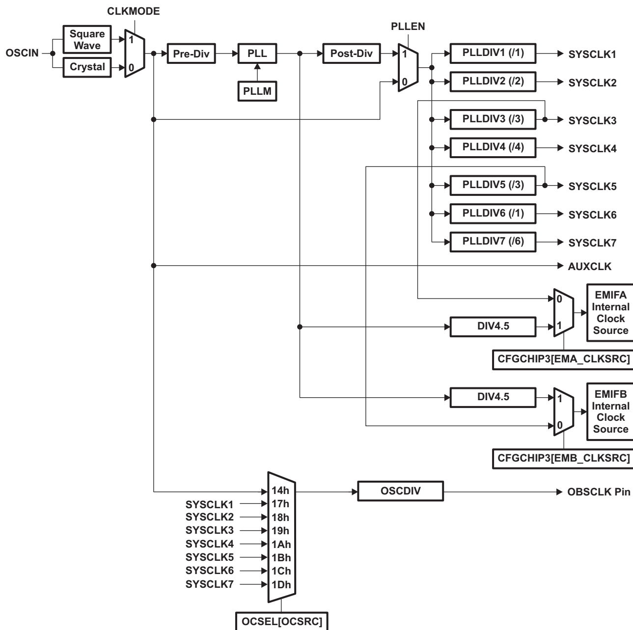
Figure 6-9. PLL Topology
