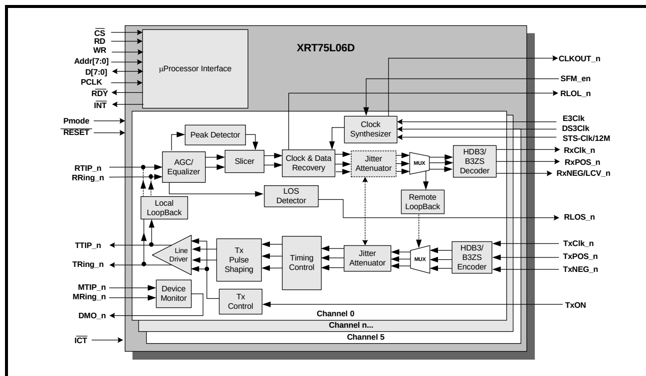
FIGURE 1. BLOCK DIAGRAM OF THE XRT 75L06D
