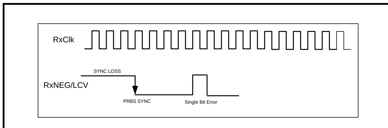
FIGURE 29. PRBS MODE
