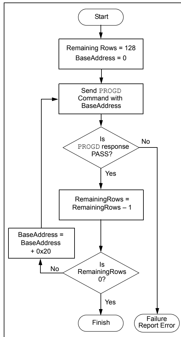
FIGURE 5-4: FLOWCHART FOR PROGRAMMING dsPIC30F6014A DATA EEPROM
