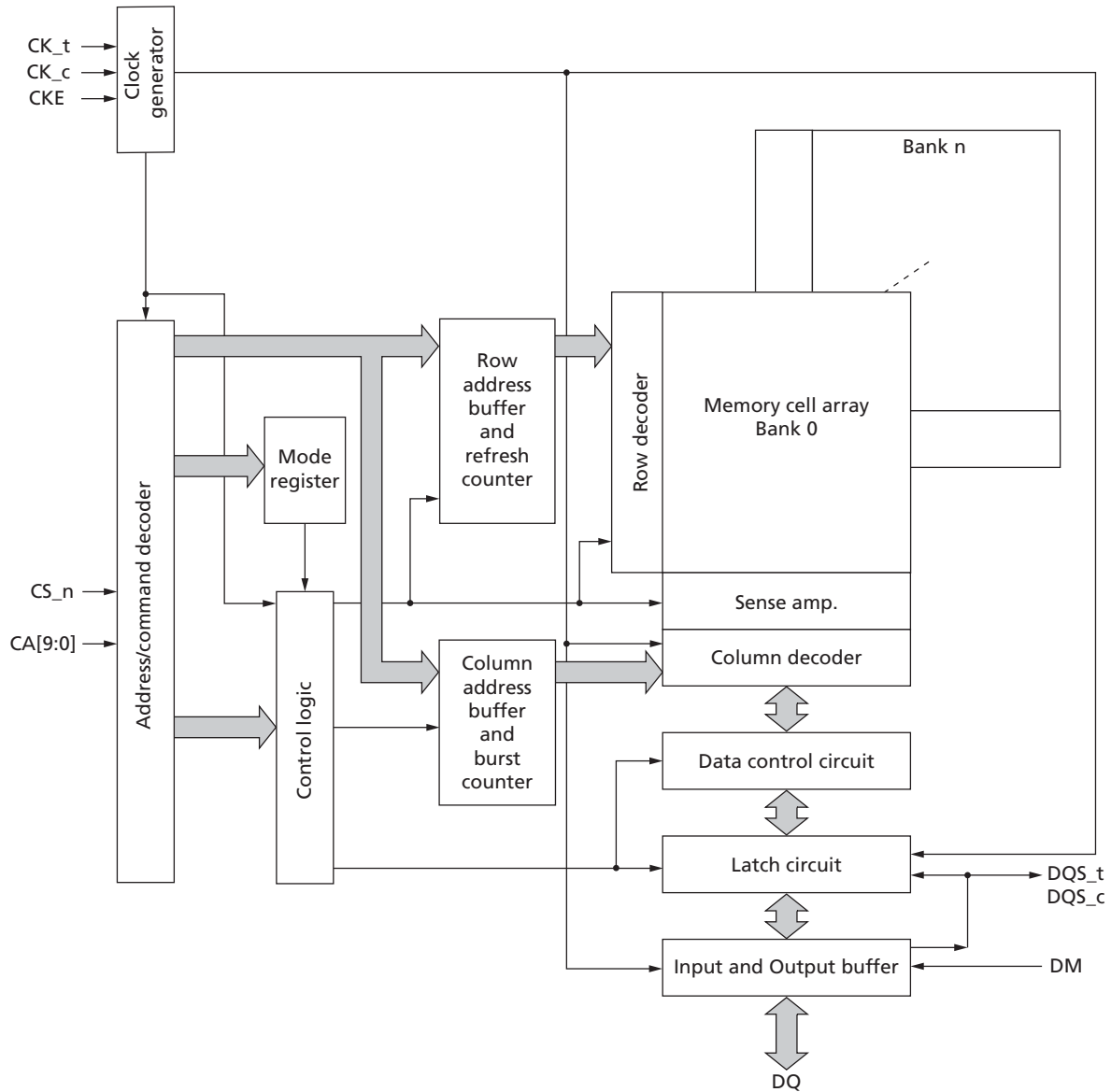
Figure 10: Functional Block Diagram
