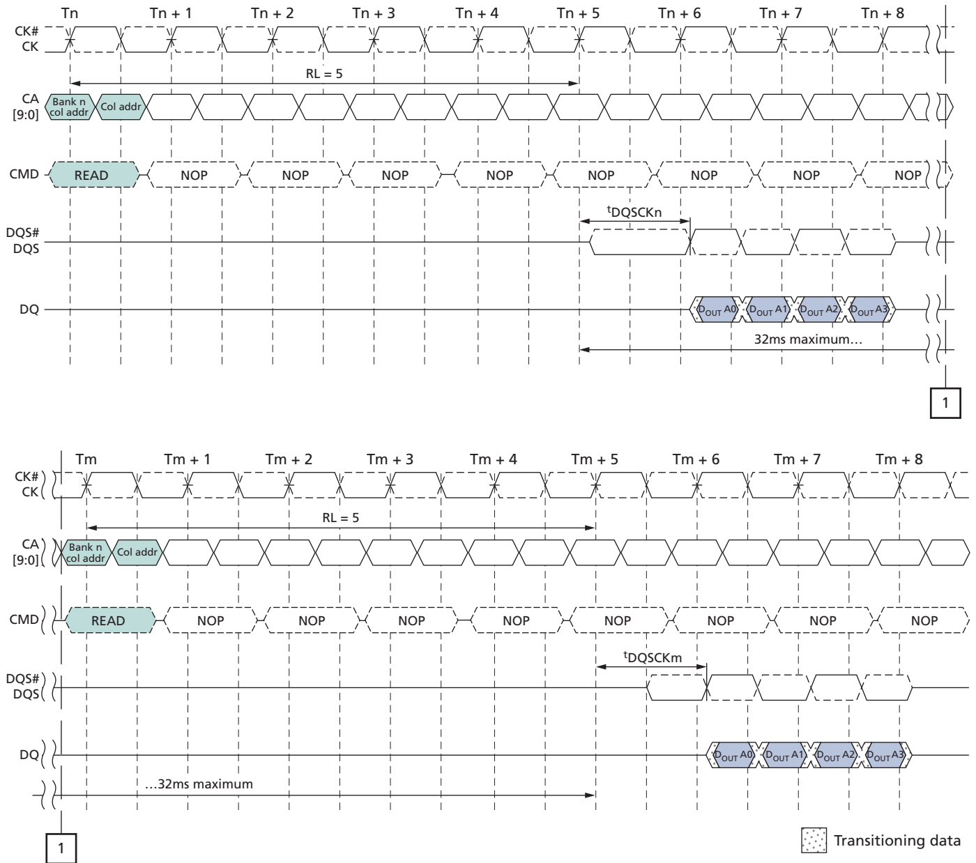
Figure 21: t_{DQSKDL} Timing
