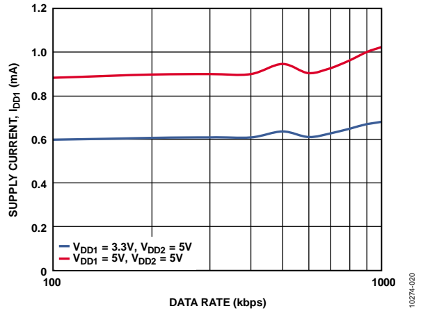
Figure 13. Supply Current ( I_{DD1} ) vs. Data Rate
