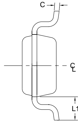
End View
