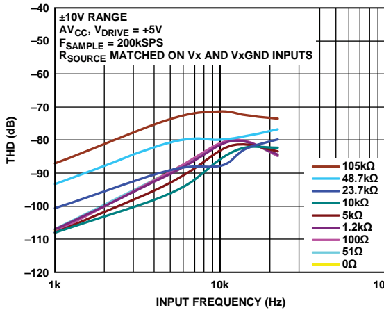
Figure 24. THD vs. Input Frequency for Various Source Impedances, \pm 10 V Range
