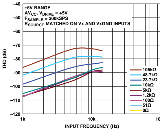
Figure 25. THD vs. Input Frequency for Various Source Impedances, \pm 5 V Range
