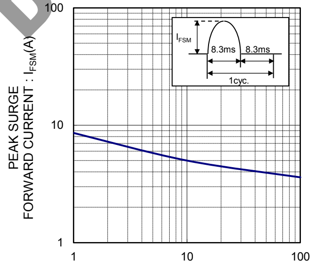
NUMBER OF CYCLES I_{FSM} -CYCLE CHARACTERISTICS
