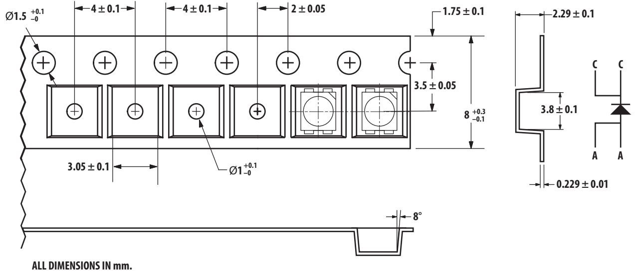
Figure 15. Tape Dimensions
