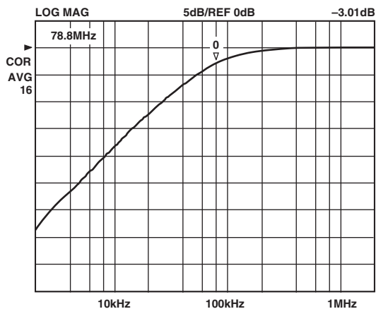
TPC 28. Rx HPF Frequency Response, f_{ADC} = 32 MHz
