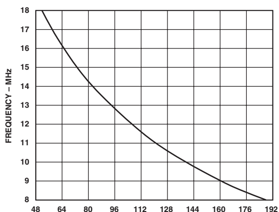
TPC 19. f_C vs. Tuning Target, f_{ADC} = 32 MHz, LPF with Wideband Rx LPF = 0
