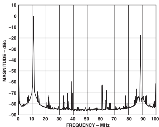
TPC 8. Single-Tone Spectral Plot @ f_{DATA} = 50\text{ MSPS} , f_{OUT} = 11\text{ MHz} , 2\times\text{ LPF}
