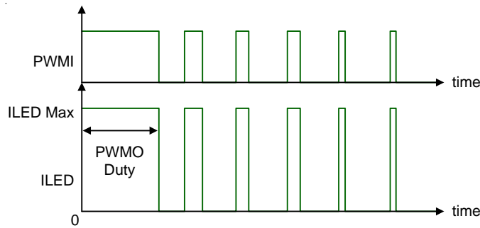
Figure 1. PWM Dimming
