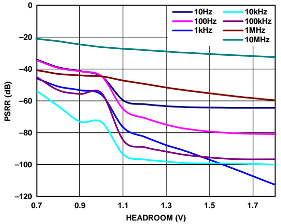
Figure 30. Power Supply Rejection Ratio (PSRR) vs. Headroom Voltage, ADM7151-04, V_{OUT} = 5V , 800 mA Load
