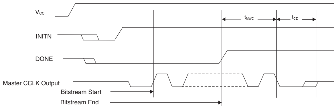
Figure 3-27. Wake-Up Timing
