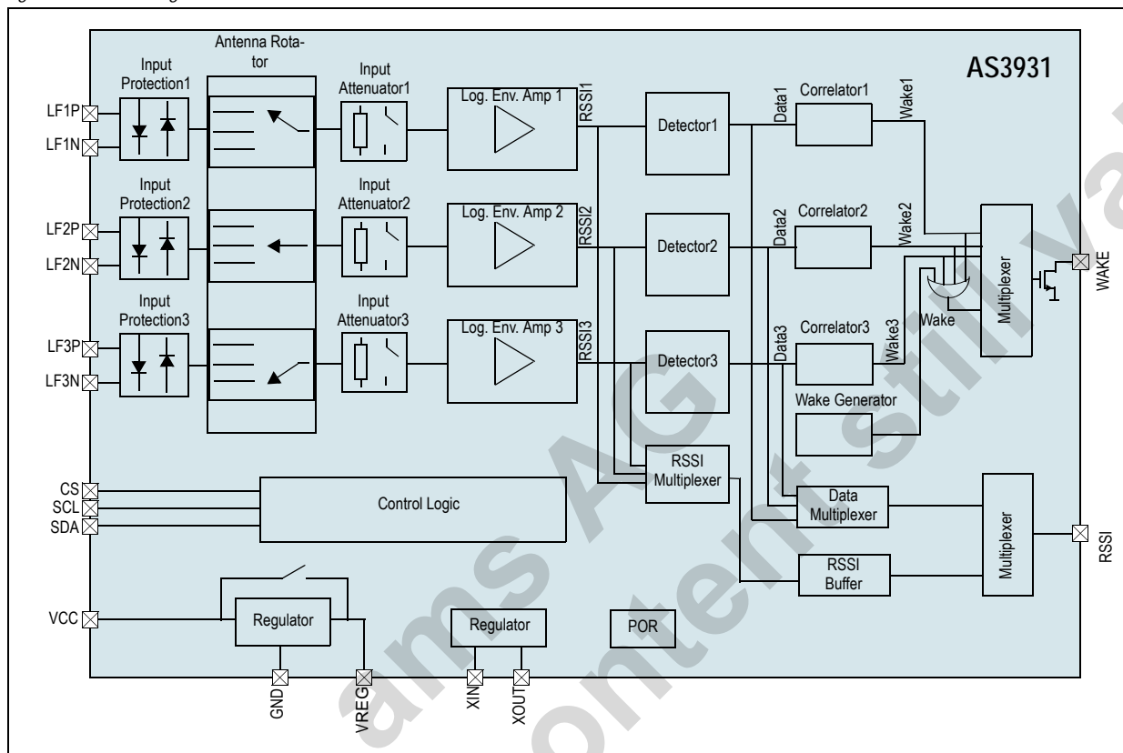
Figure 13. Block Diagram
