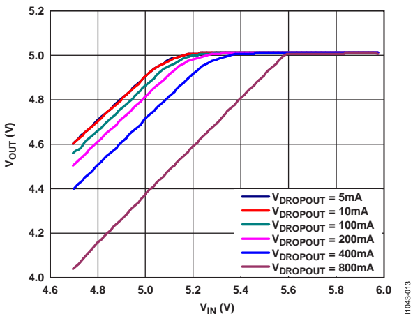
Figure 13. Output Voltage ( V_{OUT} ) vs. Input Voltage ( V_{IN} ) in Dropout, V_{OUT} = 5 V
