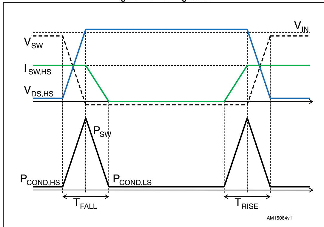
Figure 7. Switching losses
