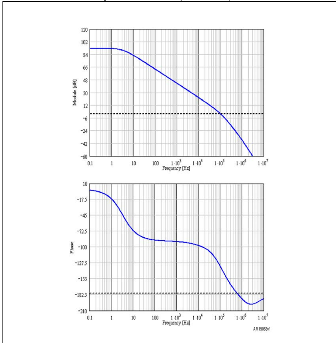
Figure 6. Module and phase bode plot
