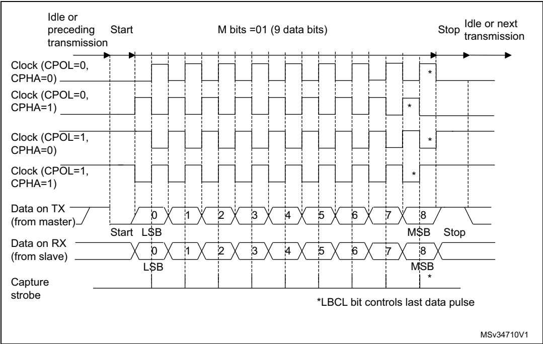
Figure 345. USART data clock timing diagram (M bits = 01)
