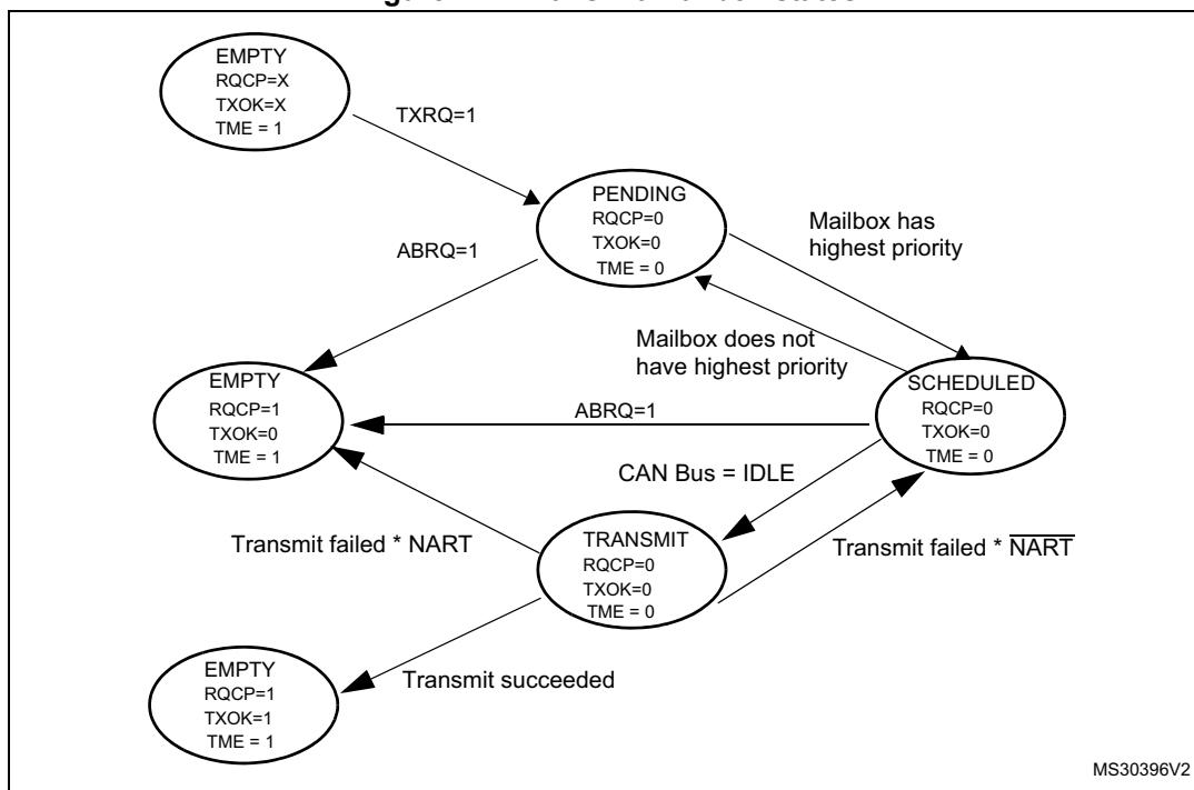
Figure 447. Transmit mailbox states
