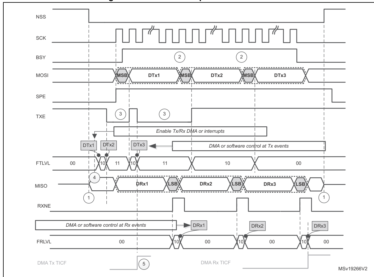
Figure 367. Master full-duplex communication
