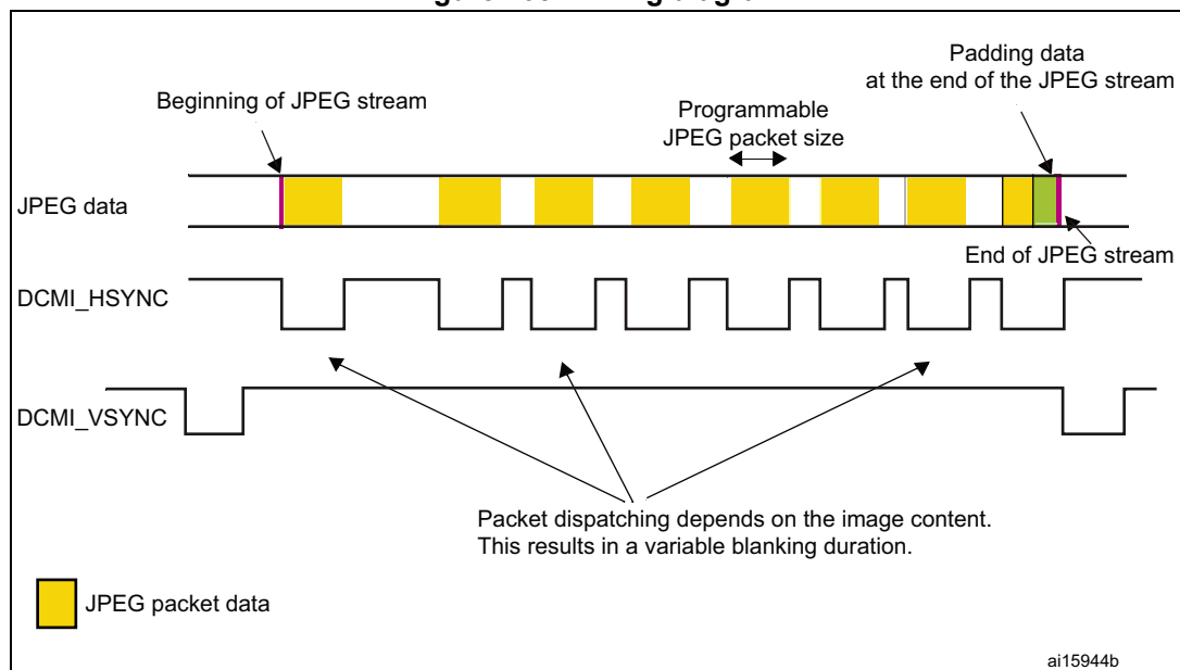
Figure 105. Timing diagram
