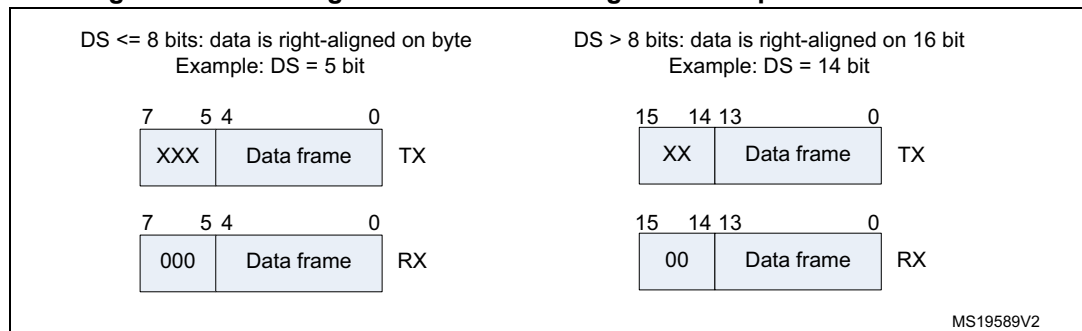
Figure 365. Data alignment when data length is not equal to 8-bit or 16-bit
