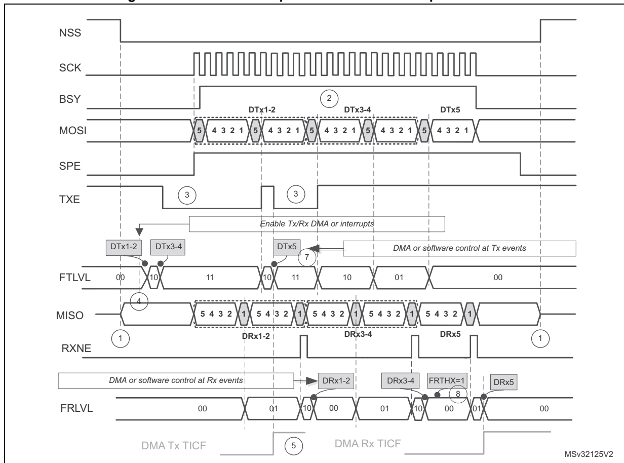
Figure 370. Master full-duplex communication in packed mode
