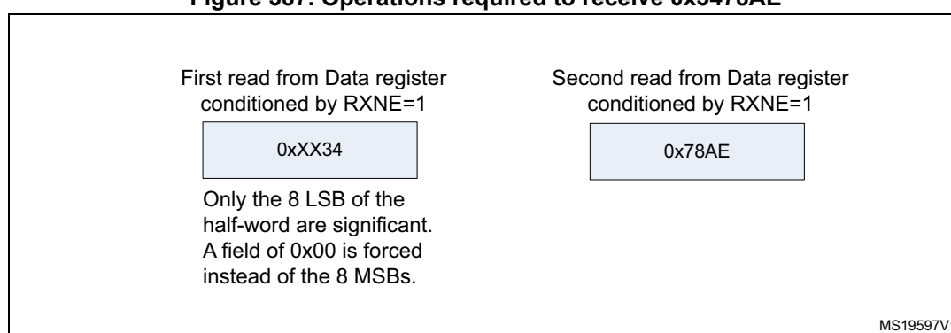
Figure 387. Operations required to receive 0x3478AE
