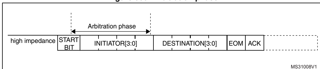
Figure 530. Arbitration phase
