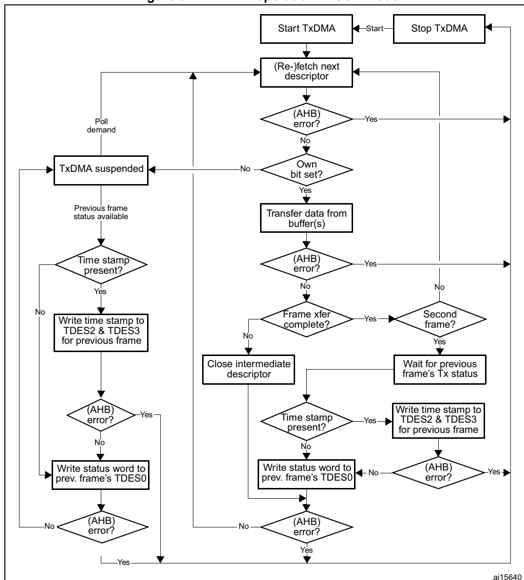
Figure 517. TxDMA operation in OSF mode
