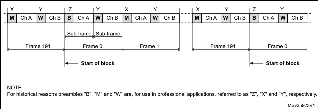
Figure 413. S/PDIF block format
