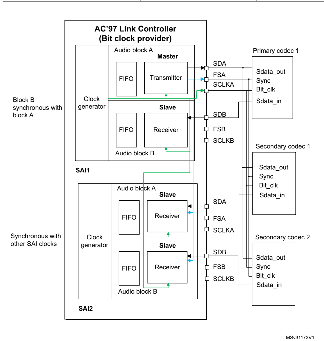
Figure 403. Example of typical AC'97 configuration on devices featuring at least 2 embedded SAI (three external AC'97 decoders)
