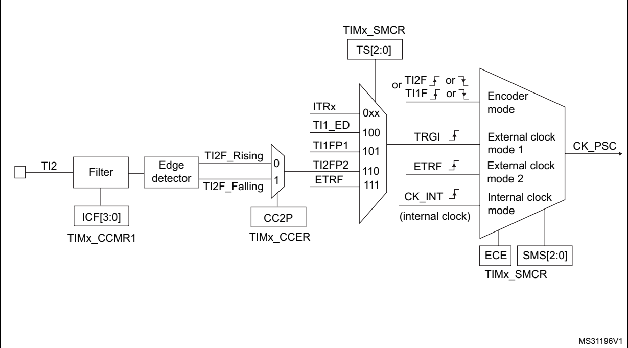
Figure 228. TI2 external clock connection example
