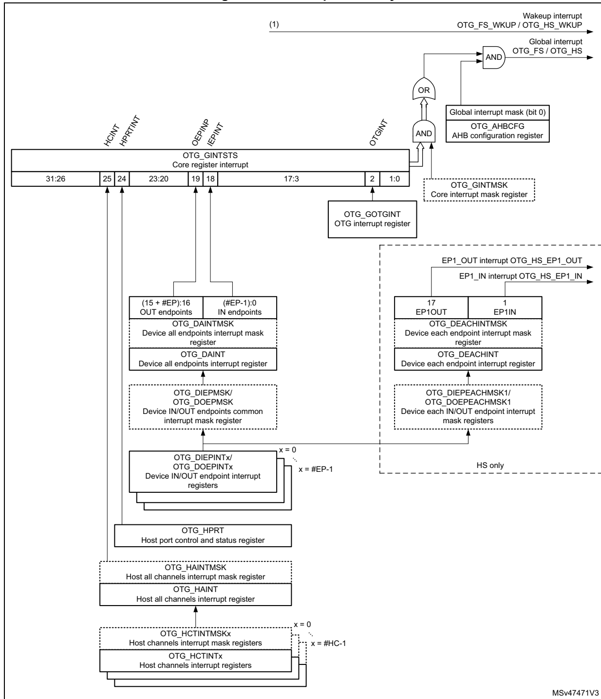
Figure 466. Interrupt hierarchy
