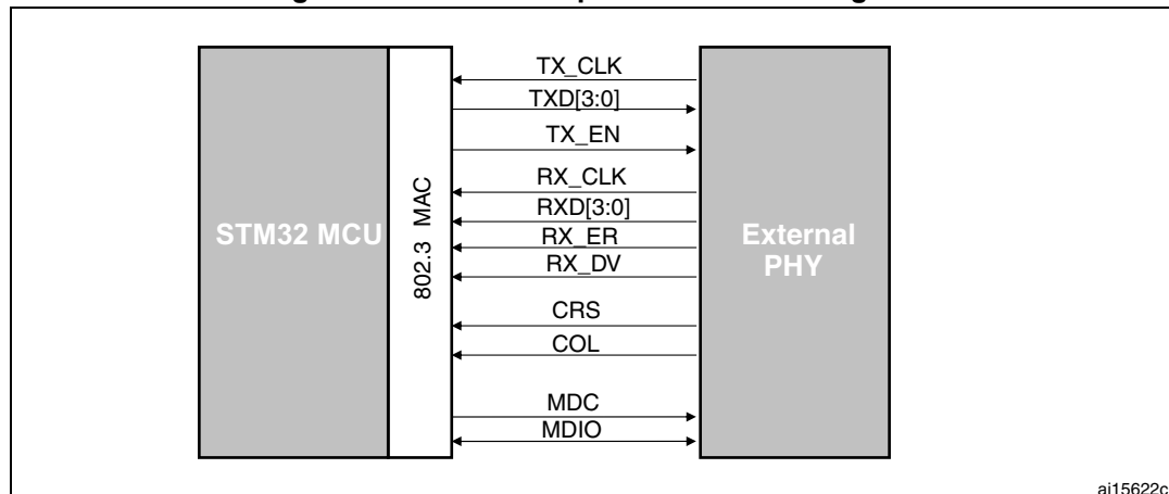
Figure 493. Media independent interface signals
