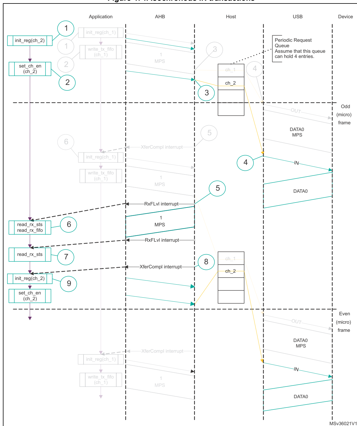
Figure 474. Isochronous IN transactions
