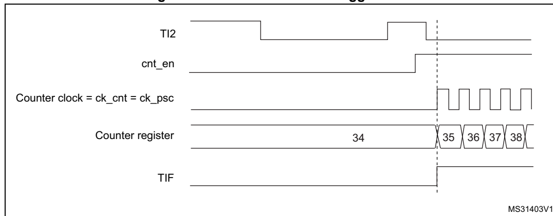
Figure 205. Control circuit in trigger mode
