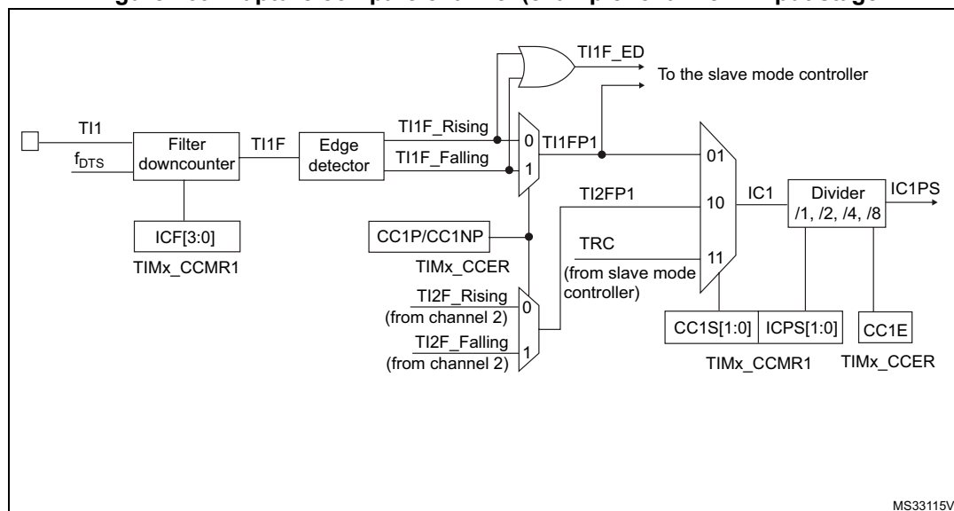
Figure 269. Capture/compare channel (example: channel 1 input stage)
