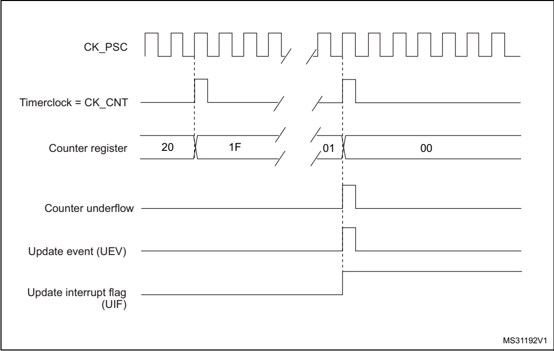
Figure 224. Counter timing diagram, internal clock divided by N
