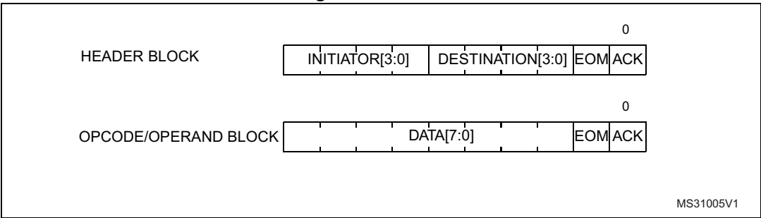
Figure 527. Blocks
