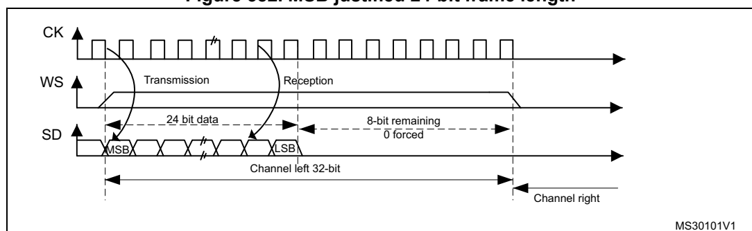
Figure 382. MSB justified 24-bit frame length
