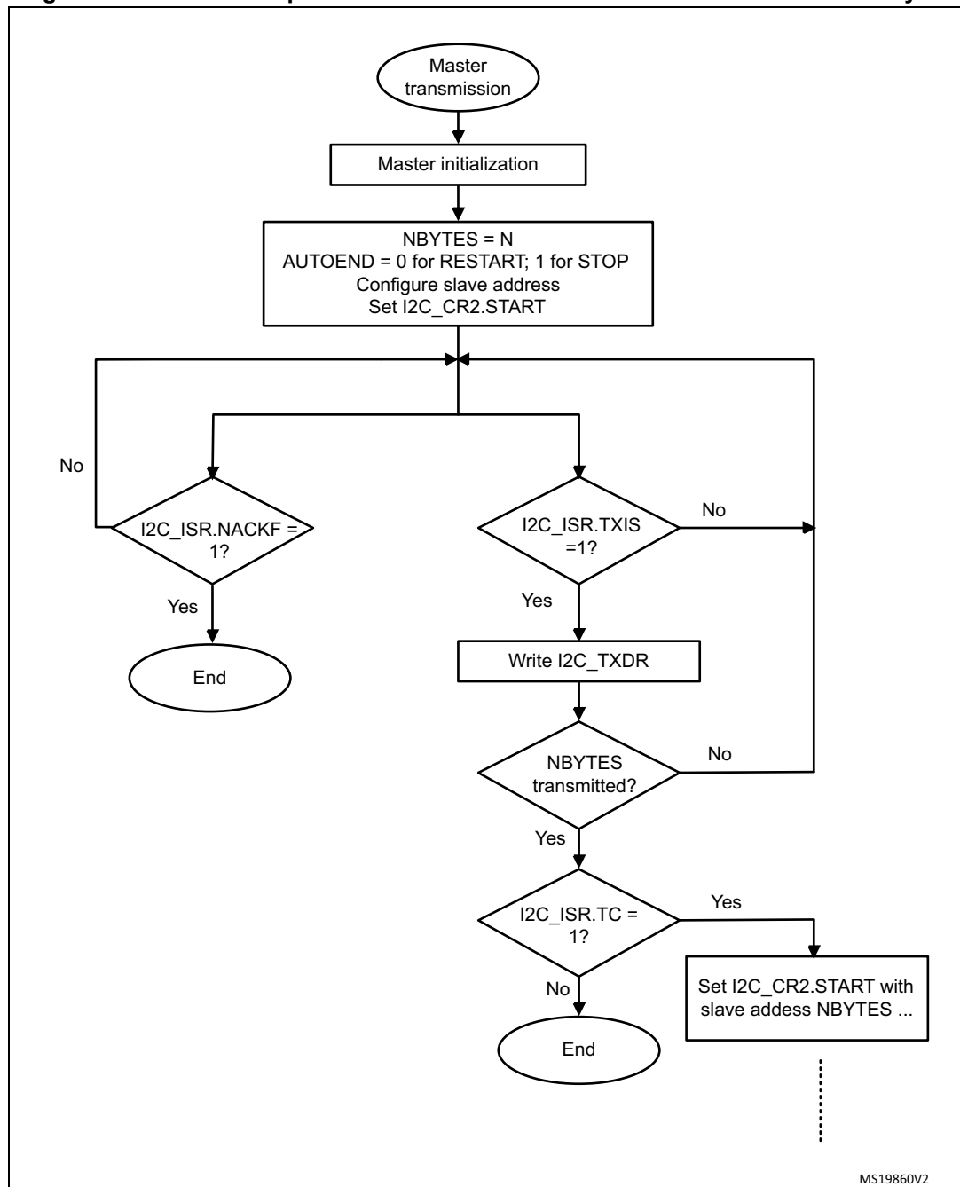
Figure 319. Transfer sequence flowchart for I2C master transmitter for N \leq 255 bytes
