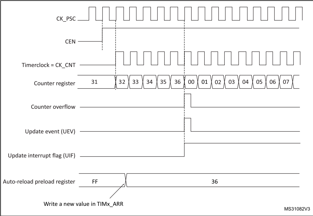
Figure 156. Counter timing diagram, update event when ARPE=0 (TIMx_ARR not preloaded)
