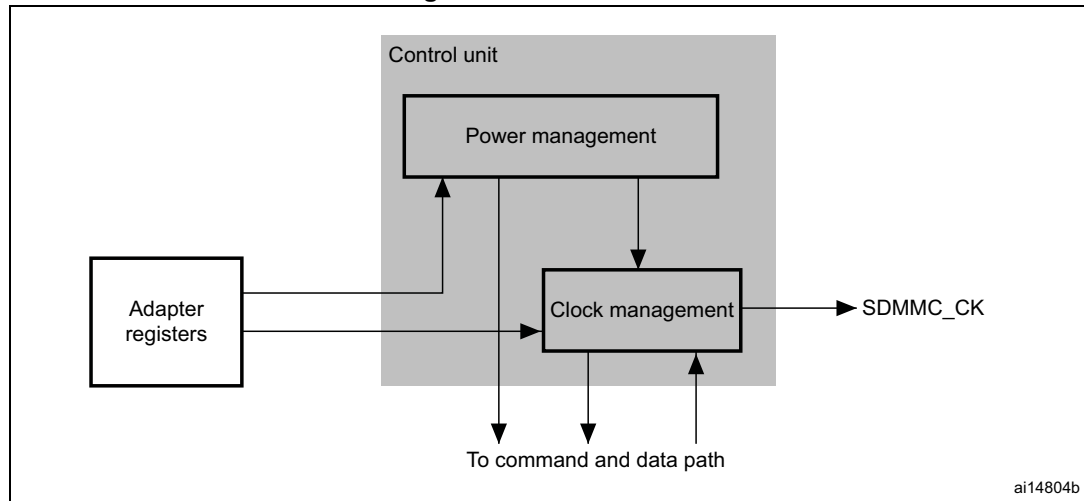
Figure 434. Control unit
