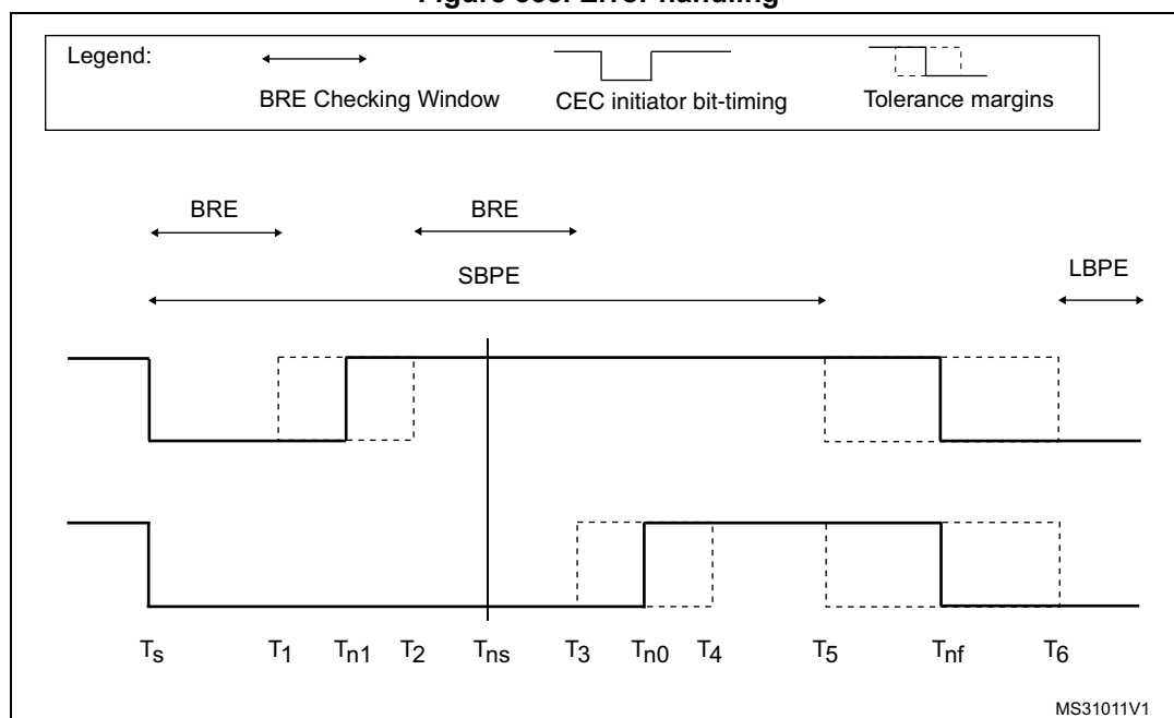
Figure 533. Error handling
