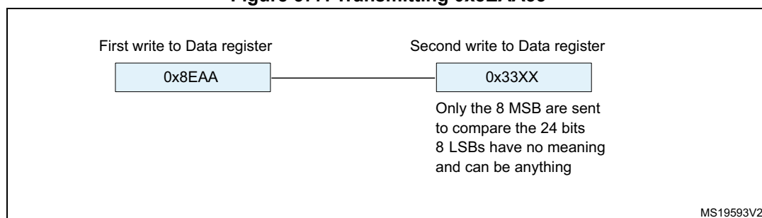
Figure 377. Transmitting 0x8EAA33
