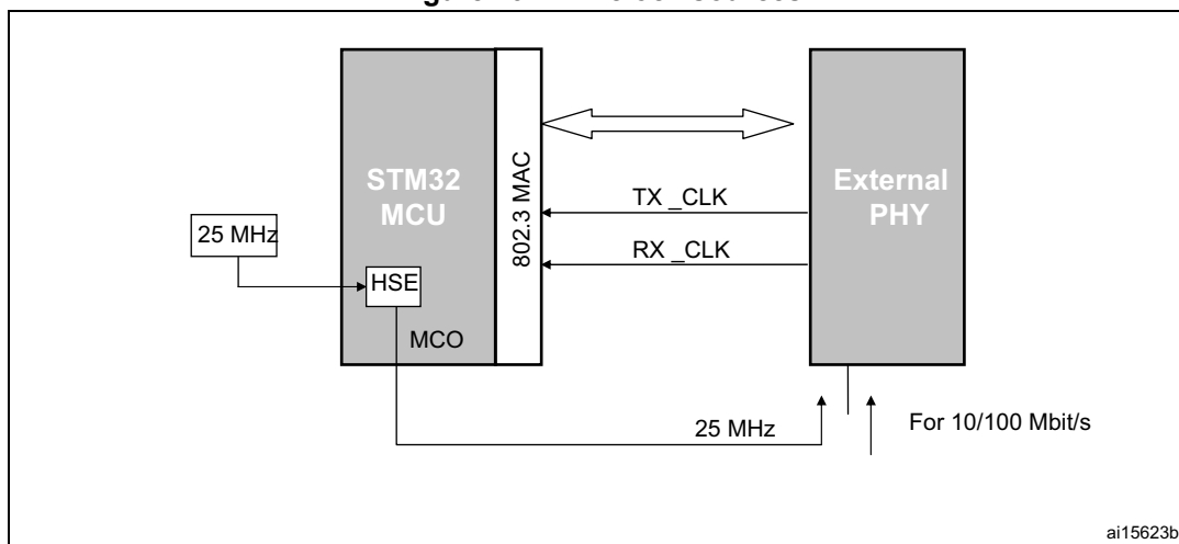
Figure 494. MII clock sources
