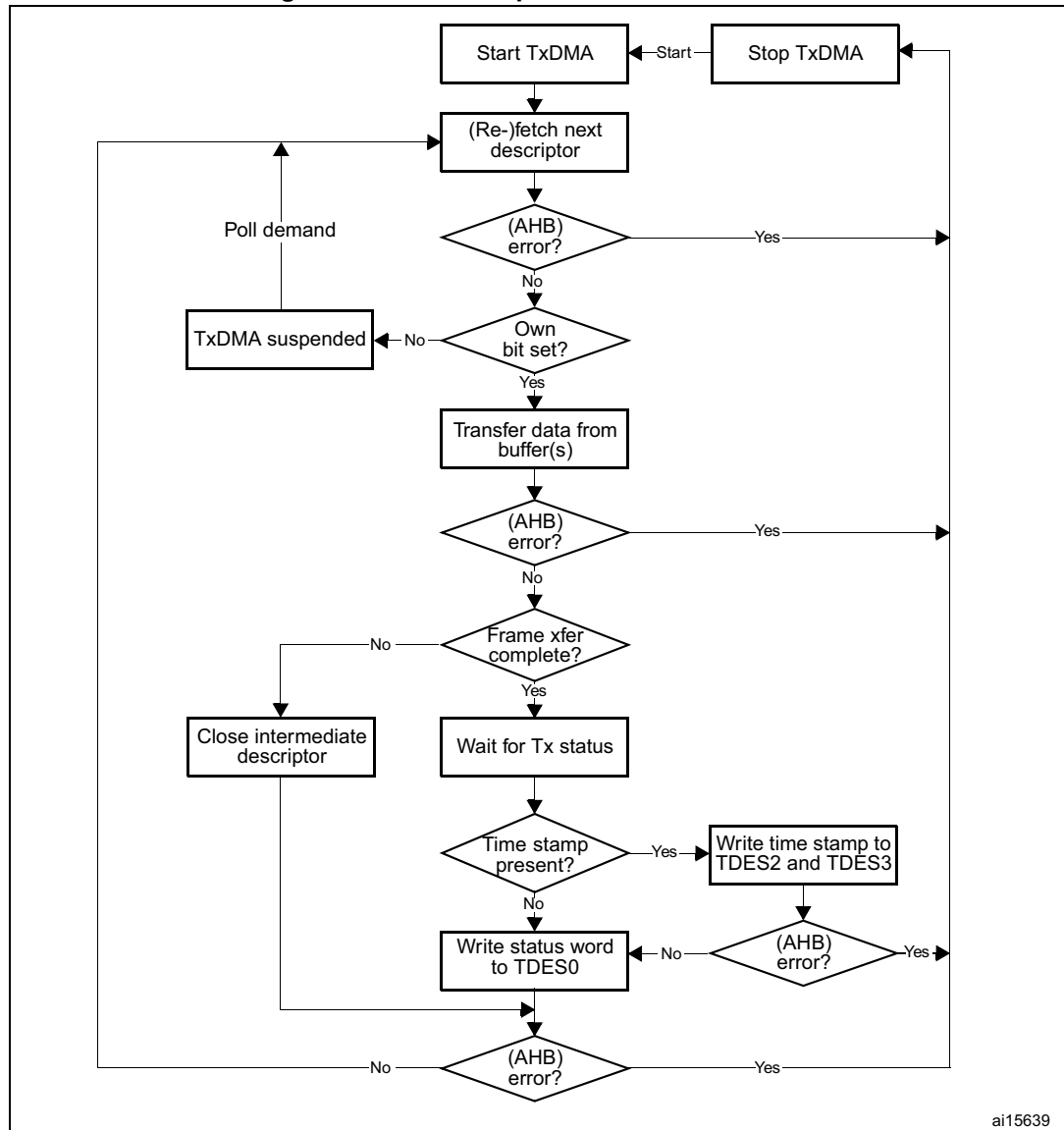
Figure 516. TxDMA operation in default mode
