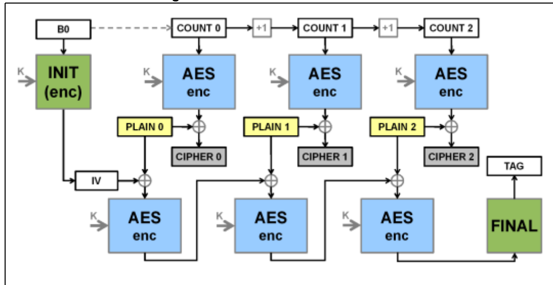
Figure 124. AES-CCM mode overview
