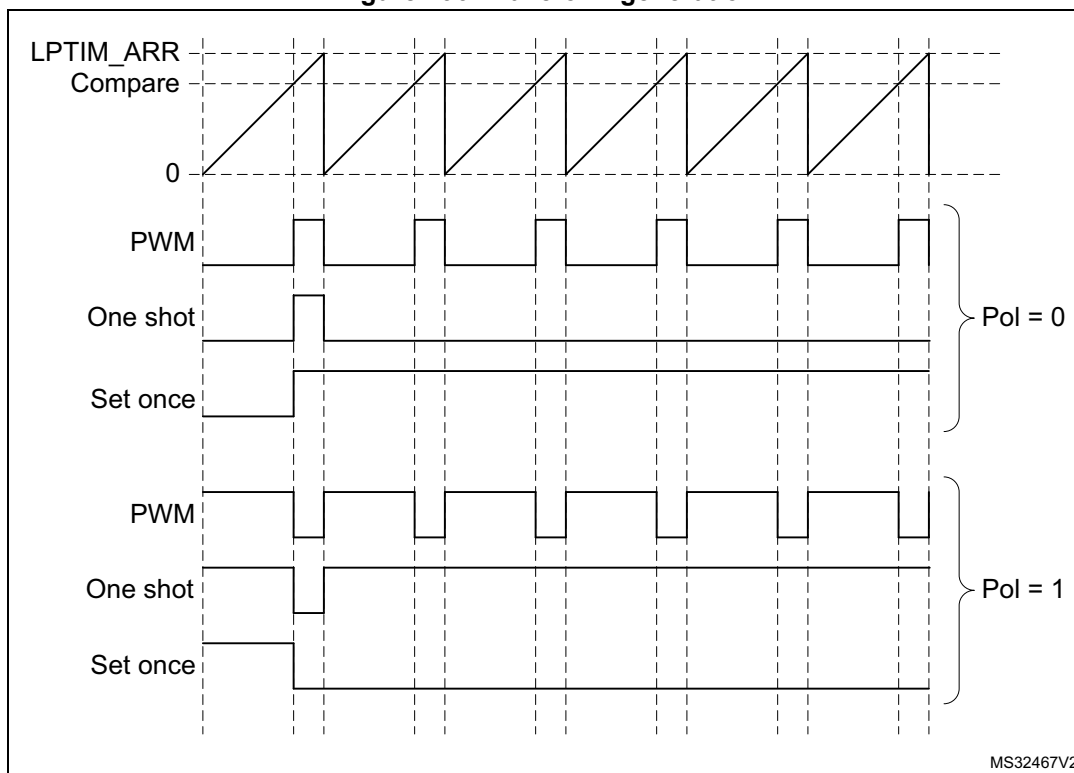
Figure 296. Waveform generation
