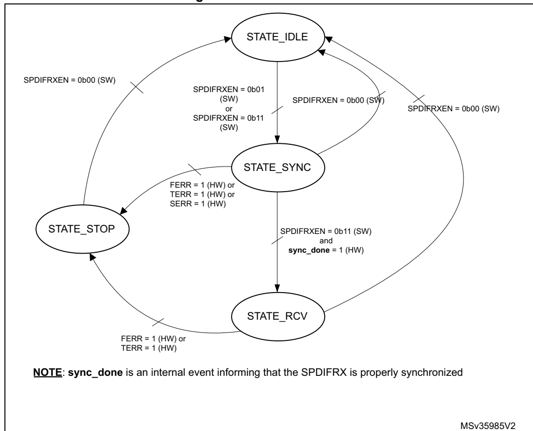
Figure 421. SPDIFRX States
