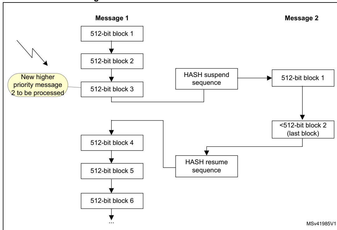
Figure 147. HASH save/restore mechanism
