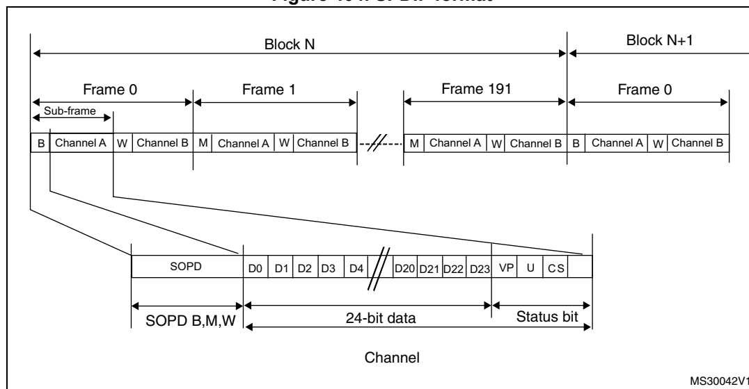
Figure 404. SPDIF format
