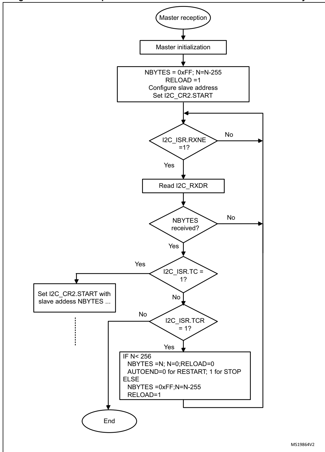
Figure 323. Transfer sequence flowchart for I2C master receiver for N &gt; 255 bytes
