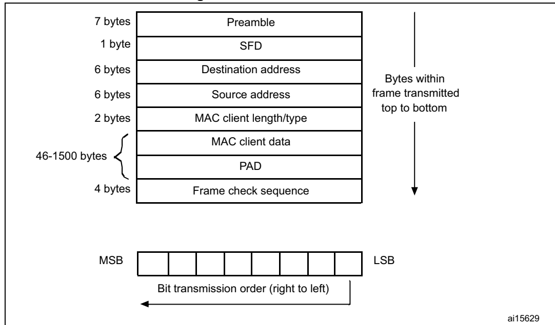
Figure 499. MAC frame format
