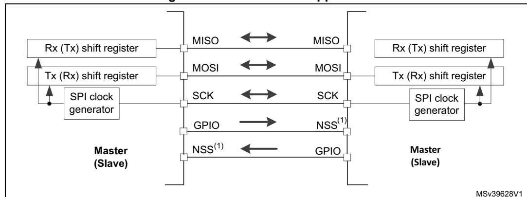
Figure 362. Multi-master application
