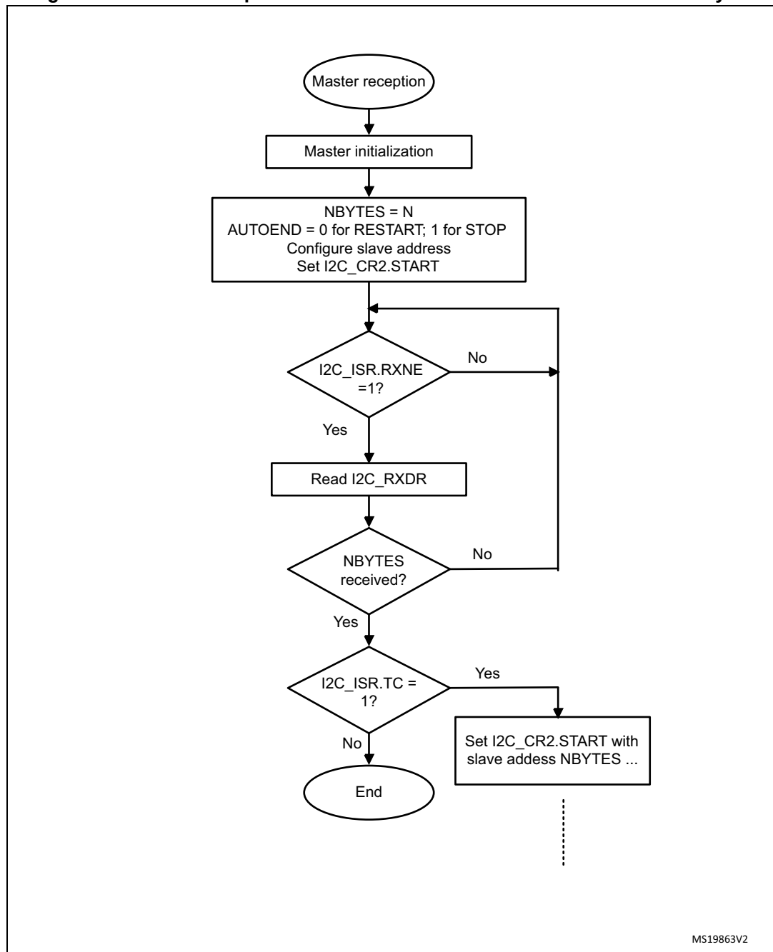
Figure 322. Transfer sequence flowchart for I2C master receiver for N \leq 255 bytes
