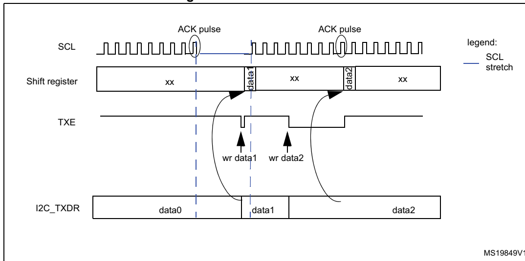
Figure 307. Data transmission
