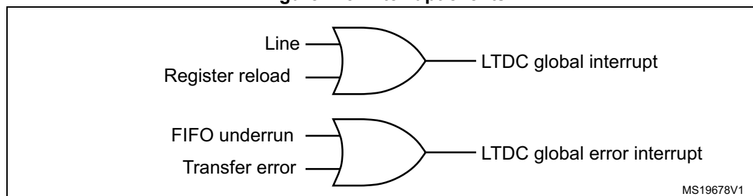
Figure 115. Interrupt events
