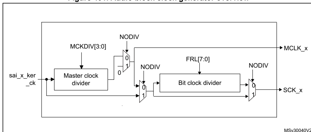
Figure 401. Audio block clock generator overview
