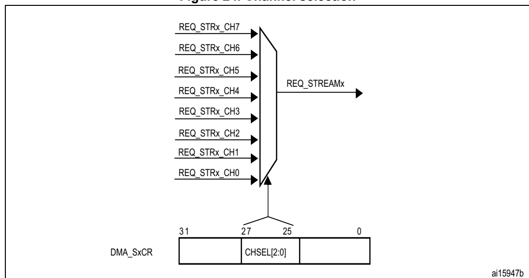
Figure 24. Channel selection
