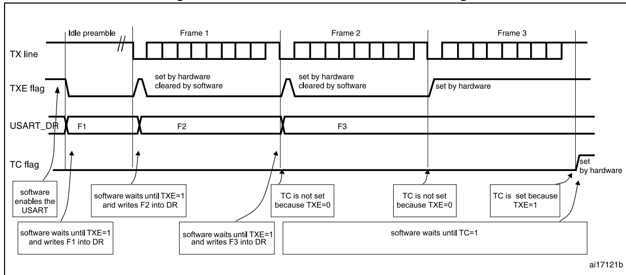
Figure 335. TC/TXE behavior when transmitting
