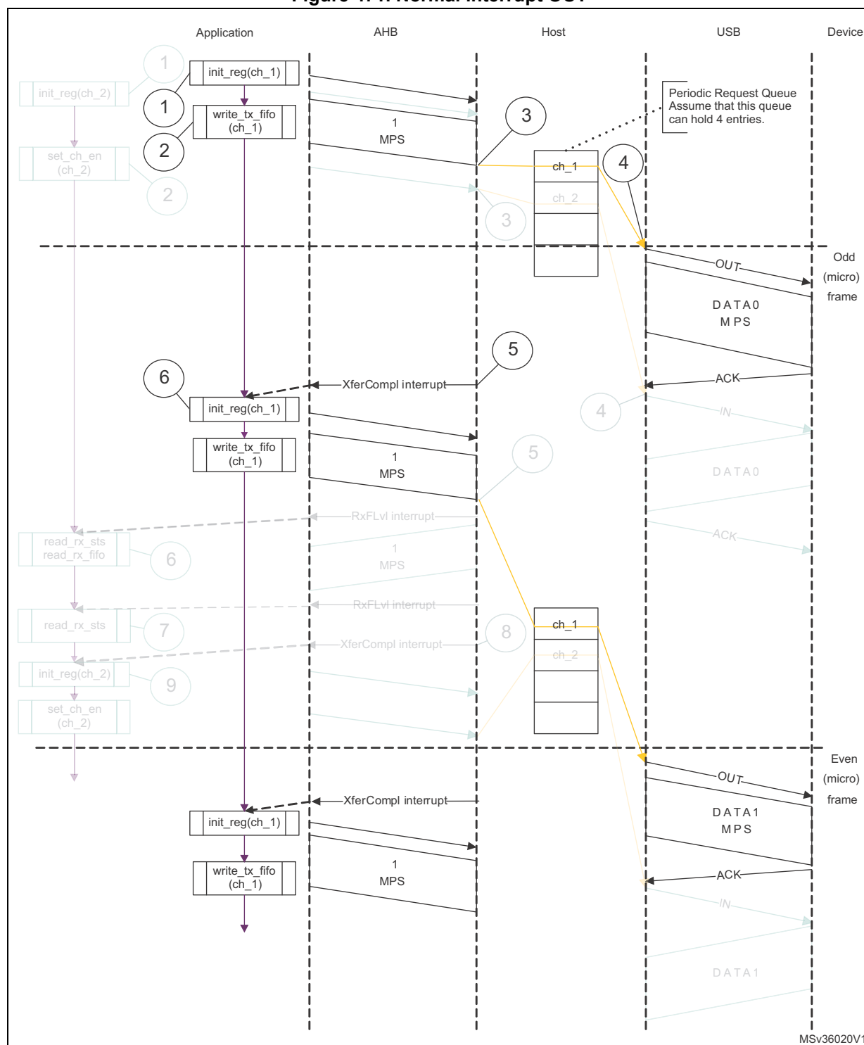
Figure 471. Normal interrupt OUT
