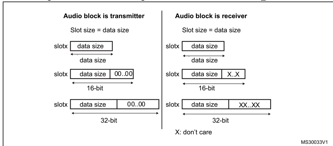
Figure 399. Slot size configuration with FBOFF = 0 in SAI_xSLOTR
