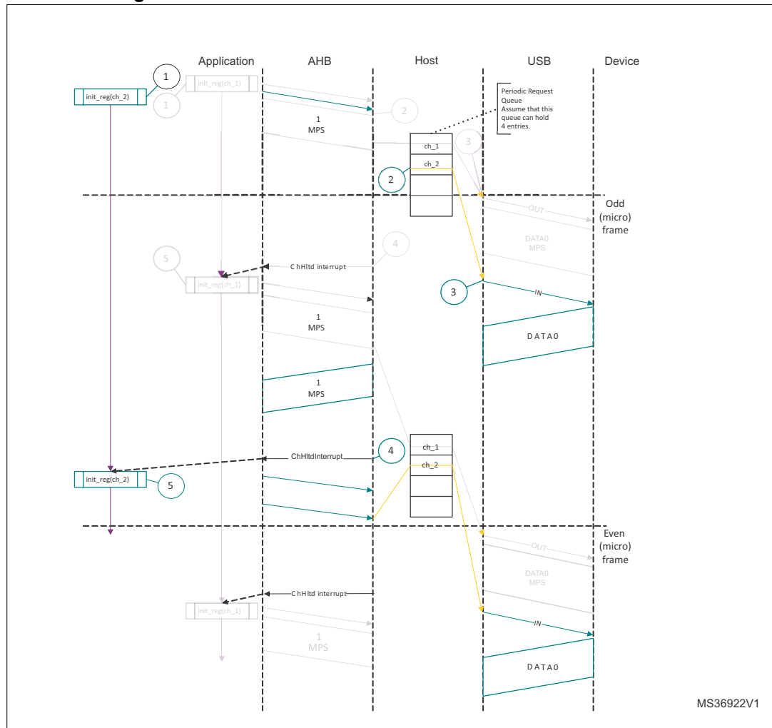
Figure 480. Normal isochronous IN transactions - DMA mode
