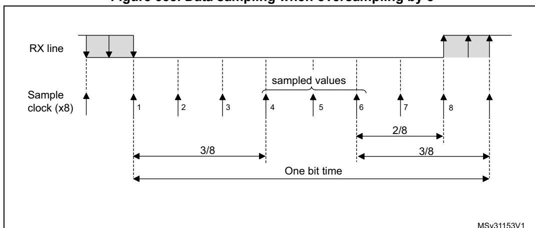
Figure 338. Data sampling when oversampling by 8
