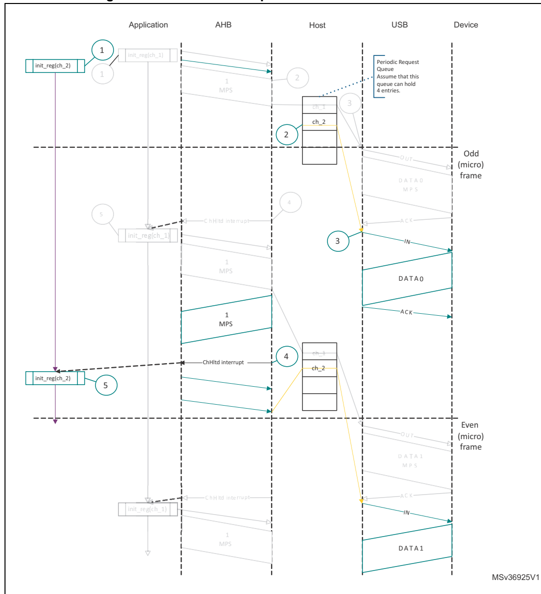
Figure 478. Normal interrupt IN transactions - DMA mode
