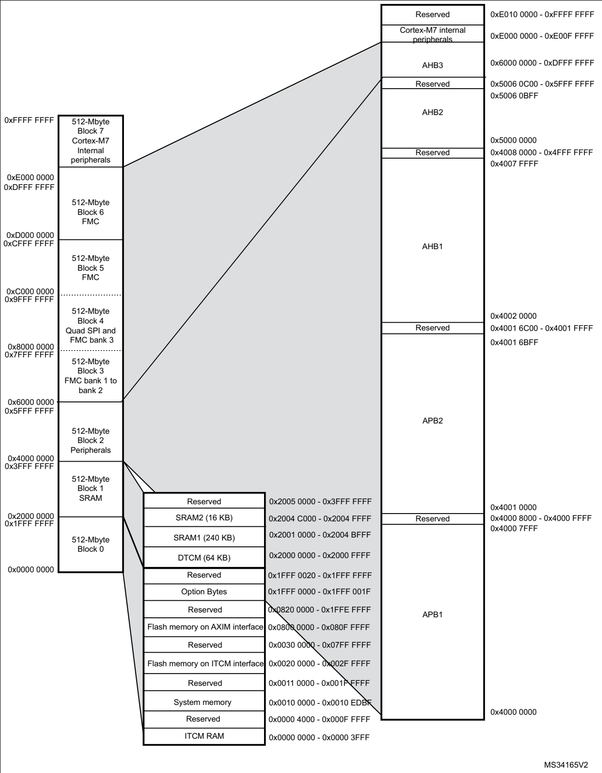
Figure 2. Memory map
