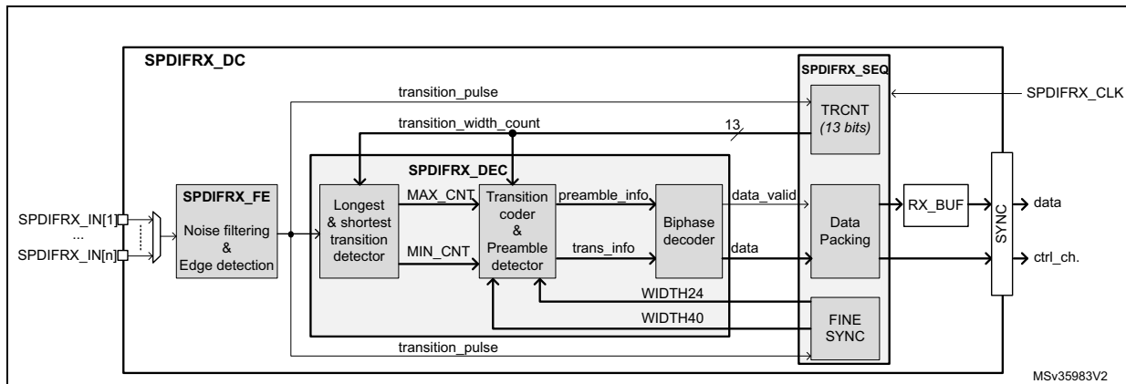
Figure 416. SPDIFRX decoder
