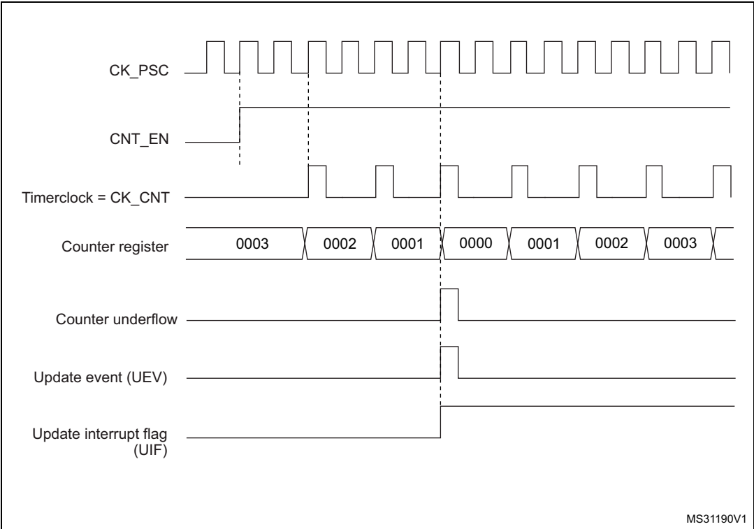
Figure 222. Counter timing diagram, internal clock divided by 2
