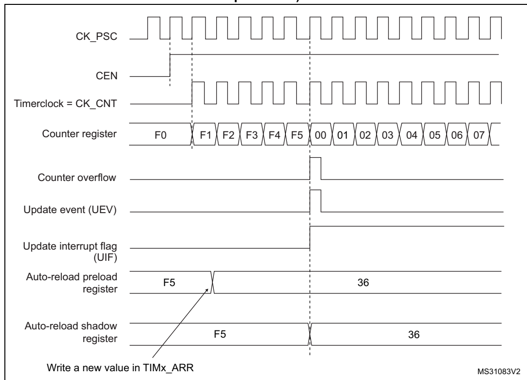
Figure 215. Counter timing diagram, Update event when ARPE=1 (TIMx_ARR preloaded)
