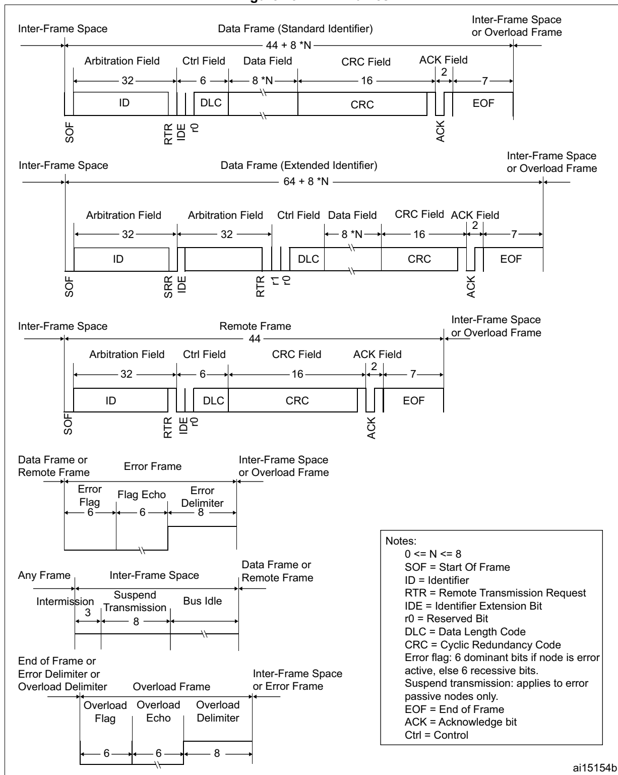
Figure 454. CAN frames
