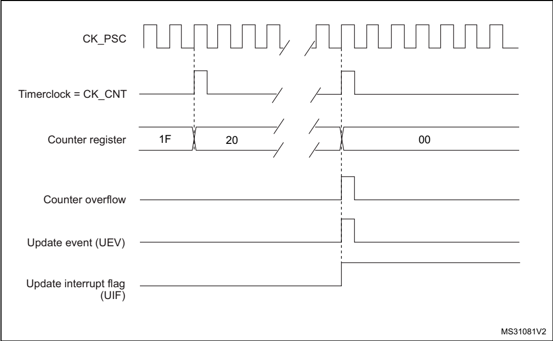
Figure 263. Counter timing diagram, internal clock divided by N
