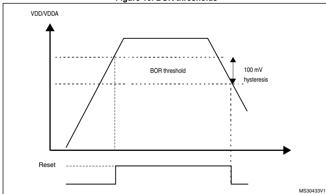
Figure 10. BOR thresholds
