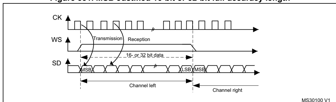
Figure 381. MSB Justified 16-bit or 32-bit full-accuracy length
