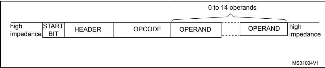
Figure 526. Message structure
