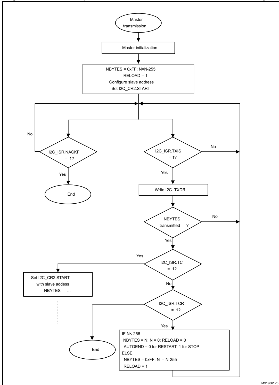
Figure 320. Transfer sequence flowchart for I2C master transmitter for N&gt;255 bytes
