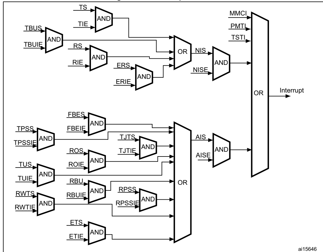
Figure 523. Interrupt scheme
