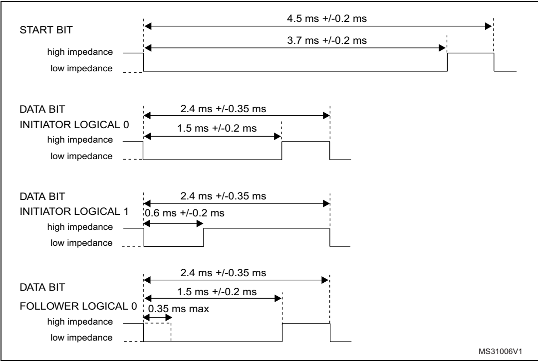
Figure 528. Bit timings
