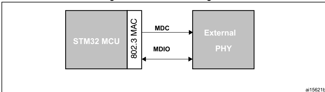
Figure 490. SMI interface signals
