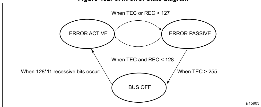
Figure 452. CAN error state diagram
