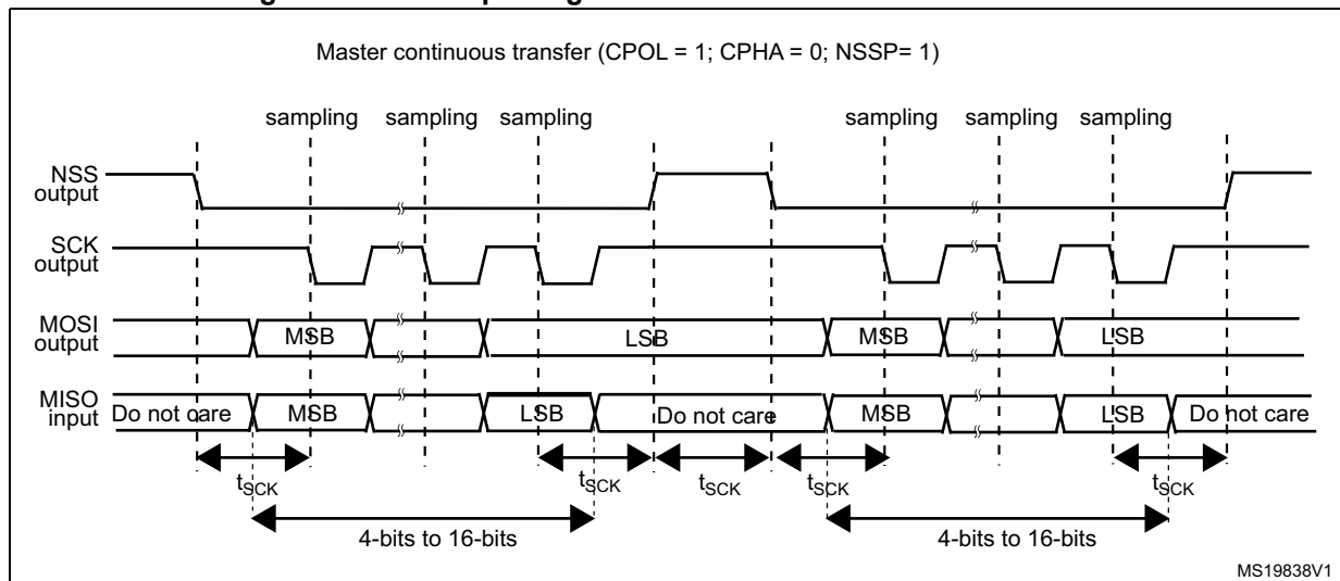
Figure 371. NSSP pulse generation in Motorola SPI master mode
