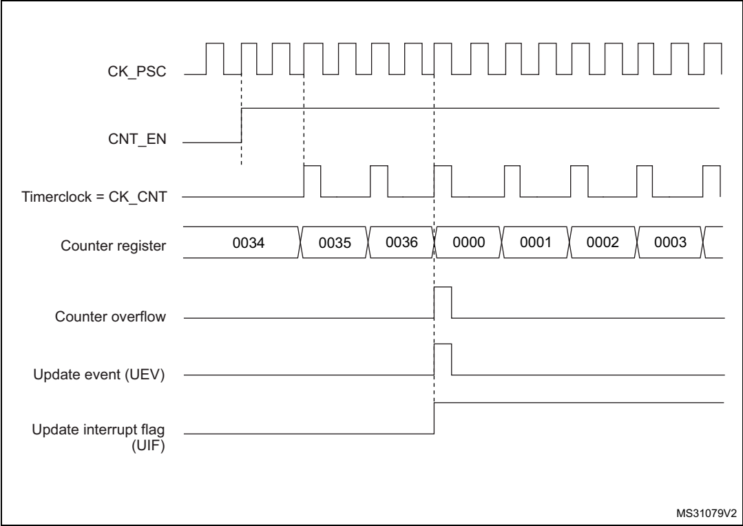
Figure 211. Counter timing diagram, internal clock divided by 2
