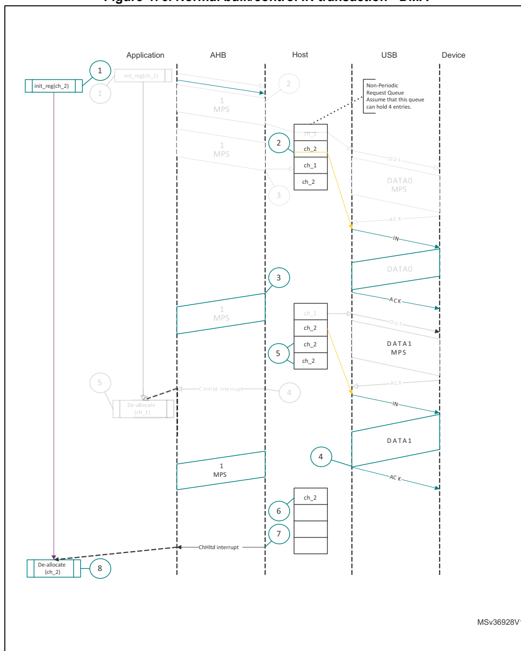
Figure 476. Normal bulk/control IN transaction - DMA
