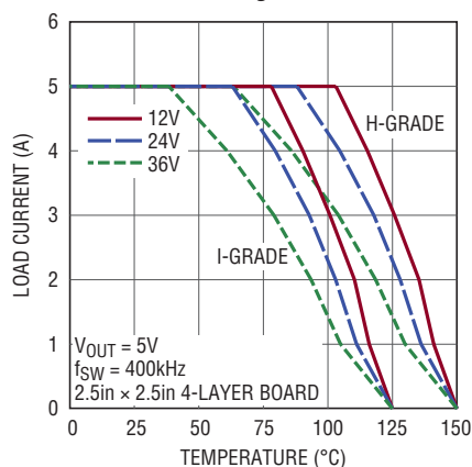
Thermal Derating
