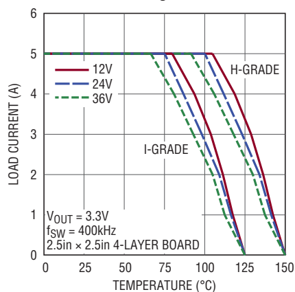
Thermal Derating
