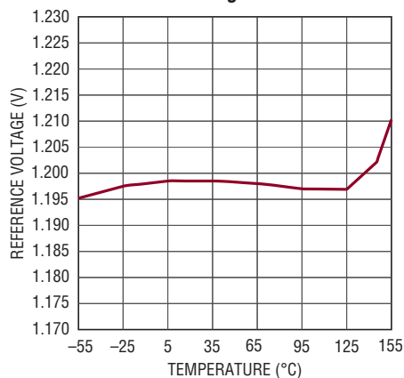
Reference Voltage
