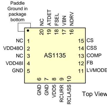
Figure 2 - Pin-out Diagram
