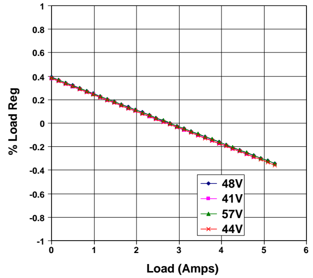
Figure 22 - 5V 30W Load Regulation
