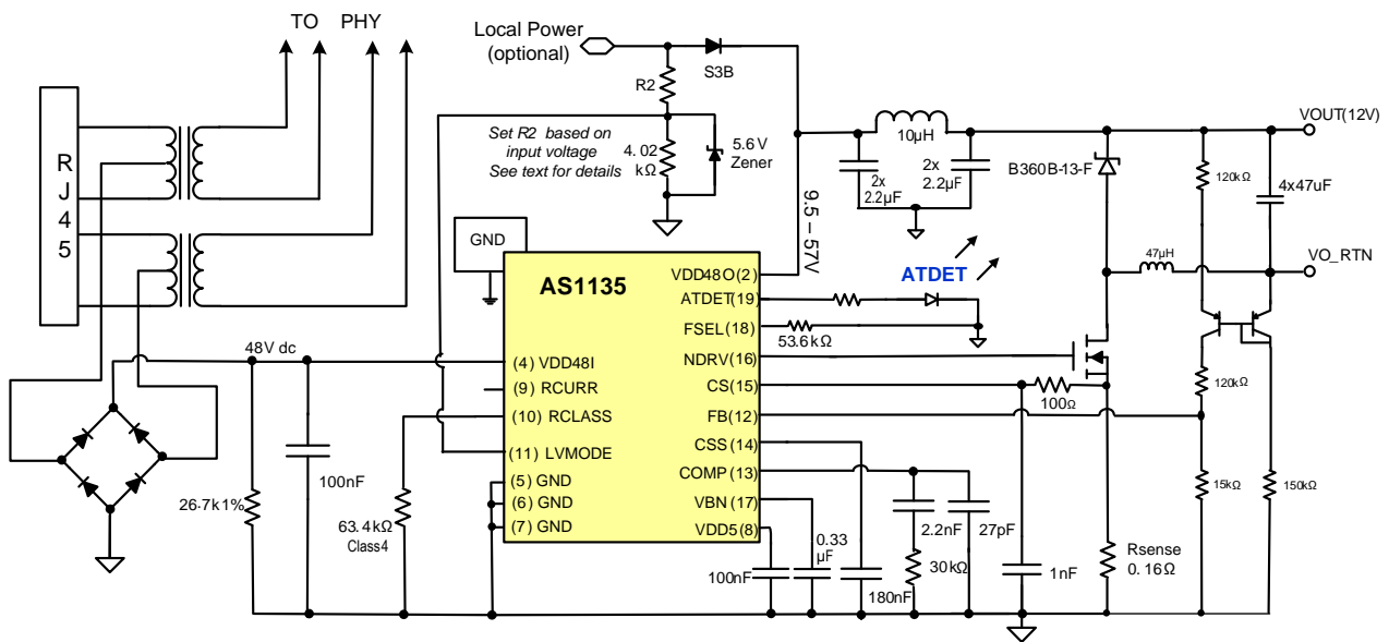
Figure 34 - PoE PD Controller with Non-Isolated BUCK DC-DC converter
