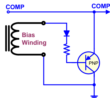
Figure 31 - Short-Circuit Protection
