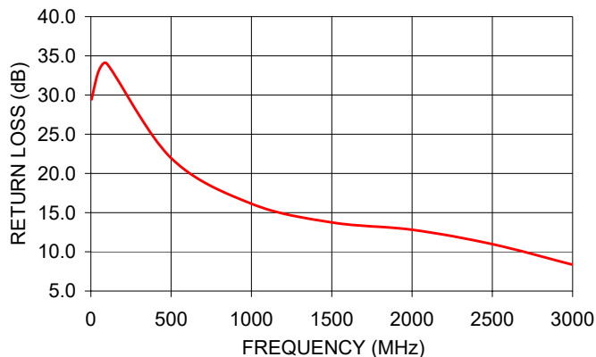
TC1-1-13M-75+ INPUT RETURN LOSS
