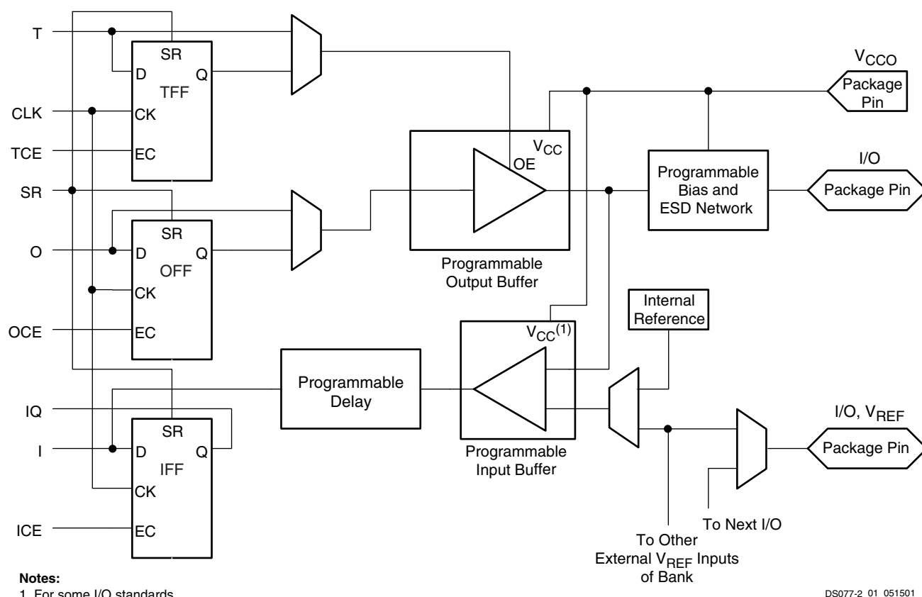
Figure 4: Spartan-II® Input/Output Block (IOB)
