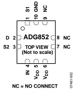
Figure 2. Pin Configurations
