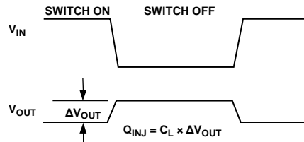
Figure 21. Charge Injection
